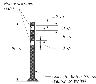
TUBULAR DELINEATOR Not to Scale
