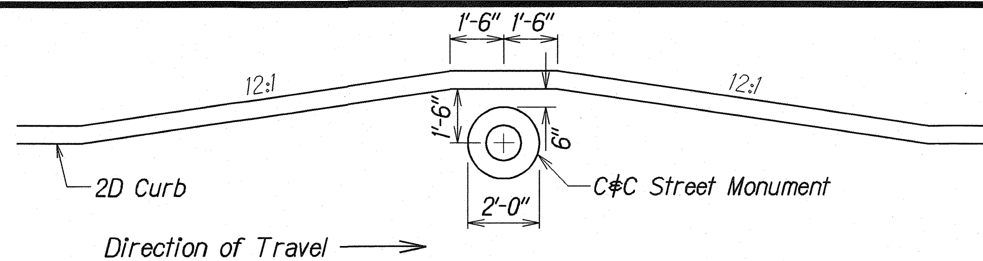
CURB ADJUSTMENT AT C&C STREET MONUMENT Not To Scale
