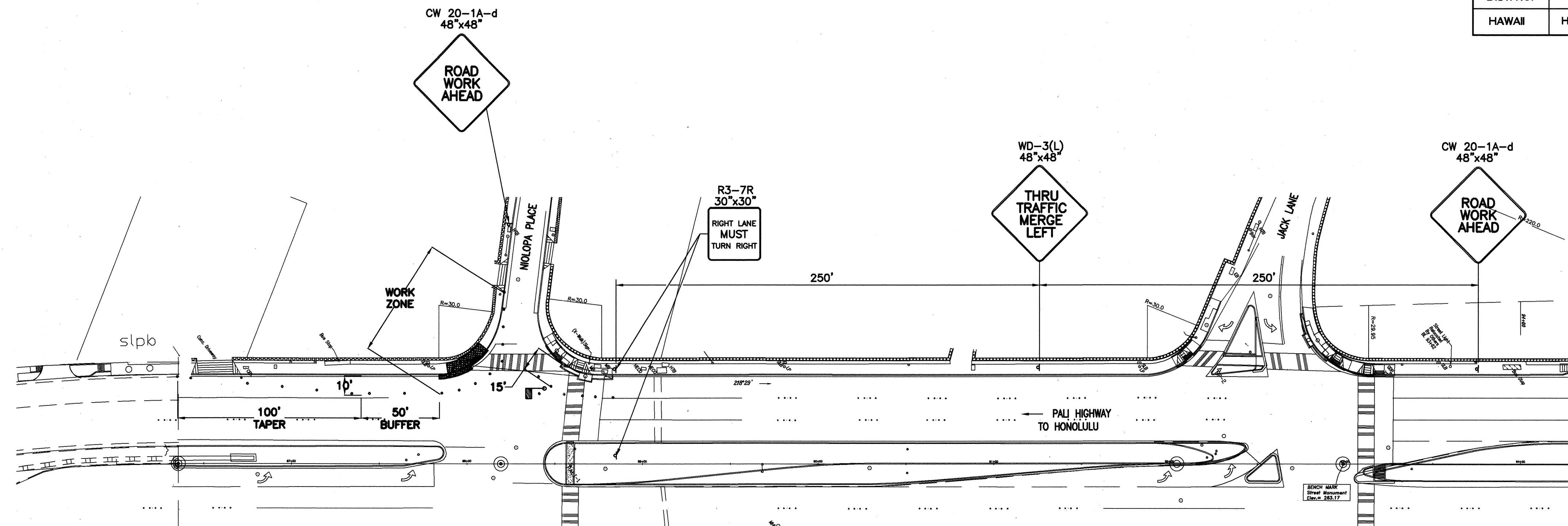
PHASE VIII TRAFFIC CONTROL SCALE: 1"=40'
