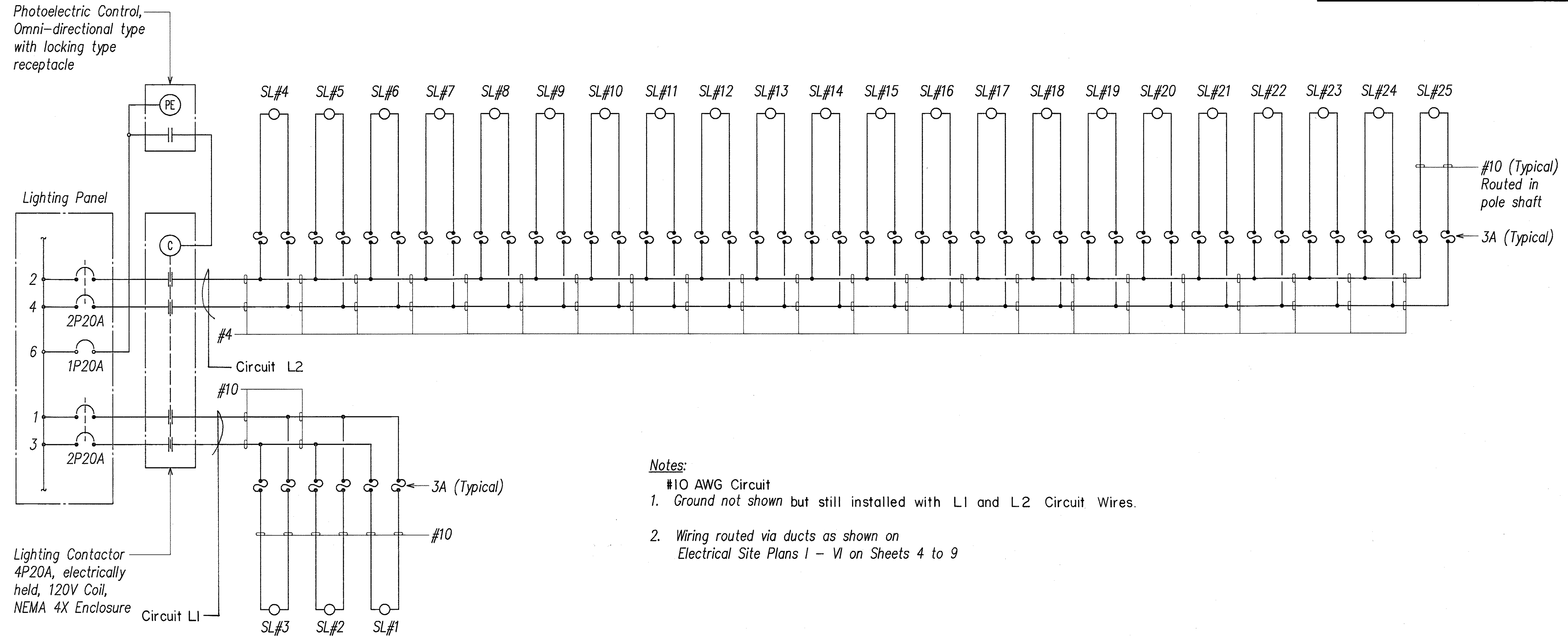
STREET LIGHT CIRCUIT WIRING DIAGRAM
