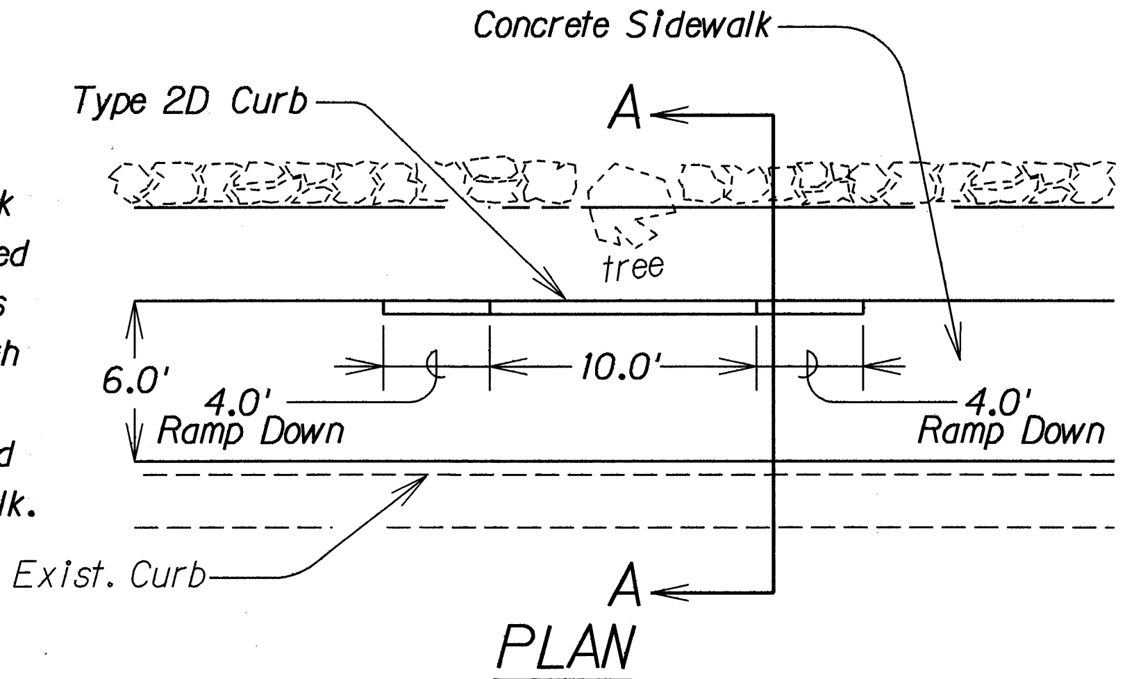
SIDEWALK DETAIL Sta. 95+21± to Sta. 95+39±, Lt. Not to Scale
