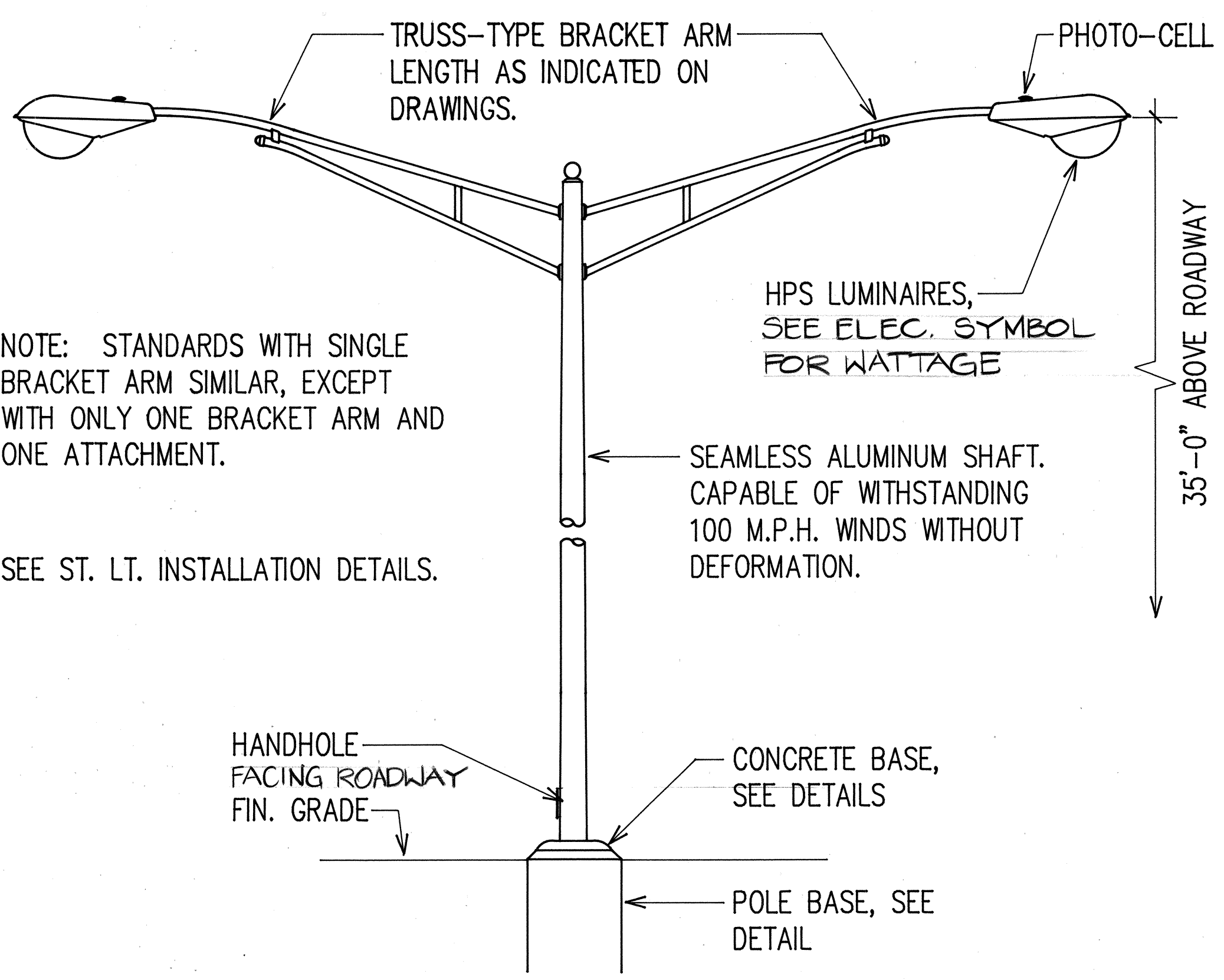
A SLIP BASE STREET LIGHT DETAIL 20E NOT TO SCALE
