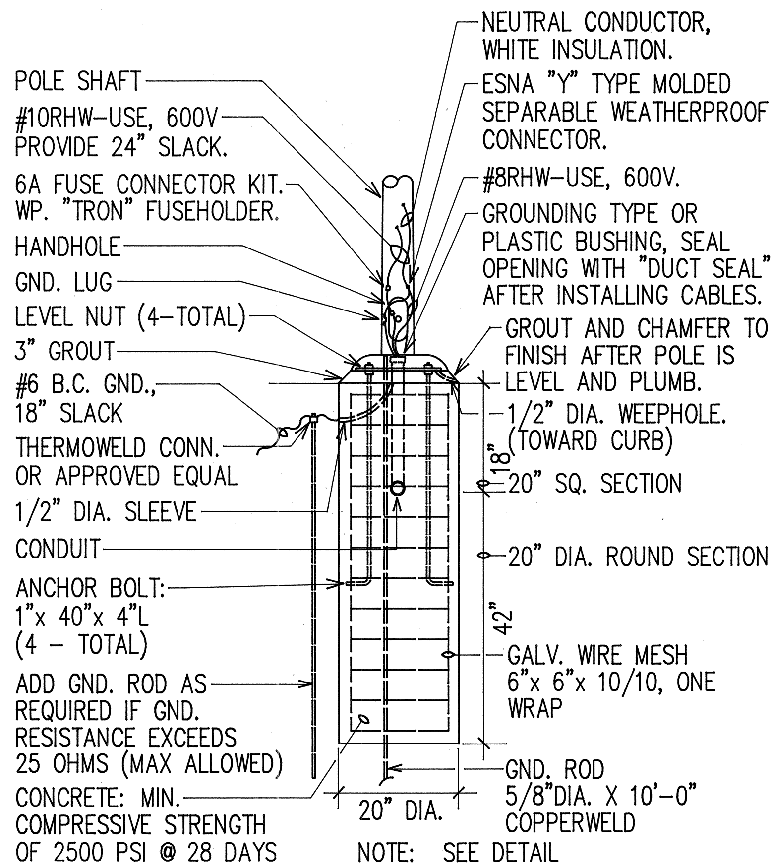
B CONCRETE BASE ELEVATION 20E NOT TO SCALE
