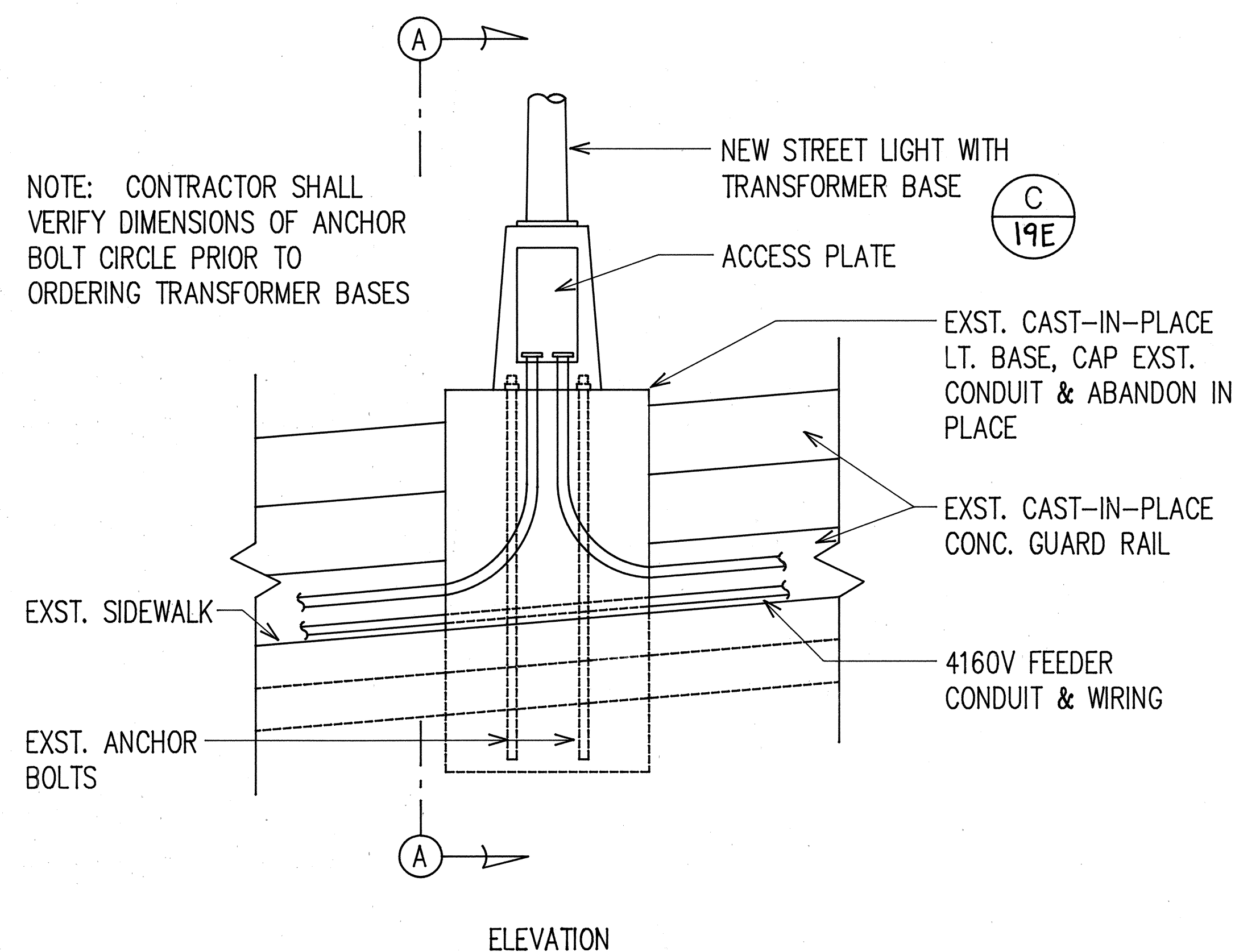
(A) STREET LIGHT INSTALLATION AT EXISTING BASE 19E NOT TO SCALE
