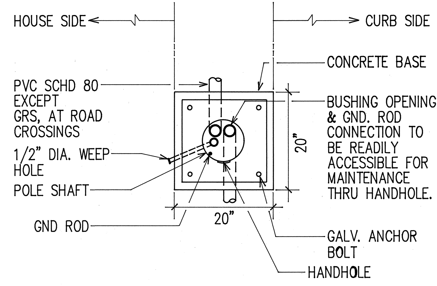
C CONCRETE BASE PLAN 20E NOT TO SCALE
