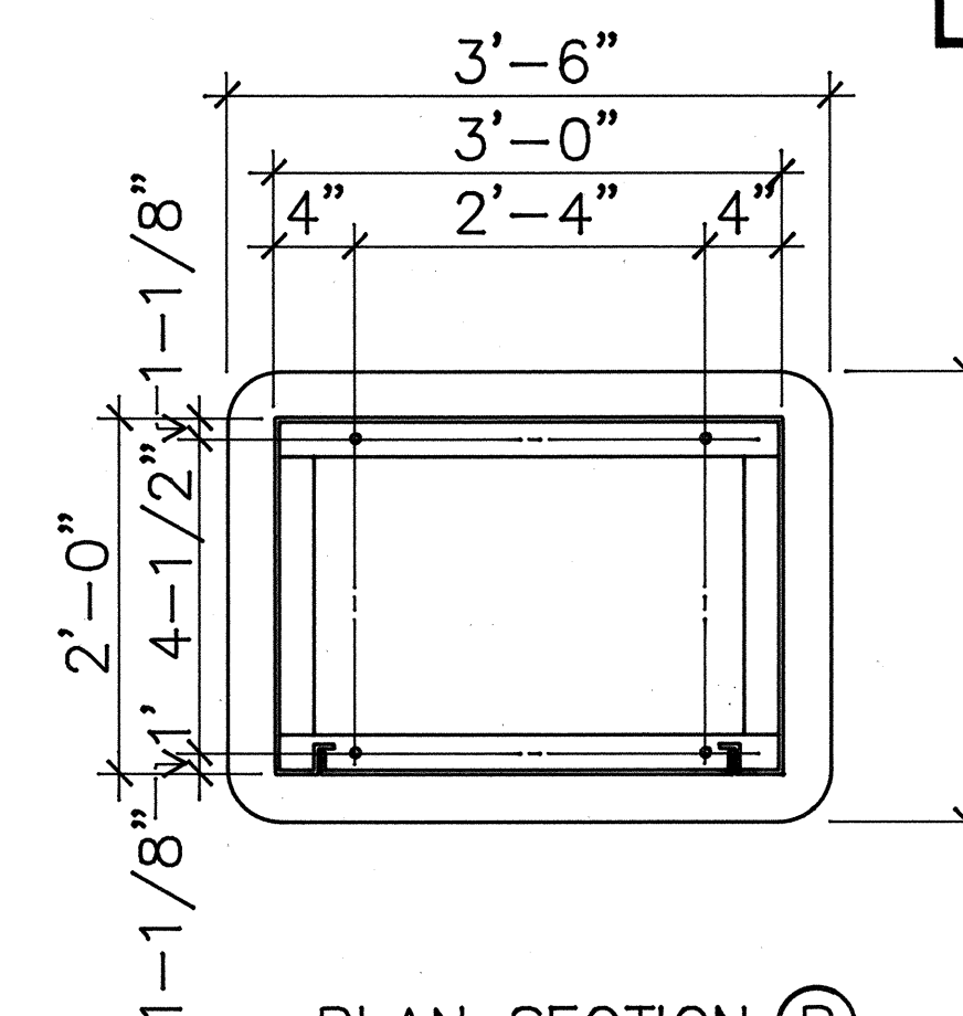
PLAN SECTION (B) (ANGLE FRAME)
