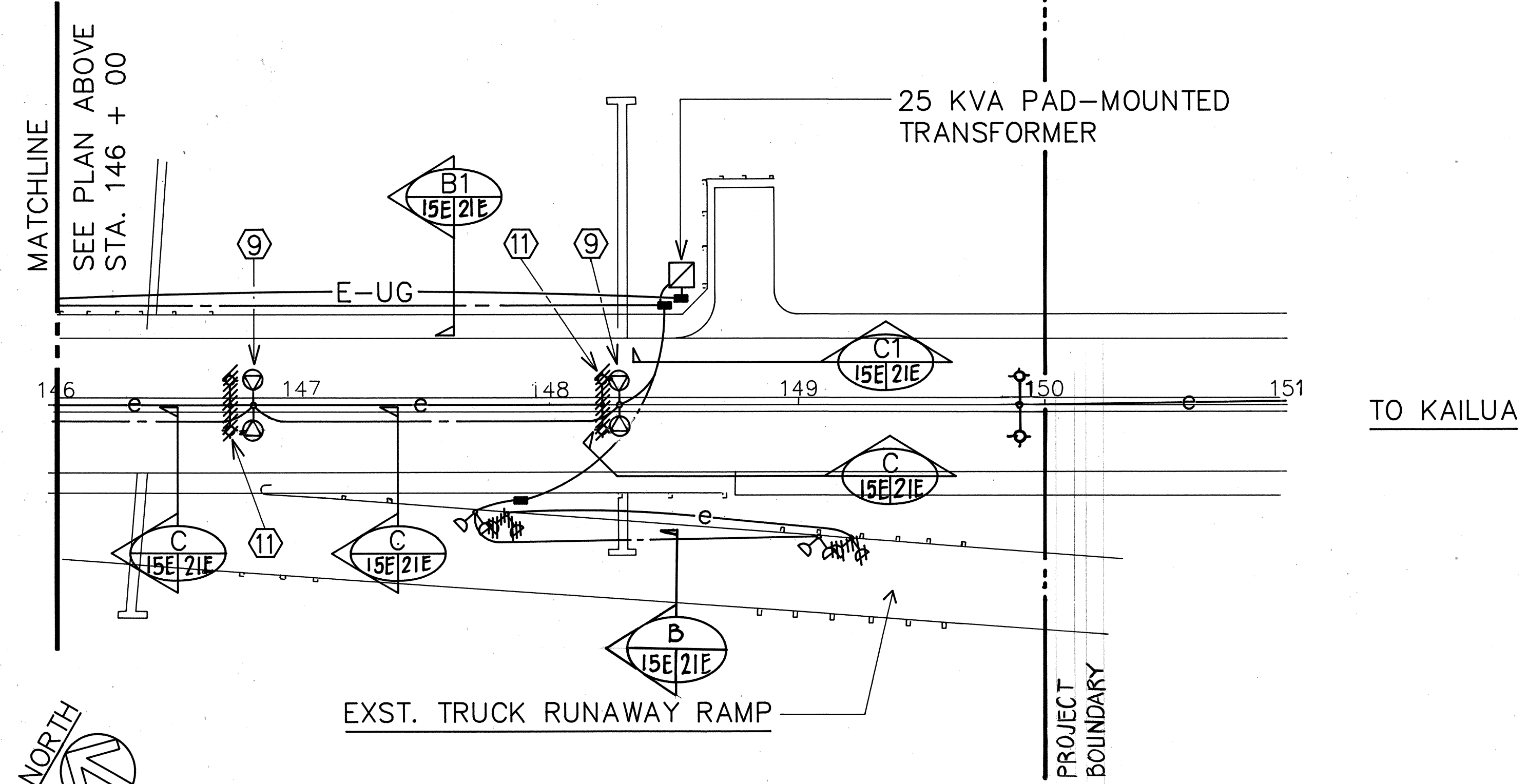
PARTIAL HIGHWAY LIGHTING PLAN - VII SCALE: 1" = 40'-0" SEE STREET LIGHT NOTES, SHT. 13E.
