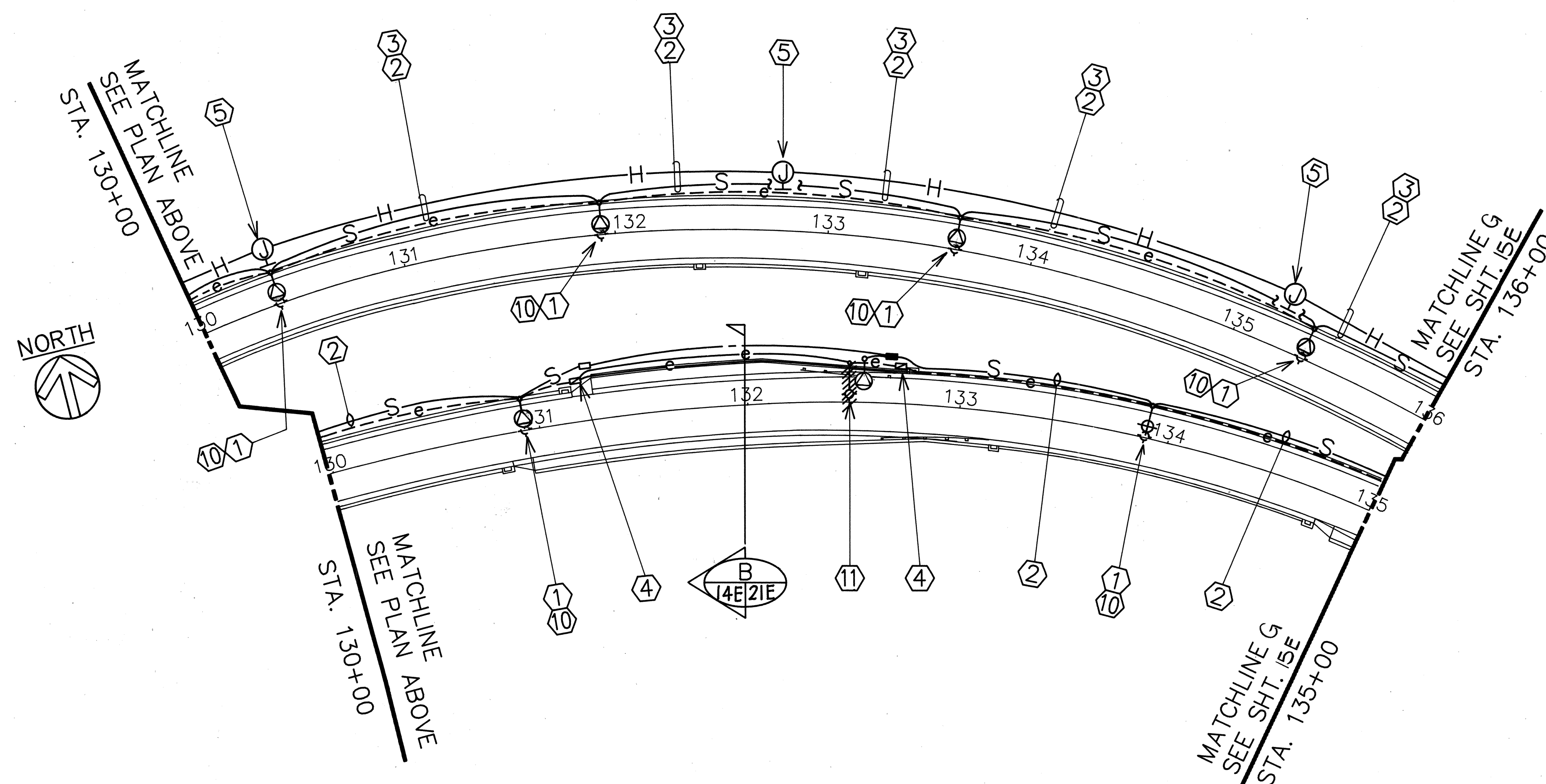
PARTIAL HIGHWAY LIGHTING PLAN - V SCALE: 1"=40'-0" SEE STREET LIGHT NOTES, SHT. 13E
