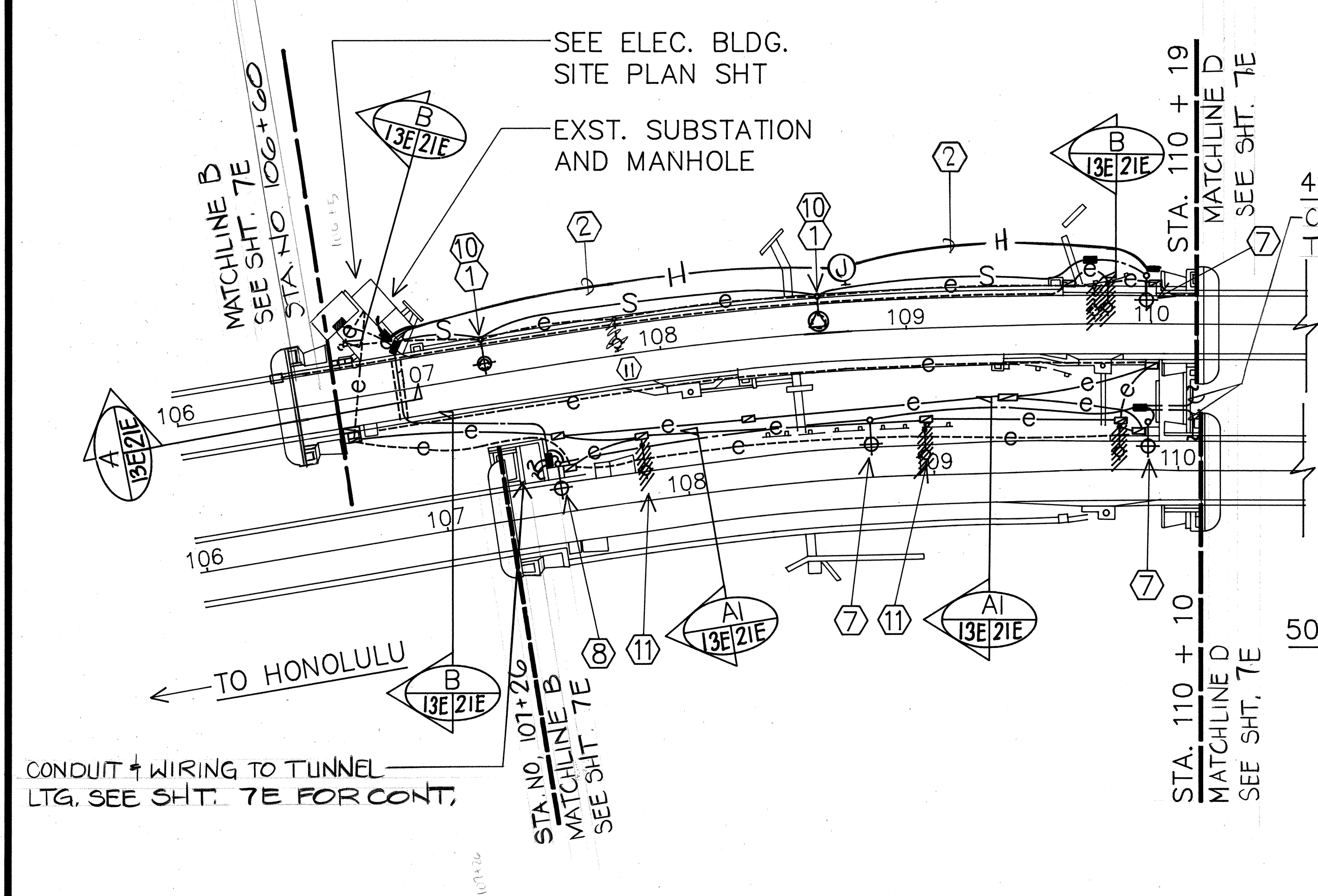
PARTIAL HIGHWAY LIGHTING PLAN - II SCALE: 1" = 40'-0"
