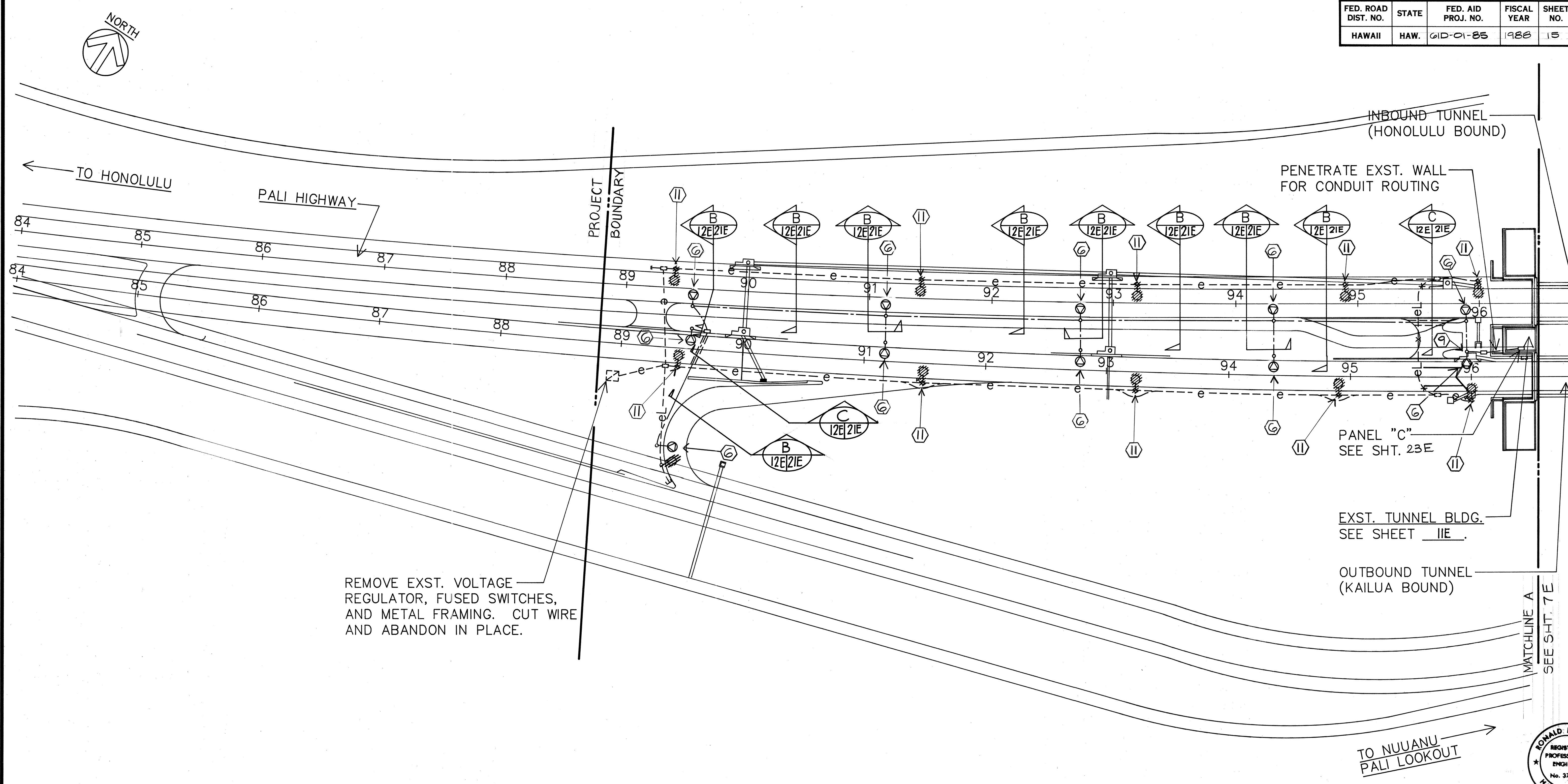
PARTIAL HIGHWAY LIGHTING PLAN - I SCALE: 1" = 40'-0" SEE STREET LIGHT NOTES, SHT. 13E
