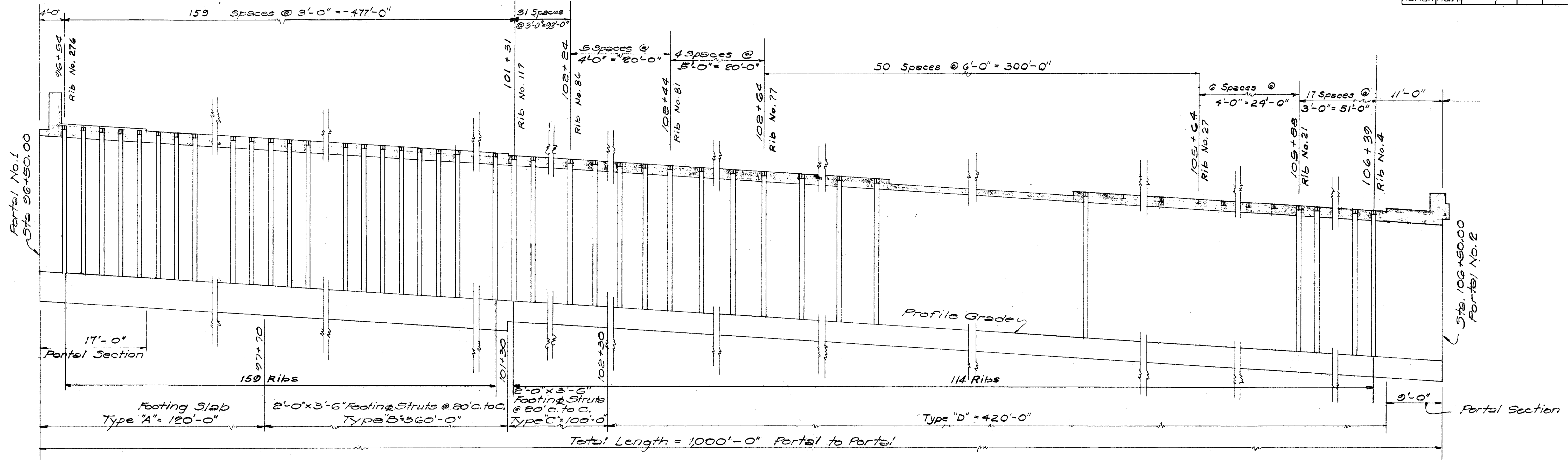
SECTION ALONG 1/8 OF TUNNEL NO. 1 1/8" = 1'-0"
