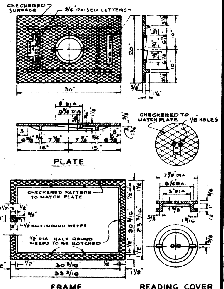
CAST IRON FRAME, PLATE & COVER TYPE II
