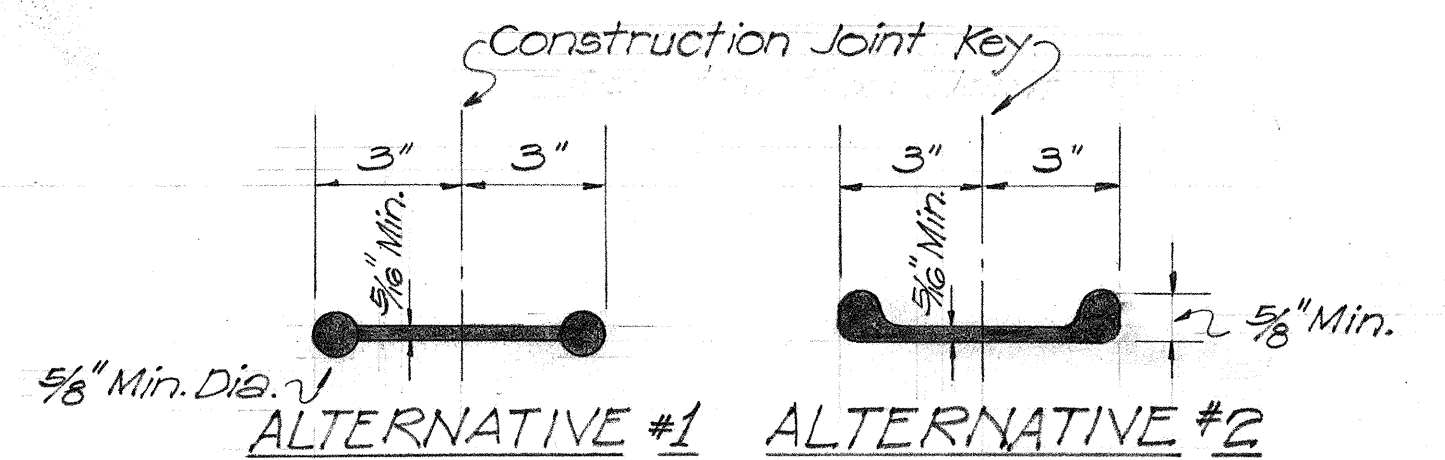
DETAIL OF RUBBER WATERSTOP At Construction Joints in Arch and Walls
