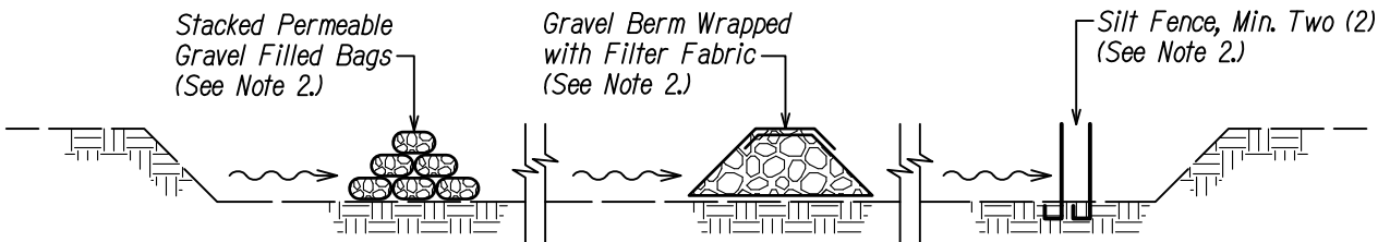
SECTION THROUGH SETTLING BASIN
