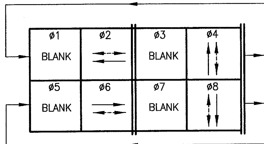
PHASE DIAGRAM NEW MODEL 170 CONTROLLER NEW MODEL 332 CABINET
