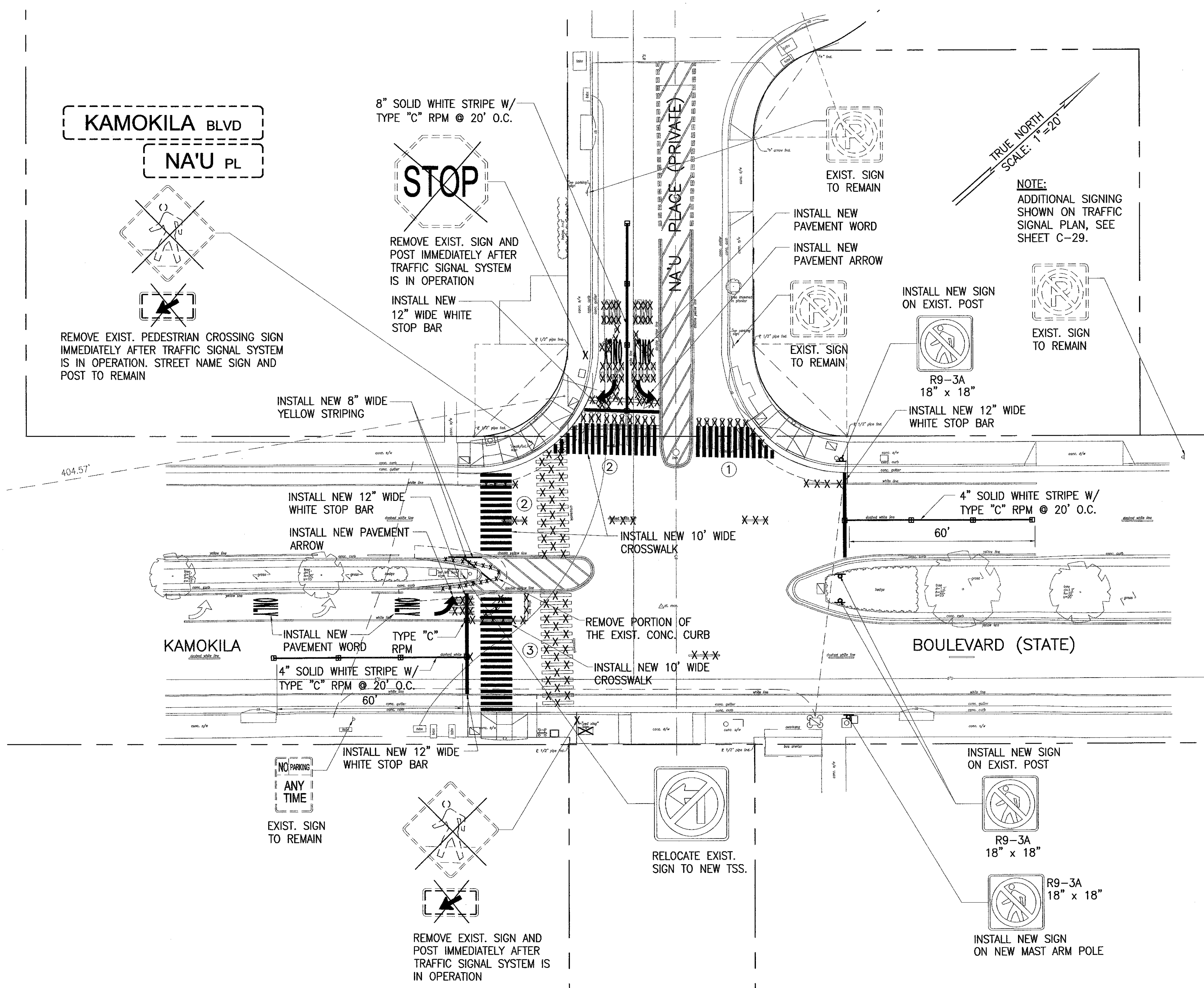
SIGNING AND STRIPING PLAN SCALE: 1"=20'
