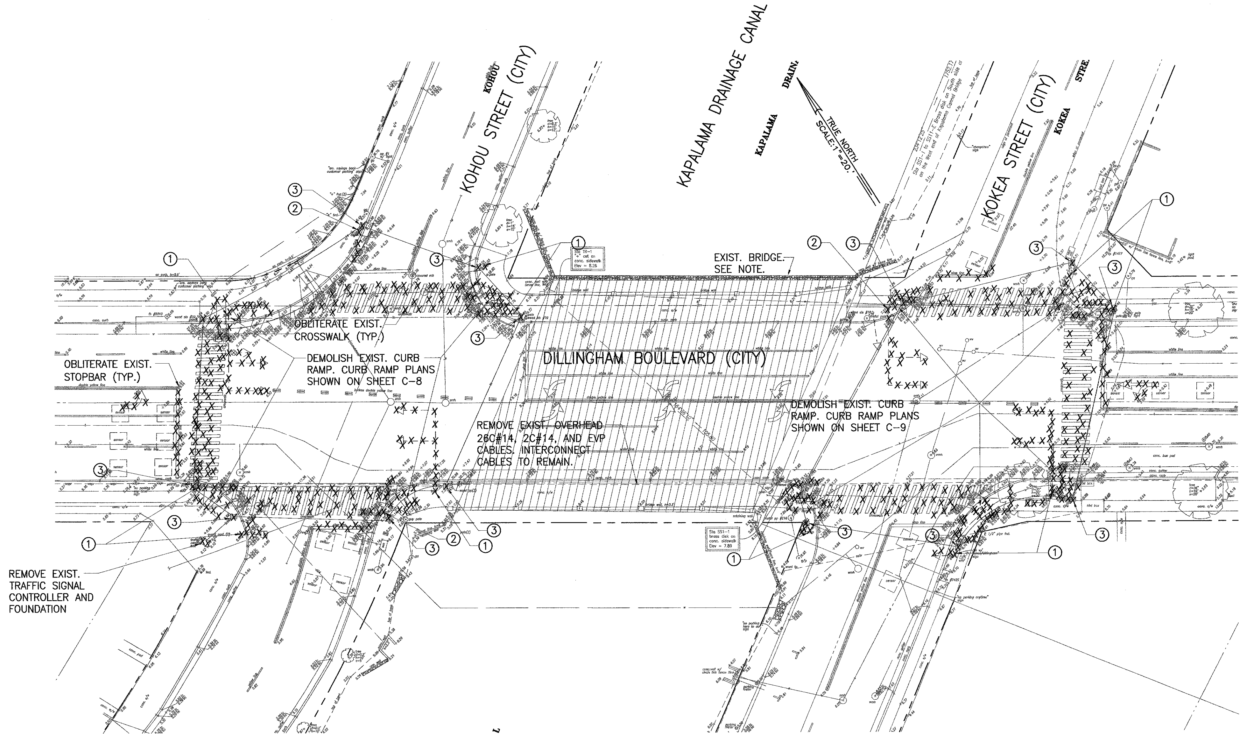
DEMOLITION PLAN SCALE: 1"=20'
