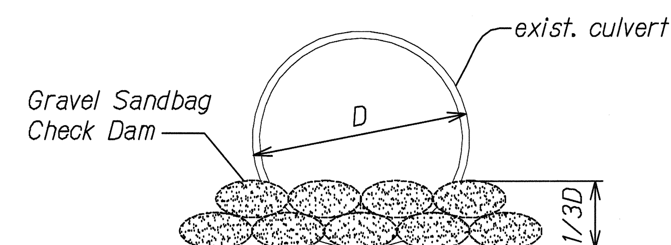
CULVERT PROTECTION DETAIL Not to Scale
