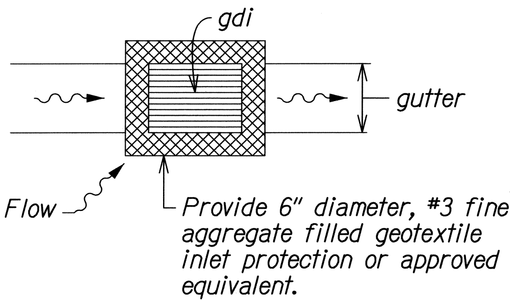
INLET PROTECTION Not to Scale
