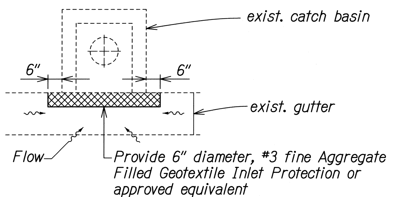
INLET PROTECTION AT EXISTING CATCH BASIN Not to Scale
