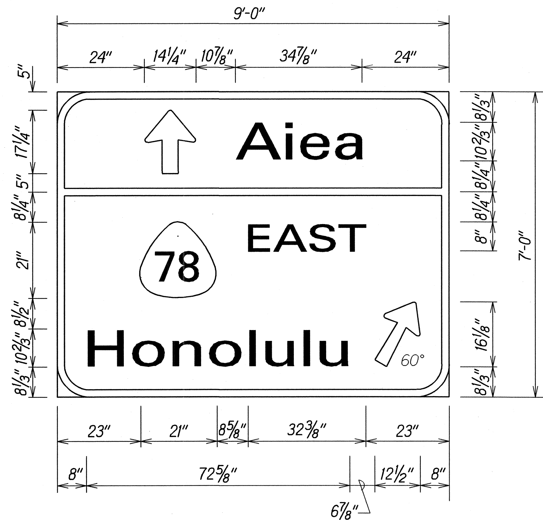
SIGN D-1 Not to Scale
