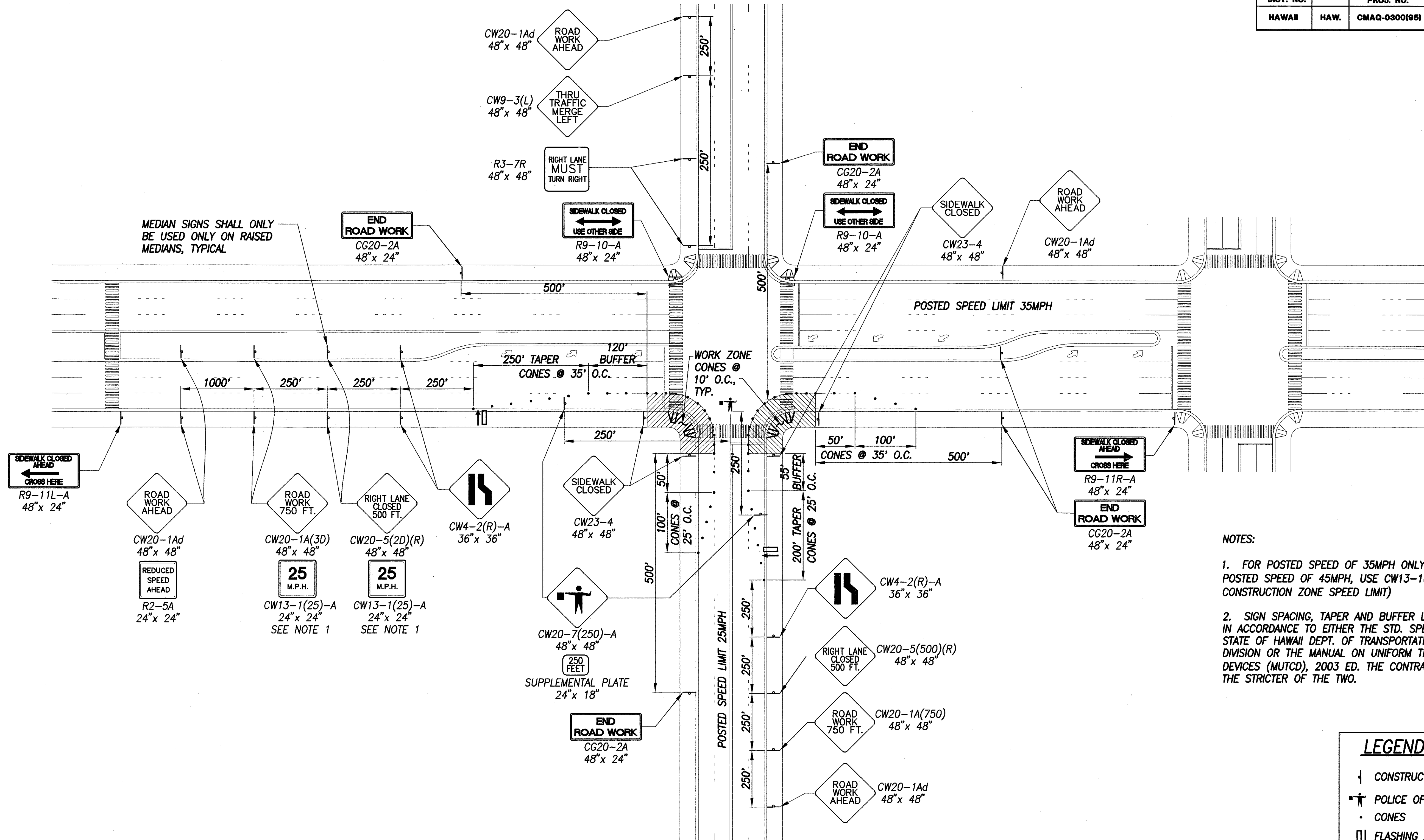
TRAFFIC CONTROL PLAN - CROSS INTERSECTION, DIVIDED HWY. - PHASE 2 SCALE: NTS
