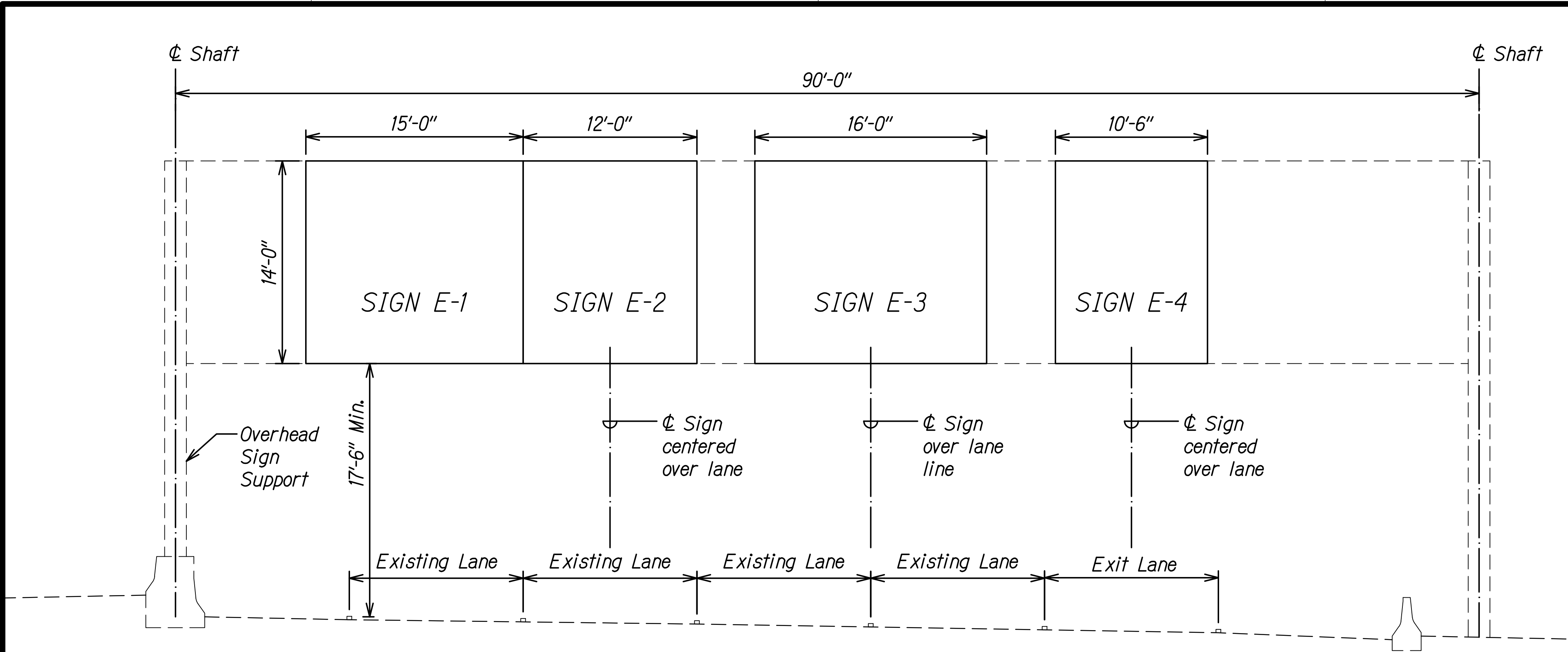
SIGN STRUCTURE H1EBR-253 (FACING DIRECTION OF TRAFFIC) Scale: 1"=5'
