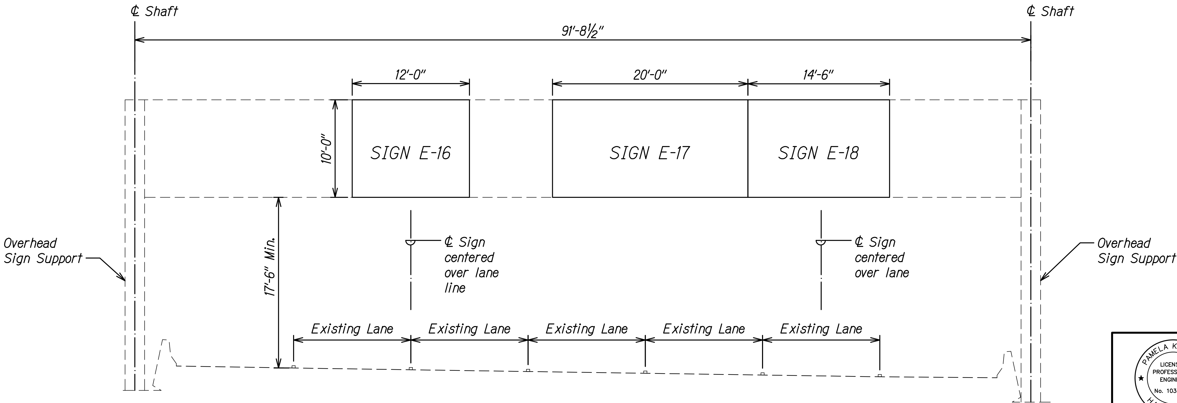
SIGN STRUCTURE HIWB-505 (FACING DIRECTION OF TRAFFIC) Scale: 1"=5'
