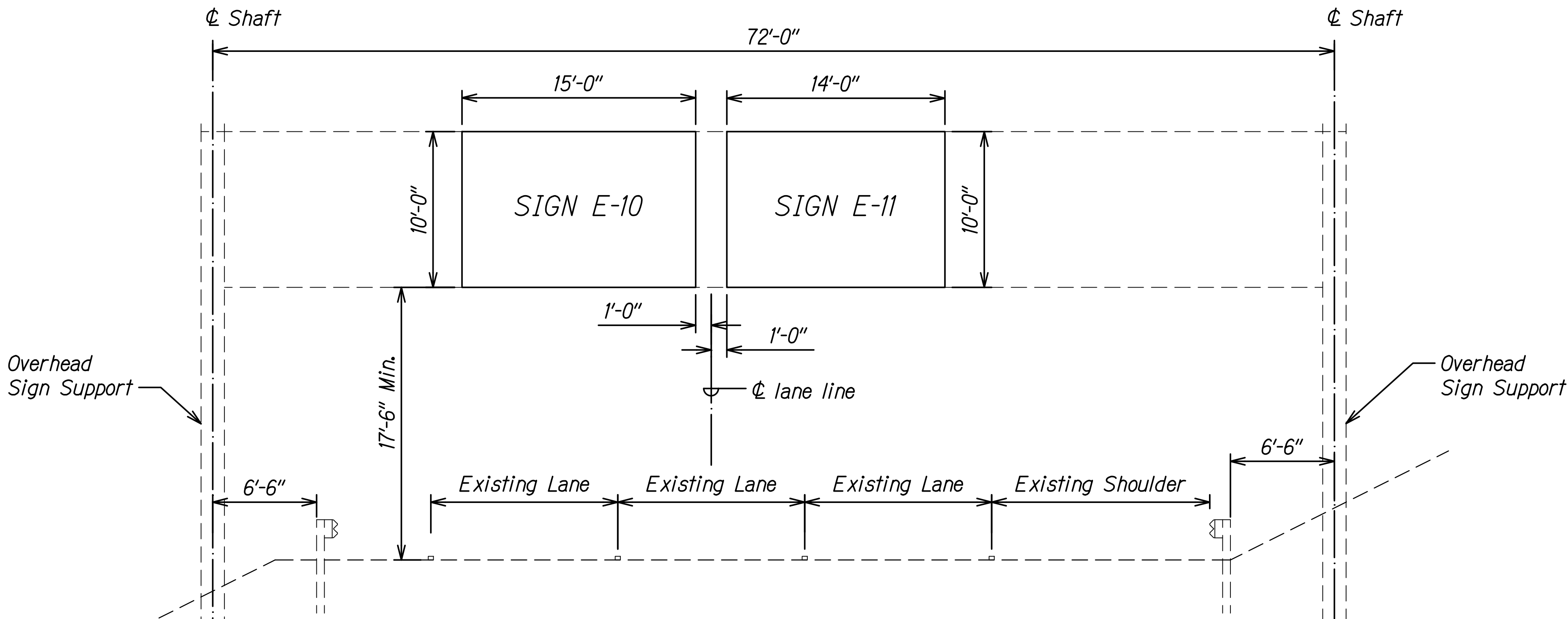
SIGN STRUCTURE 78EBR-830 (FACING DIRECTION OF TRAFFIC) Scale: 1"=5'
