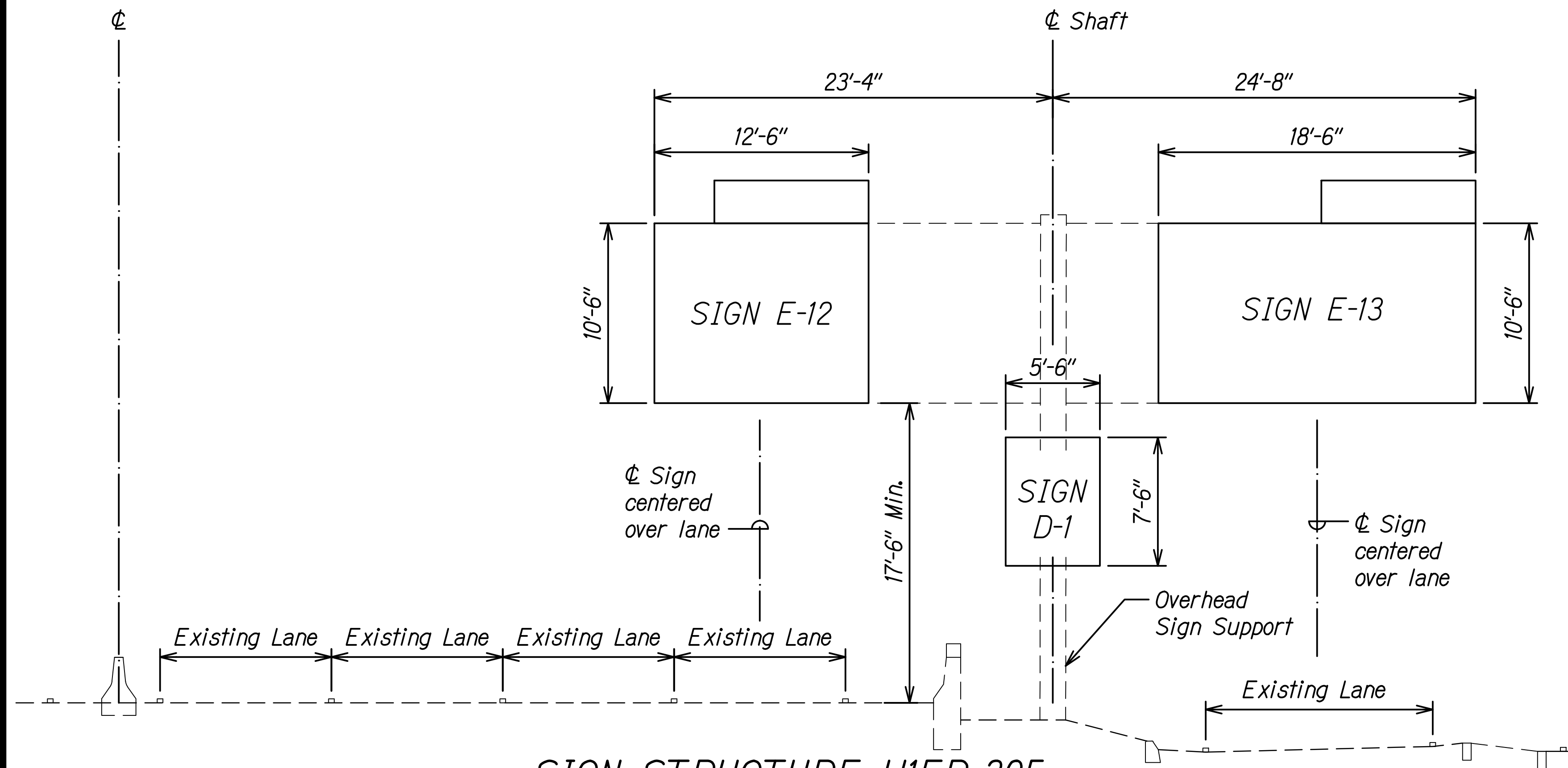
SIGN STRUCTURE HIEB-305 (FACING DIRECTION OF TRAFFIC) Scale: 1"=5'
