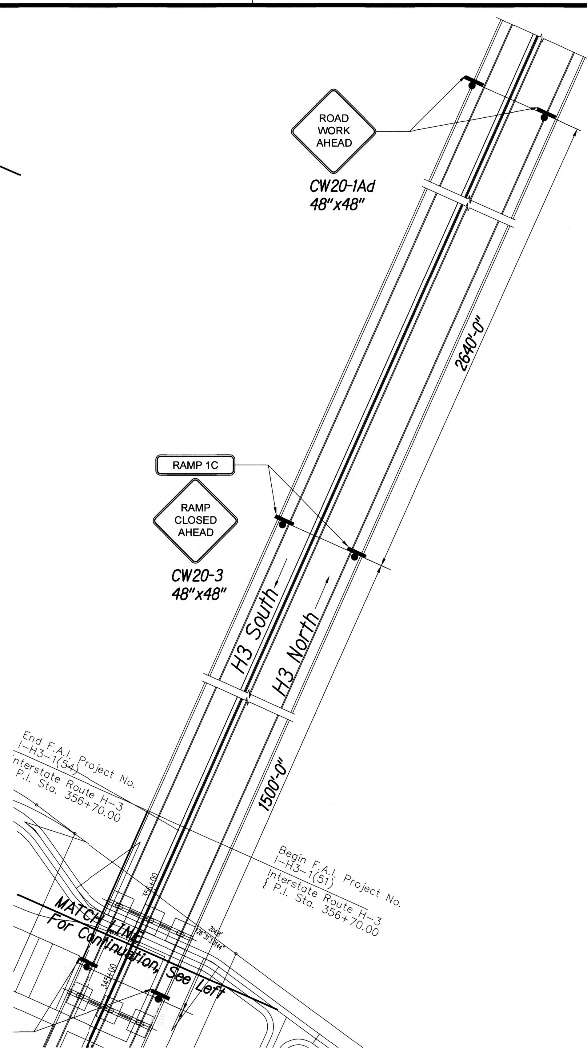
78WBR-871 TRAFFIC CONTROL PLAN-09 PHASE 3 1 Scale: 1" = 60' C13.11 C13.11
