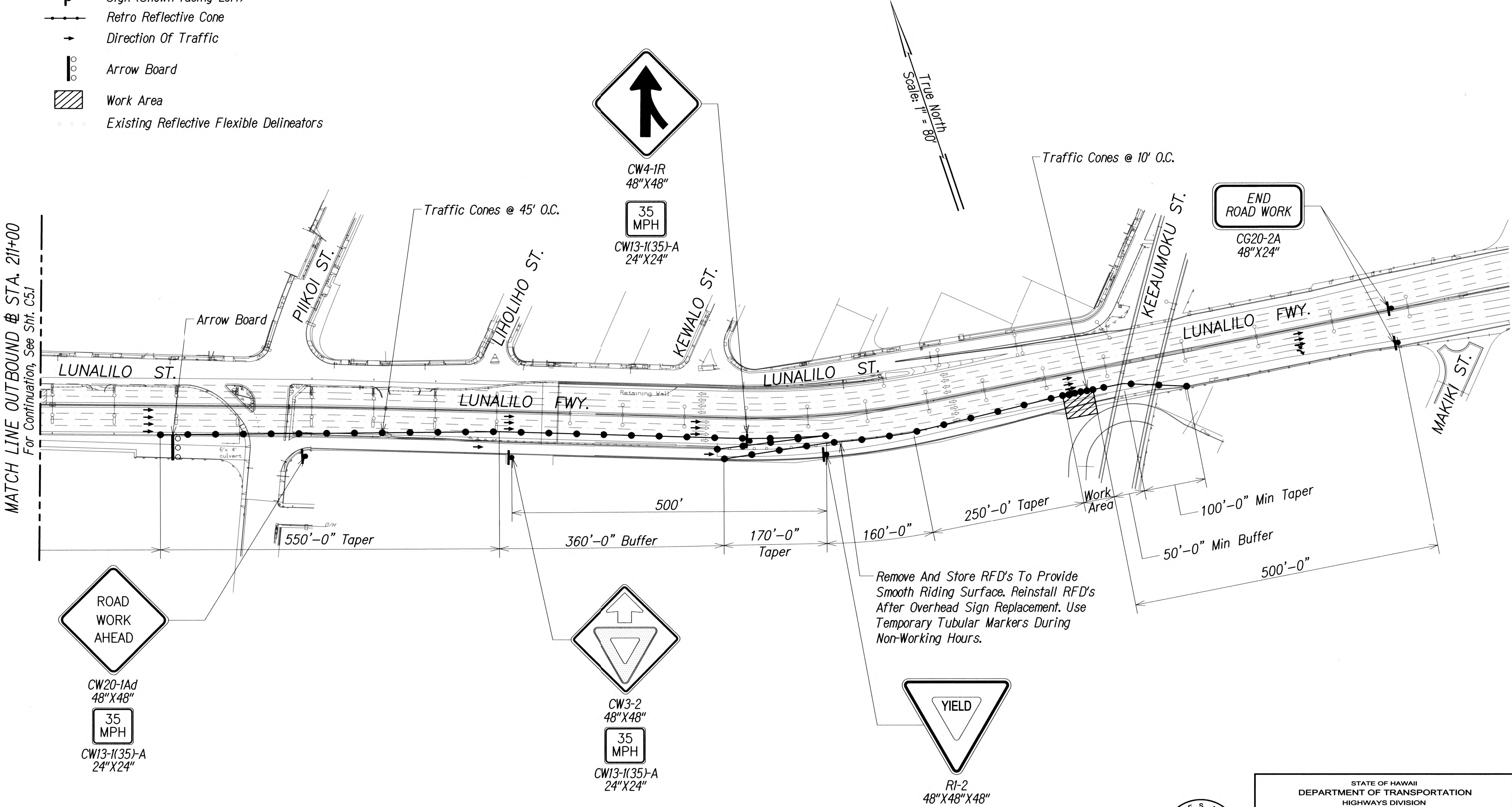
TRAFFIC CONTROL PLAN - PHASE 1 Scale: 1"=80'
