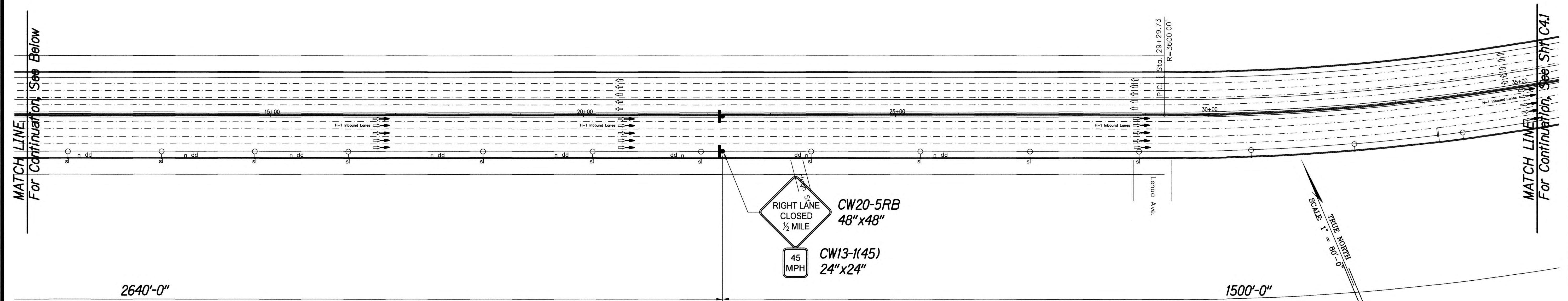
HI EAST BOUND TRAFFIC CONTROL PLAN Scale: 1" = 80'
