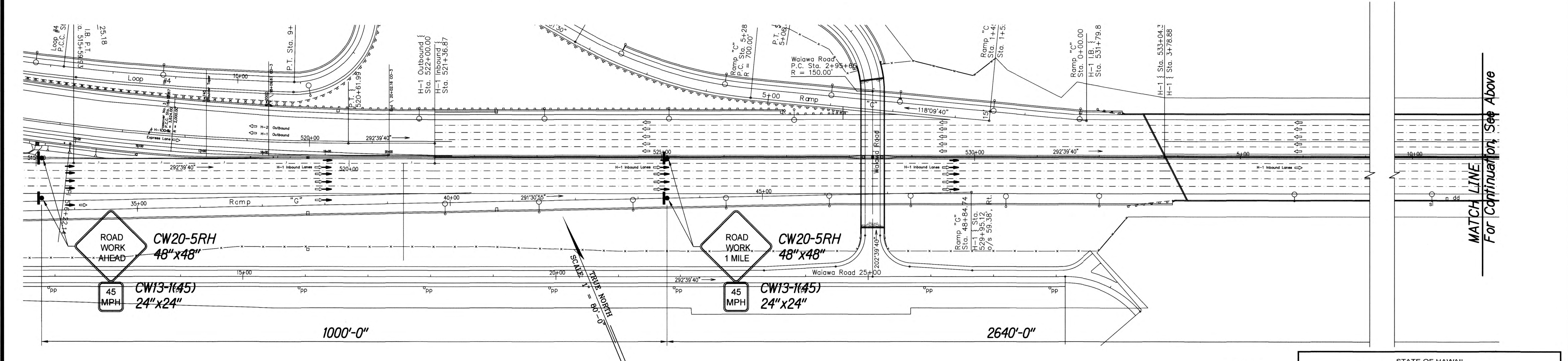
HI EAST BOUND TRAFFIC CONTROL PLAN Scale: 1" = 80'
