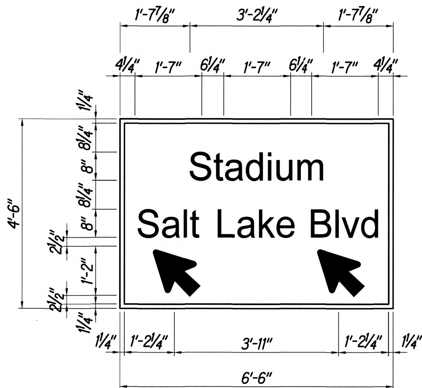
H1WB-418 Not to Scale
