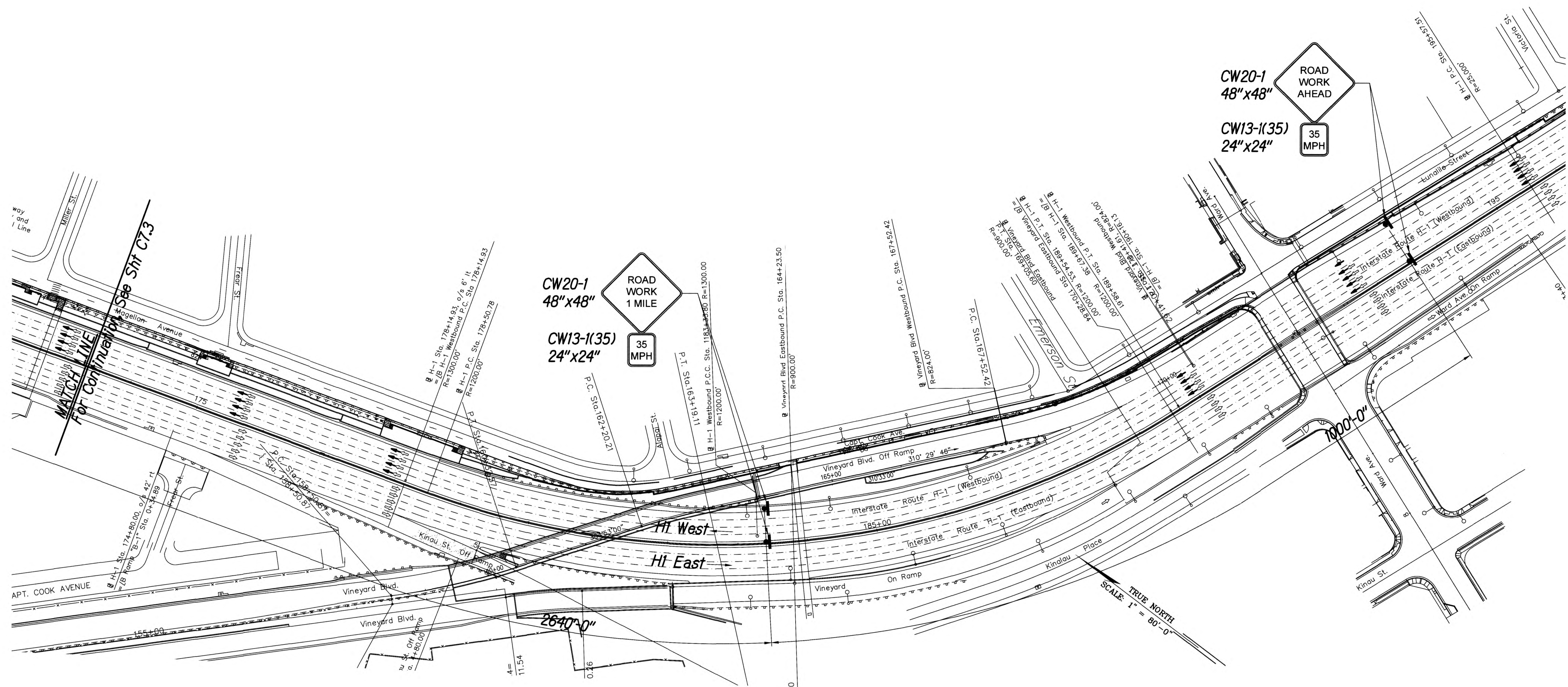
HI WEST BOUND TRAFFIC CONTROL PLAN Scale: 1" = 80'
