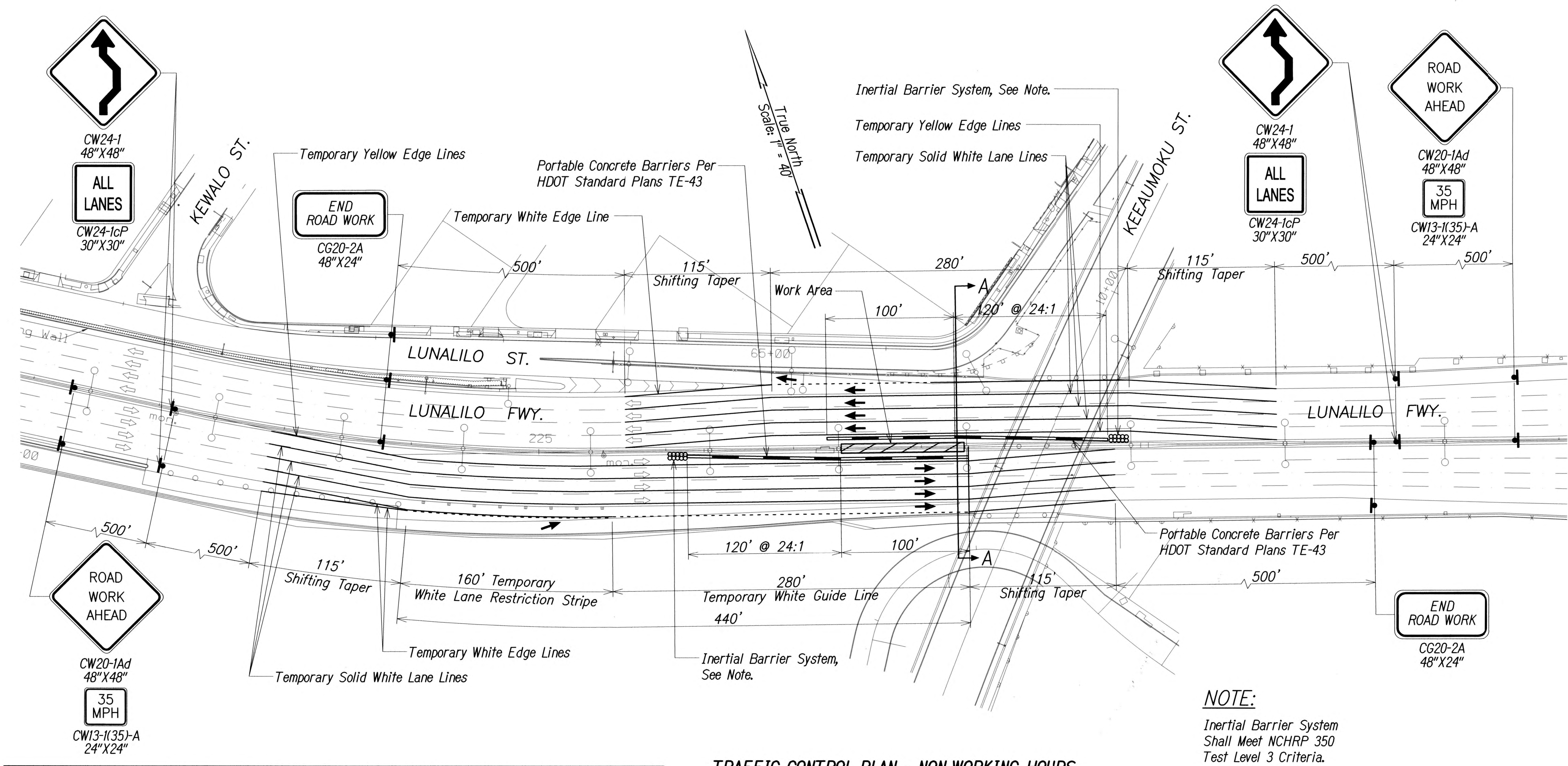
TRAFFIC CONTROL PLAN - NON-WORKING HOURS Scale: 1"=40'
