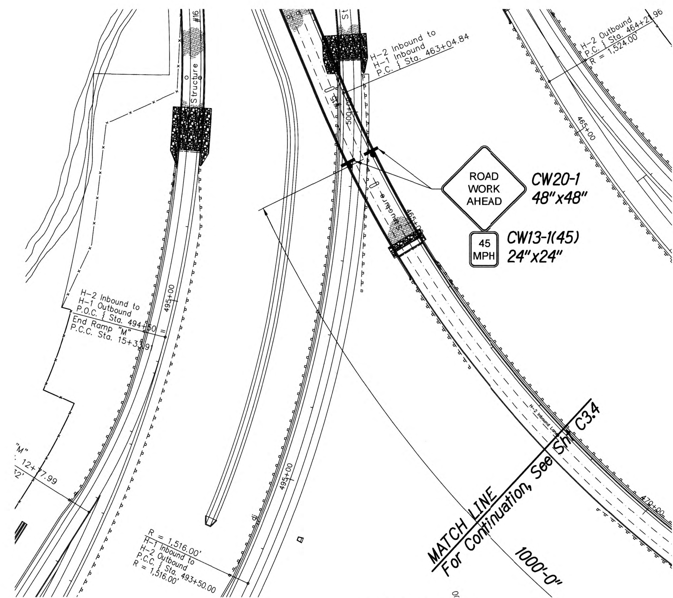
HI EAST BOUND TRAFFIC CONTROL PLAN Scale: 1" = 80'
