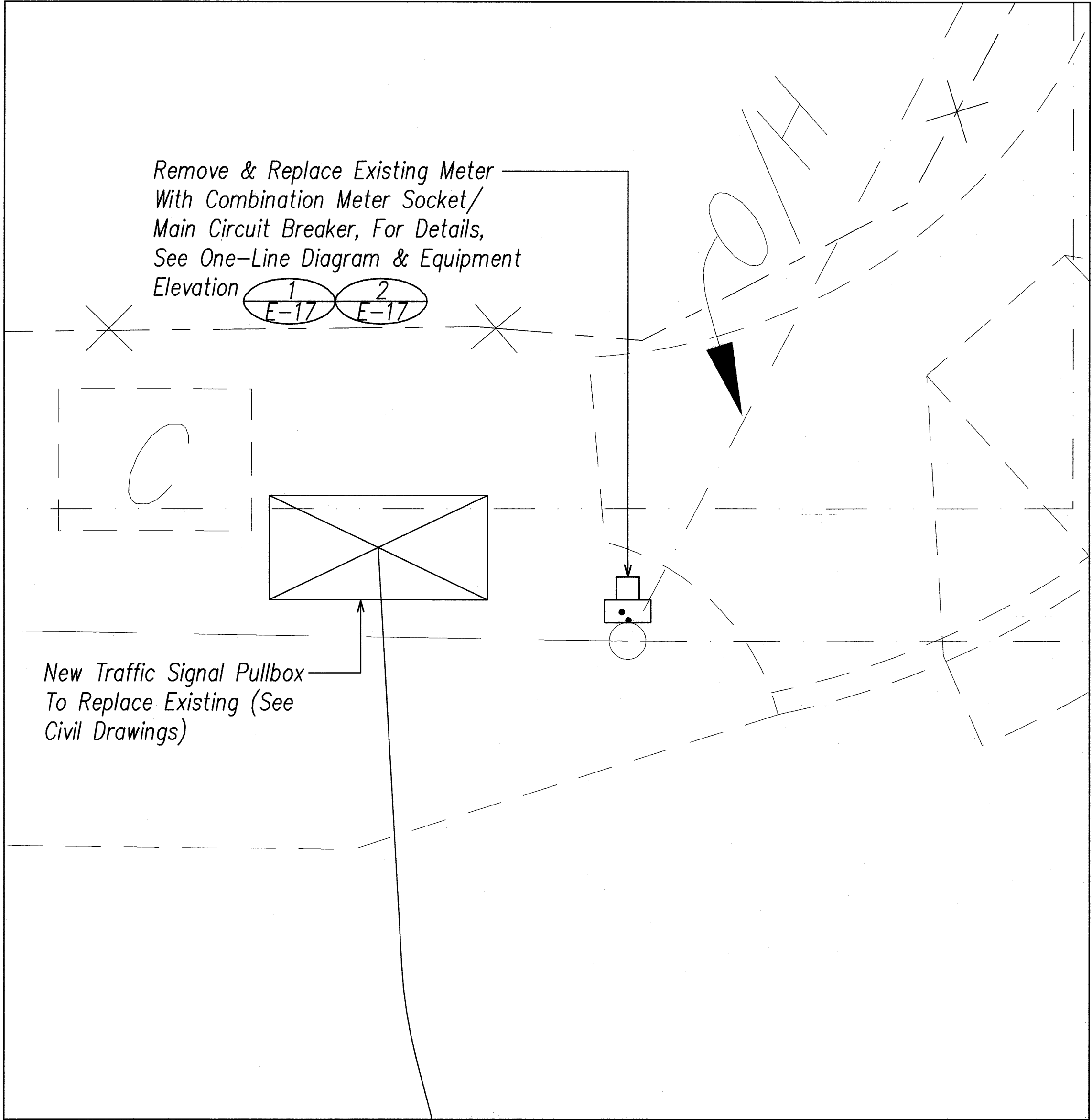
2 New Electrical Meter Enlarged Plan E-16 SCALE: 1"=2'
