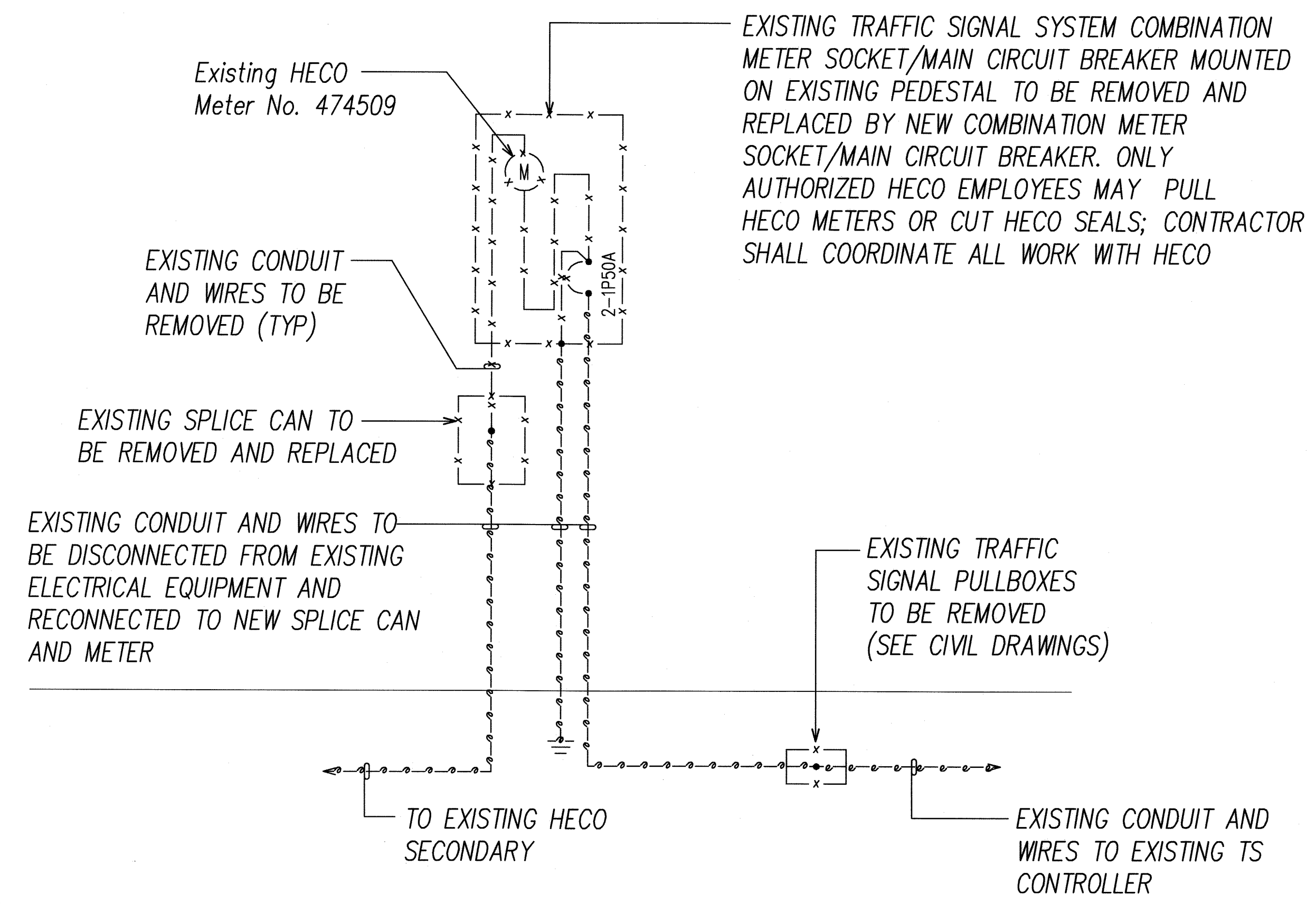
DEMOLITION ONE-LINE DIAGRAM
