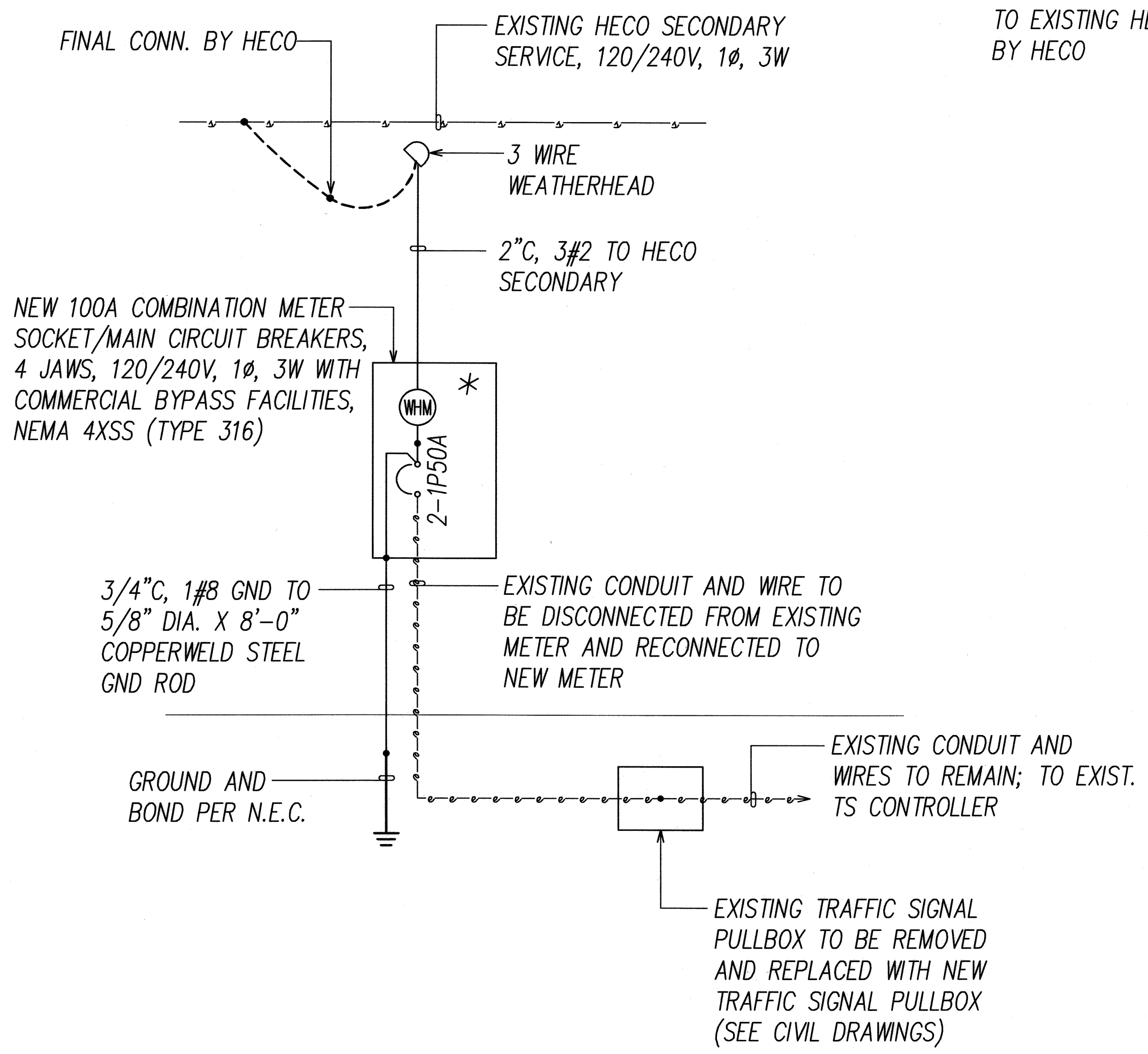
NEW ONE-LINE DIAGRAM
