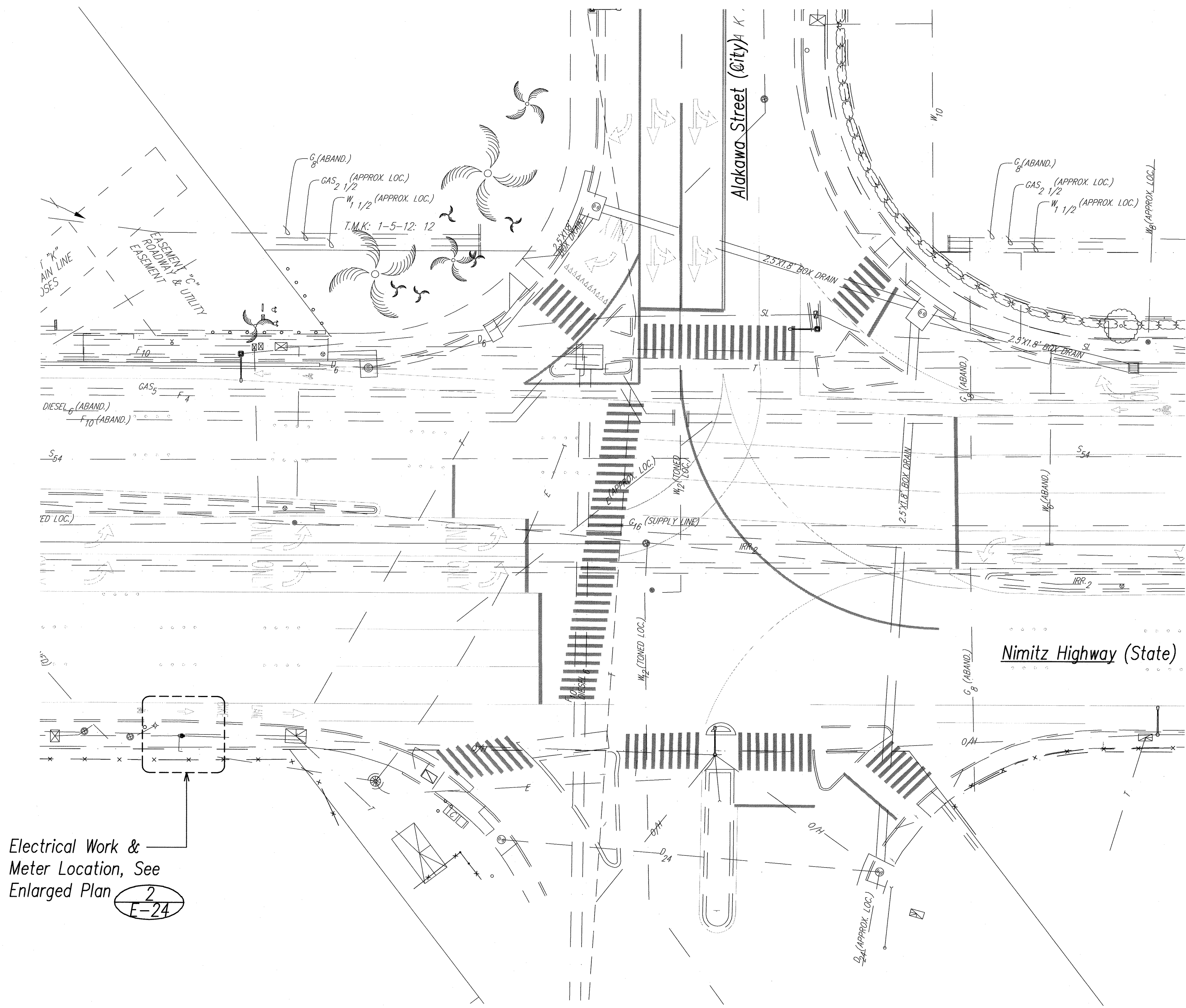
1 E-24 Nimitz Hwy. / Alakawa Street - Electrical Plan SCALE: 1"=20'
