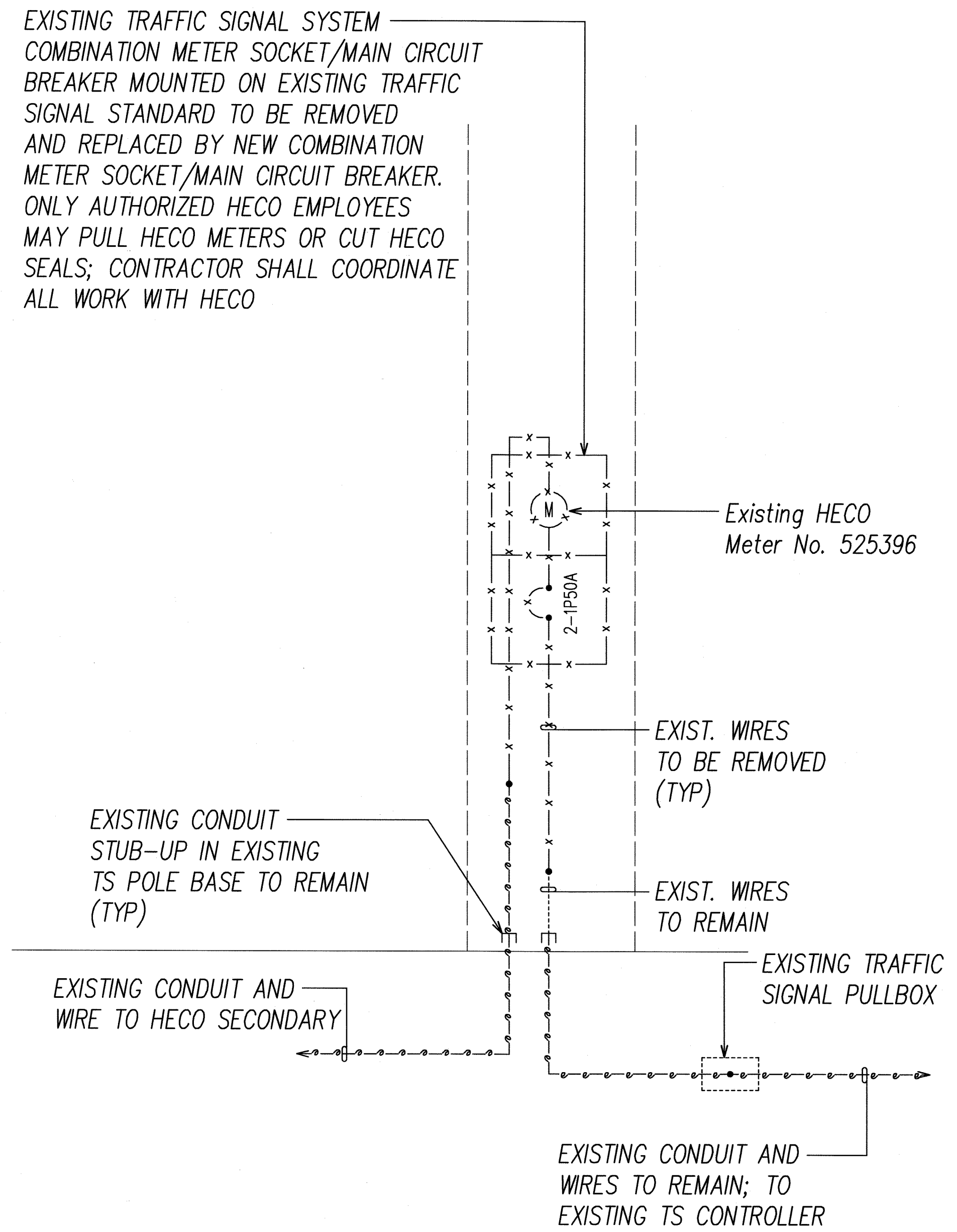
DEMOLITION ONE-LINE DIAGRAM
