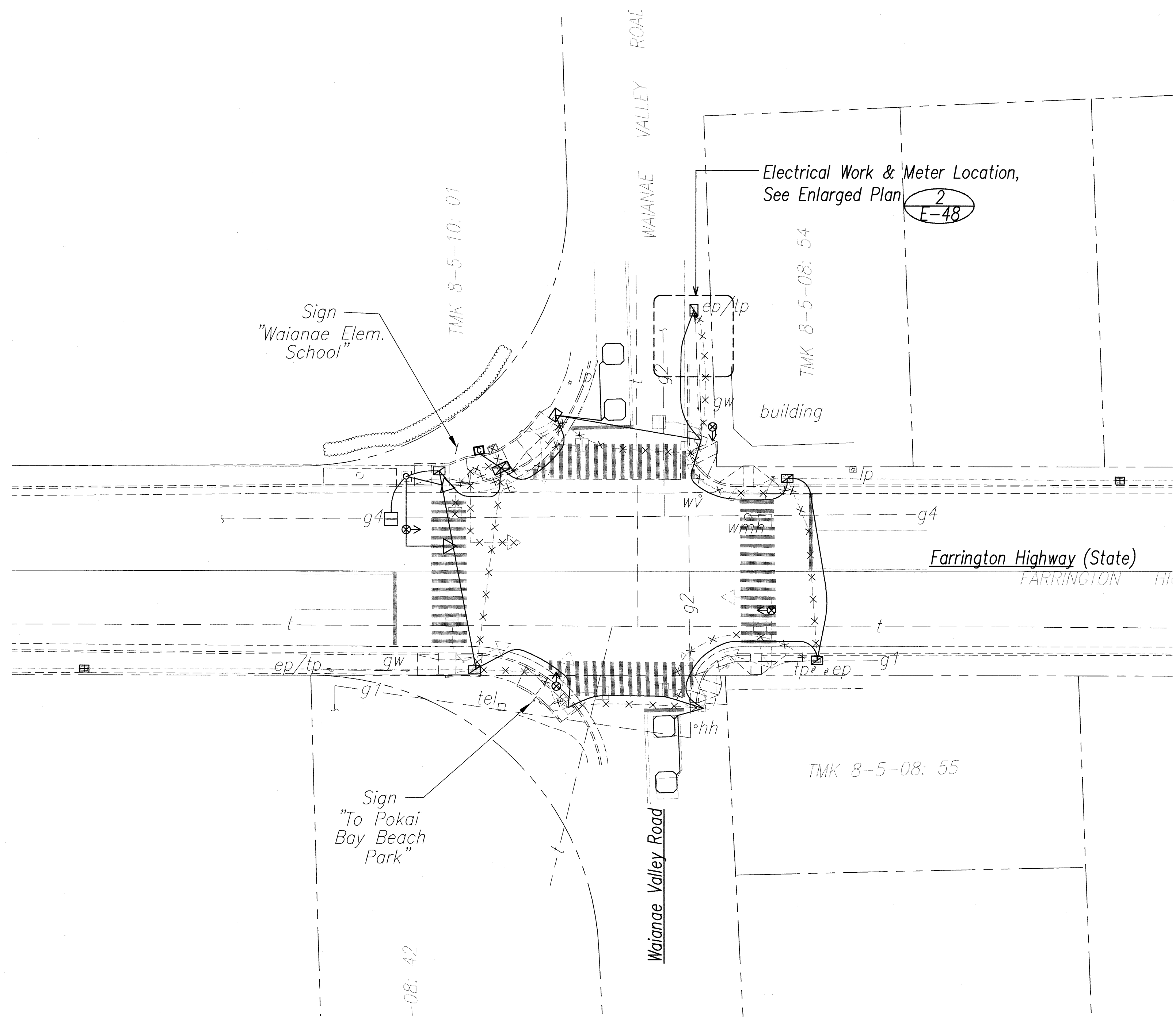
1 Farrington Hwy. / Waianae Valley Road – Electrical Plan E-48 SCALE: 1"=20'
