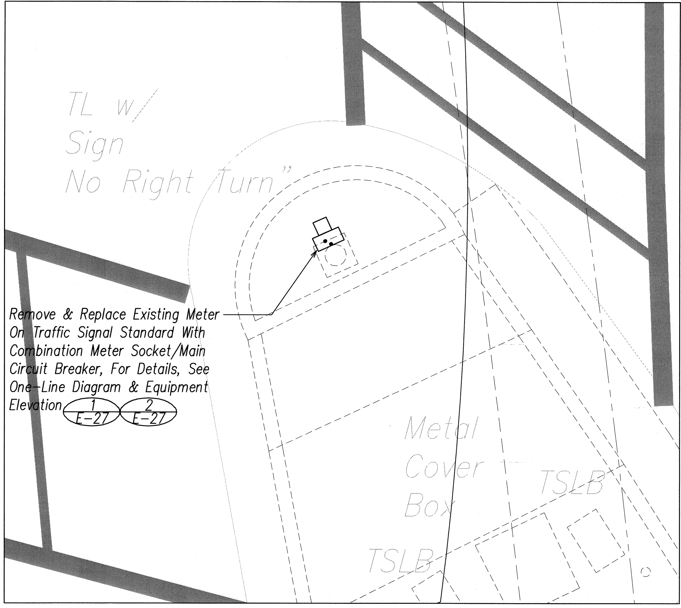
2 E-26 New Electrical Meter Enlarged Plan SCALE: 1"=2' NORTH
