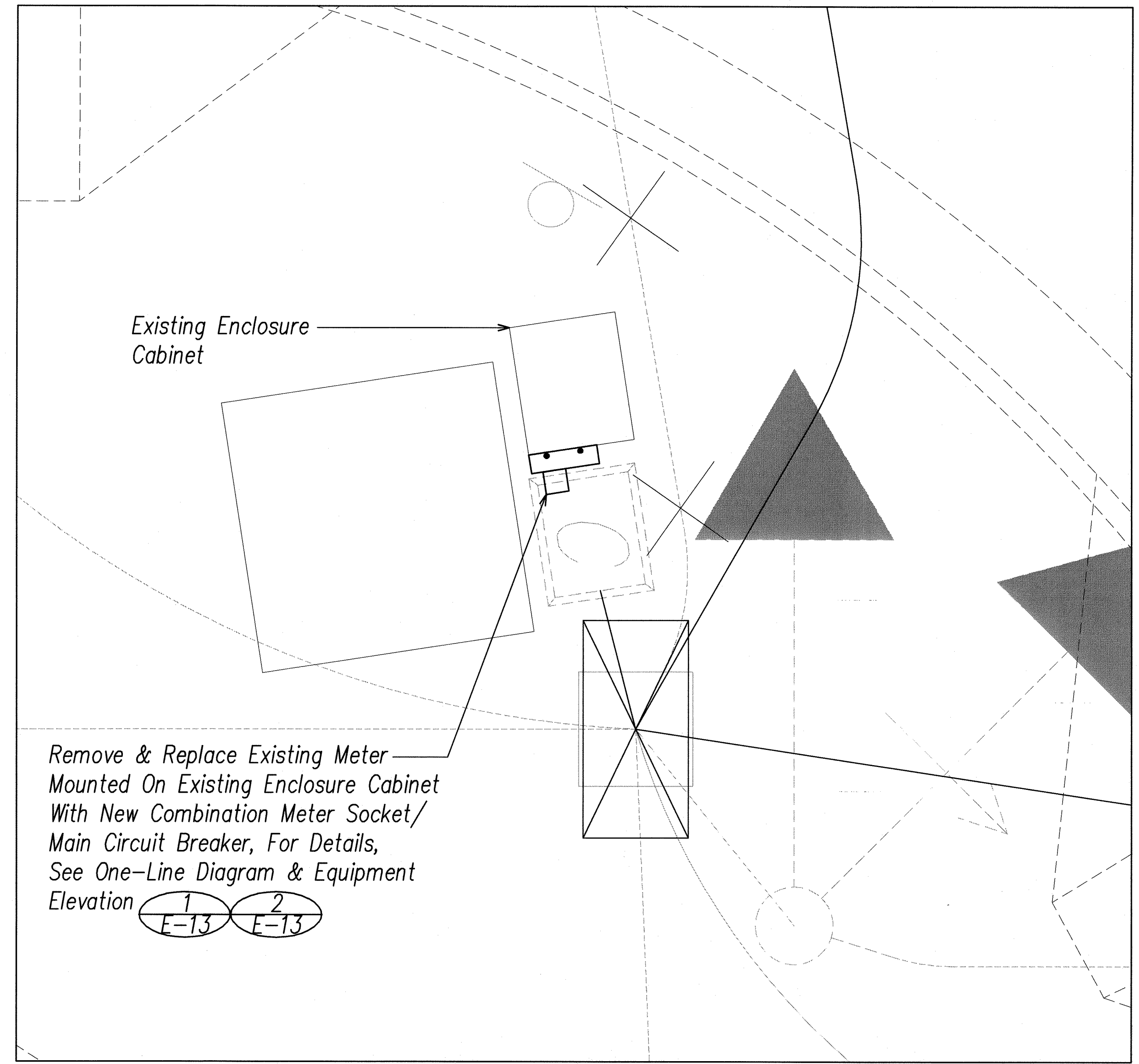
2 E-12 New Electrical Meter Enlarged Plan SCALE: 1"=2'
