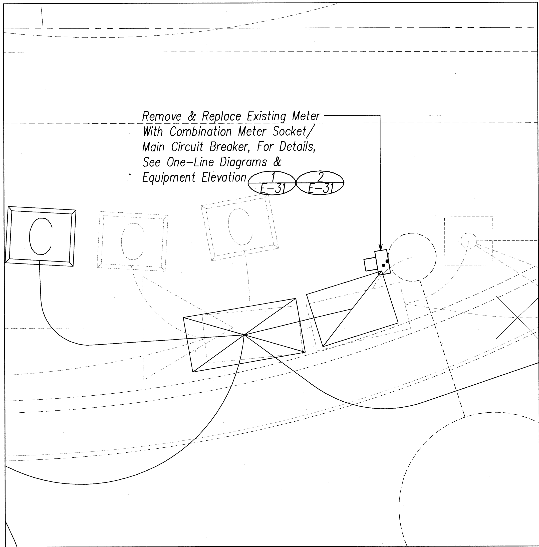
2 E-30 New Electrical Meter Enlarged Plan SCALE: 1"=2'
