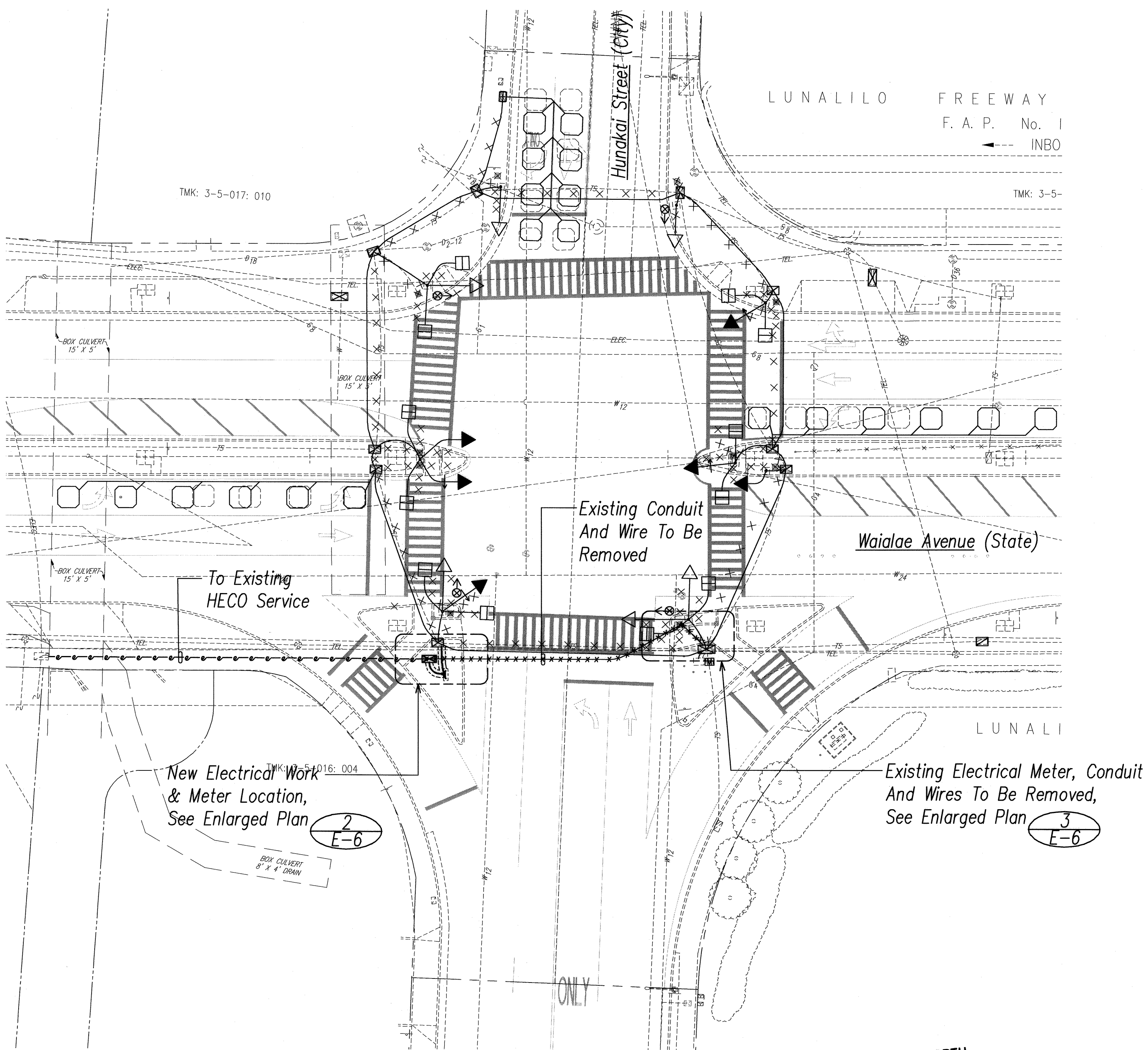
1 E-6 Wai'ala Avenue / Hunakai Street - Electrical Plan SCALE: 1"=20'
