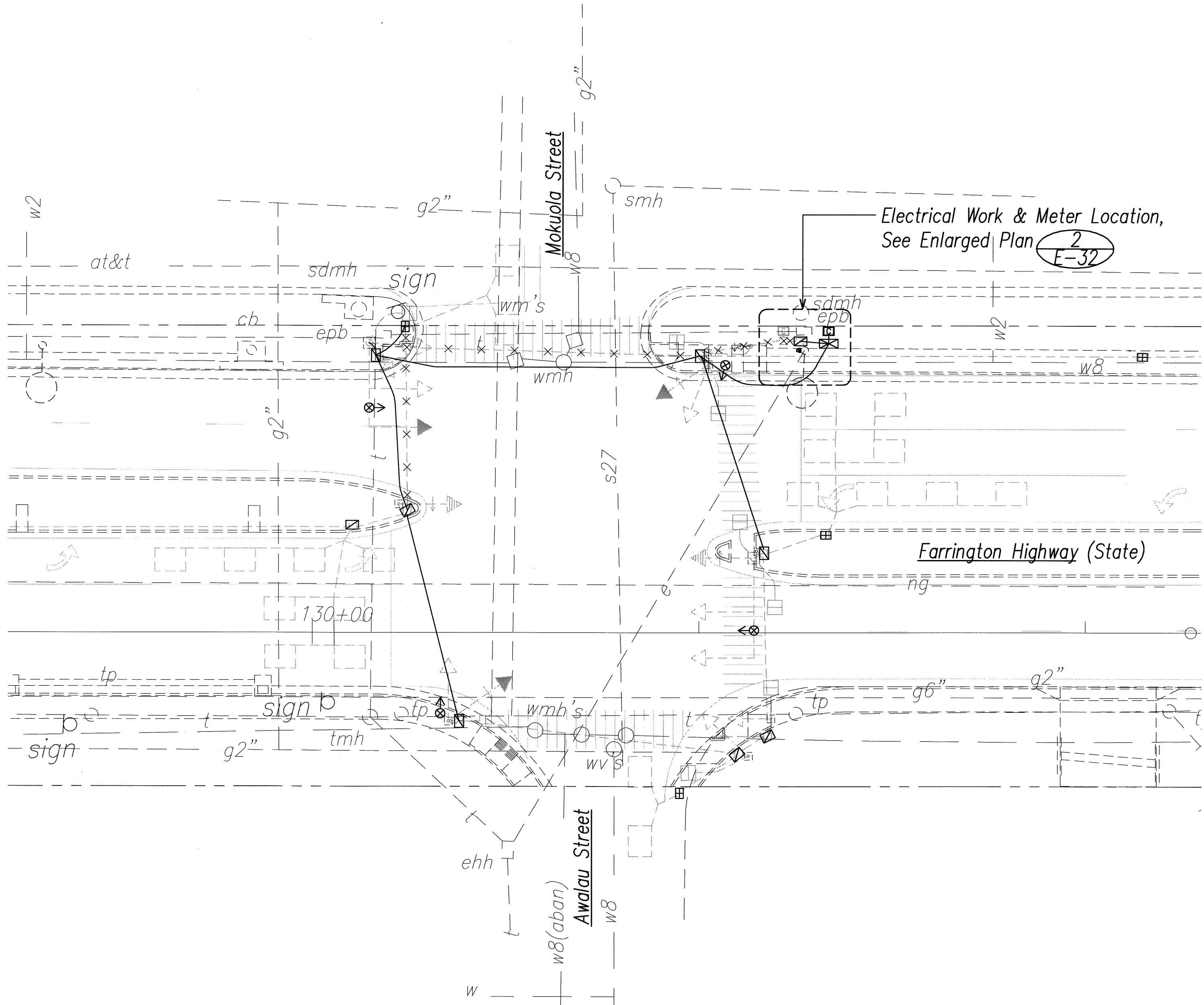
1 E-32 Farrington Hwy. / Mokuola Street - Electrical Plan SCALE: 1"=20'
