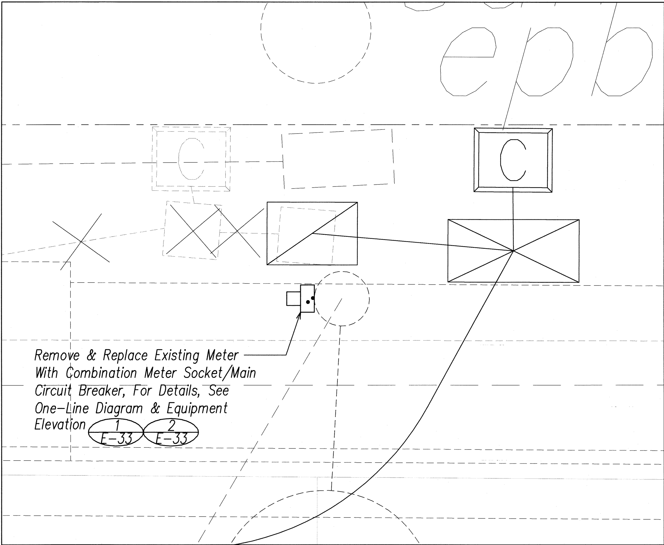
2 E-32 New Electrical Meter Enlarged Plan SCALE: 1"=2'
