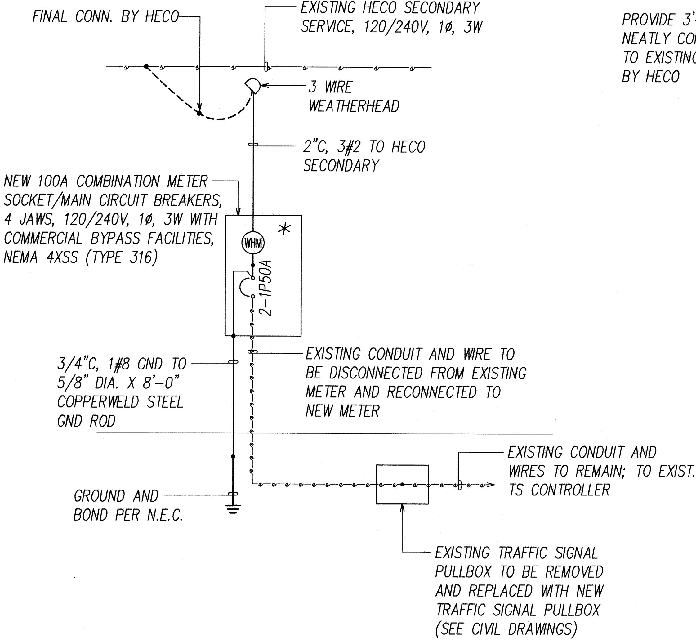
NEW ONE-LINE DIAGRAM
