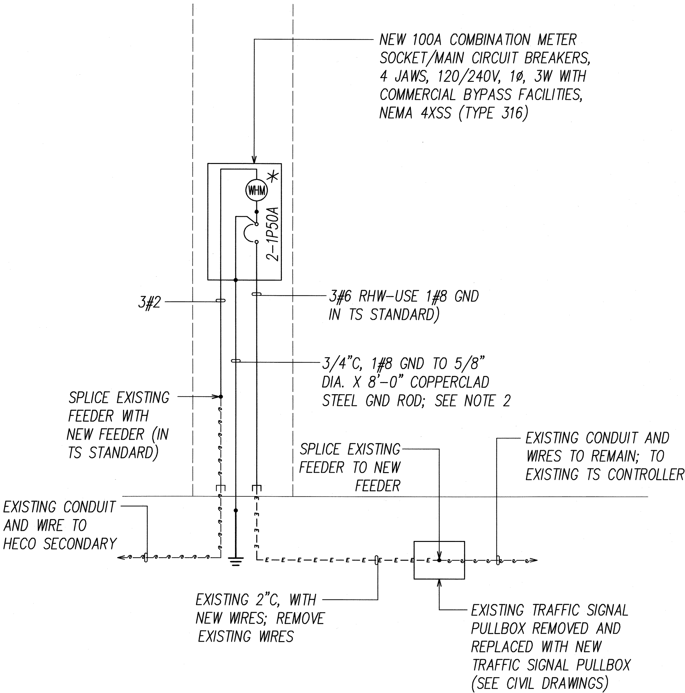
NEW ONE-LINE DIAGRAM
