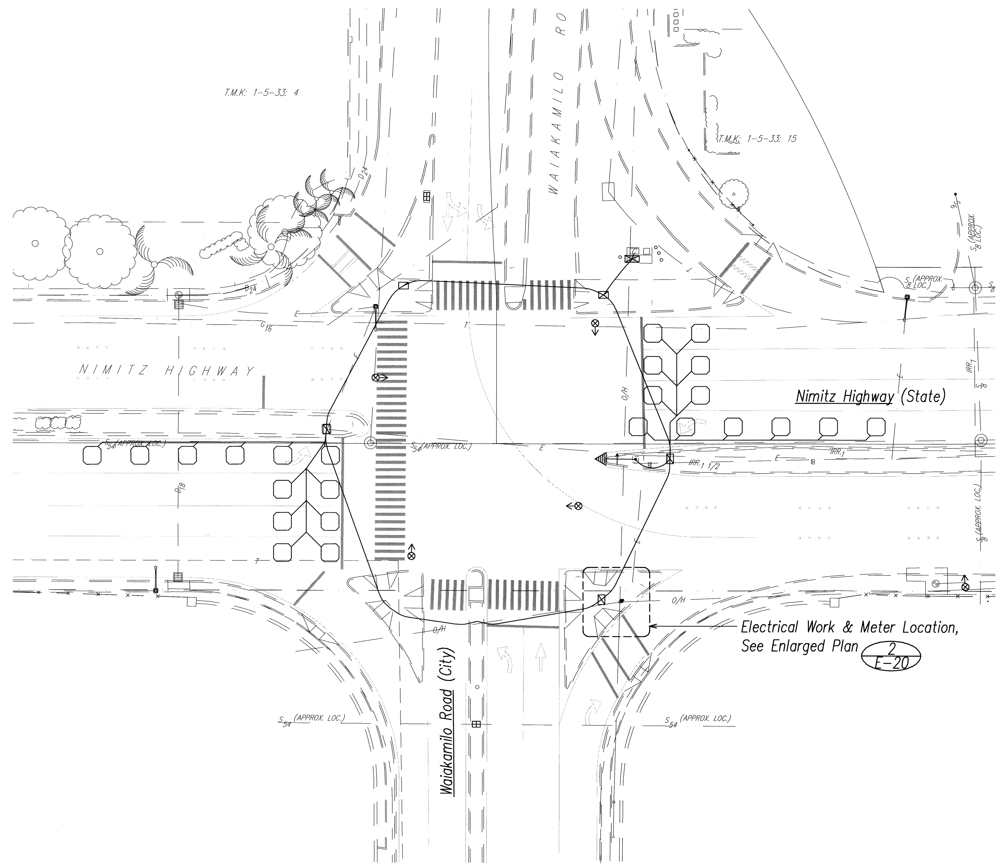
1 Nimitz Hwy. / Waikamilo Road - Electrical Plan E-20 SCALE: 1"=20' NORTH
