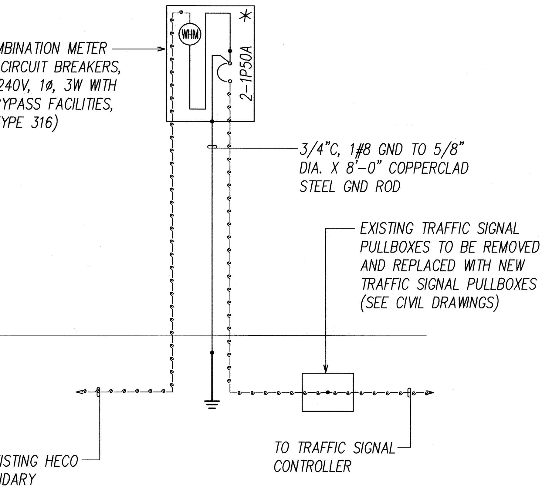
NEW ONE-LINE DIAGRAM
