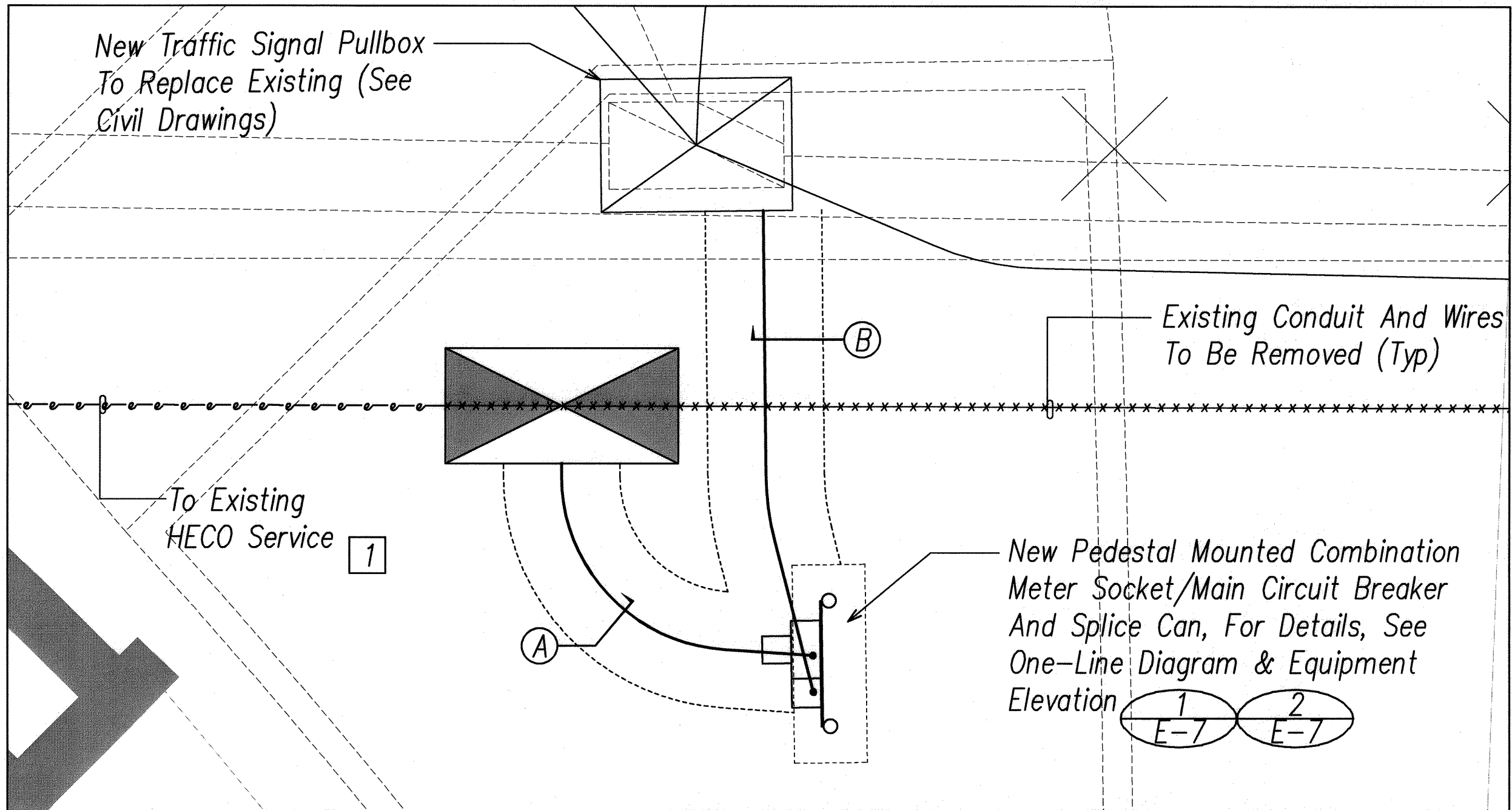
2 E-6 New Electrical Meter Enlarged Plan SCALE: 1"=2'
