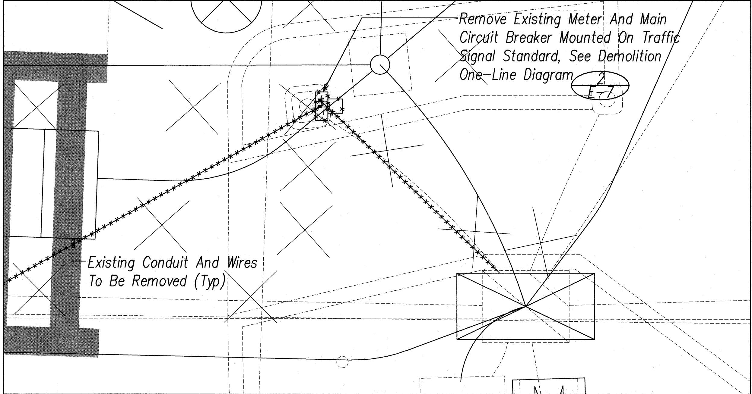
3 E-6 Existing Electrical Meter Enlarged Plan SCALE: 1"=2'
