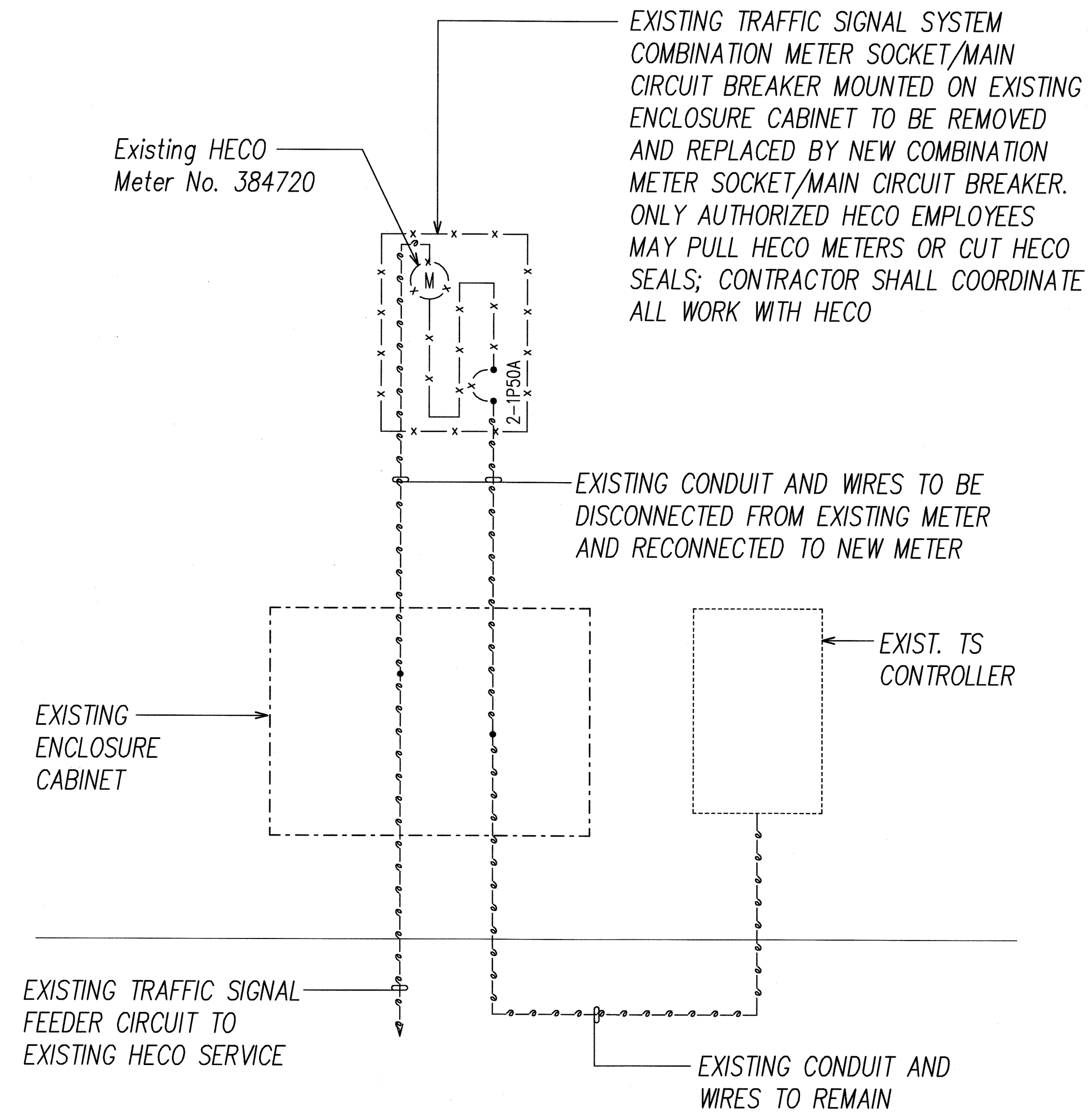
DEMOLITION ONE-LINE DIAGRAM
