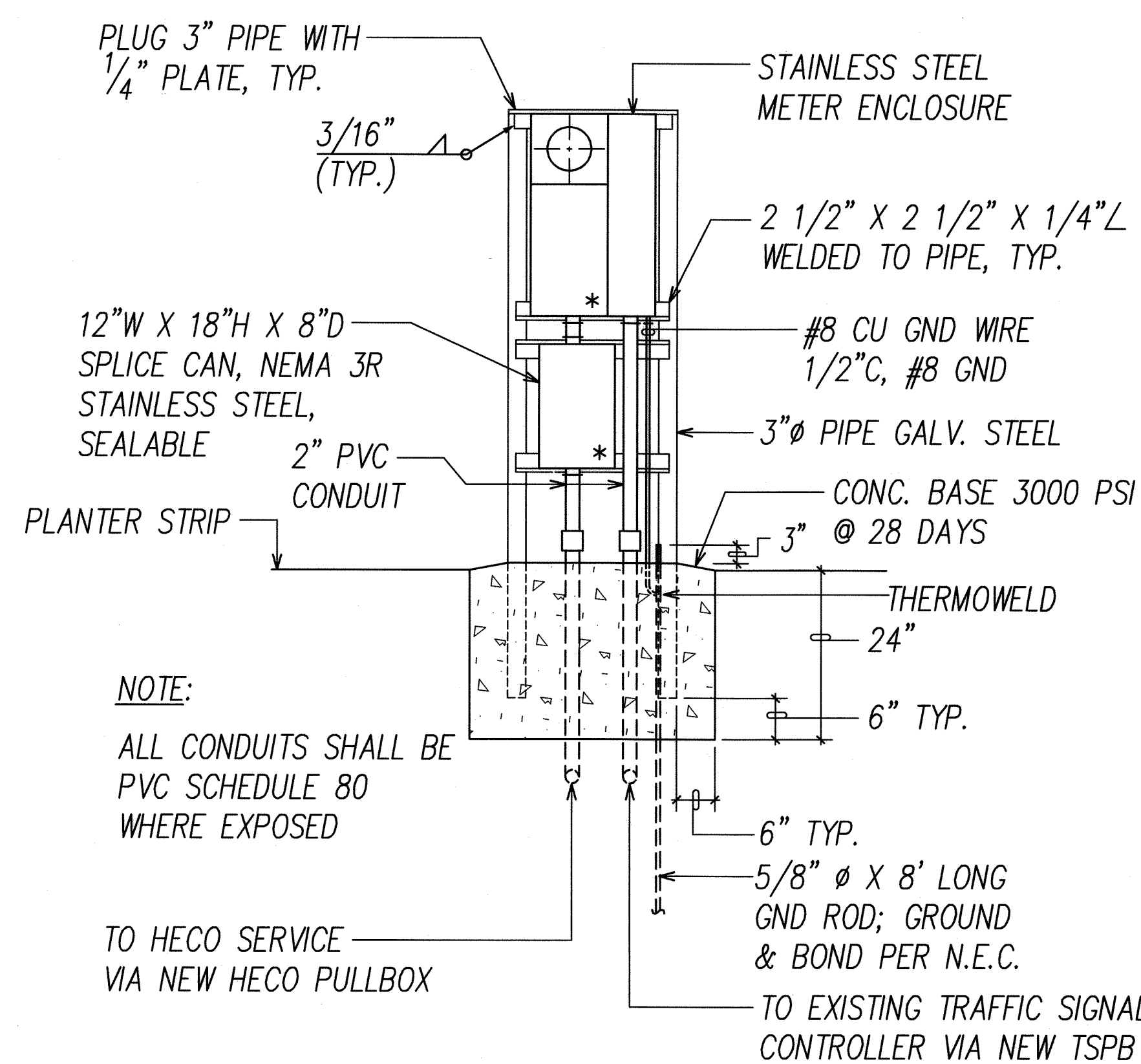
FRONT ELEVATION
