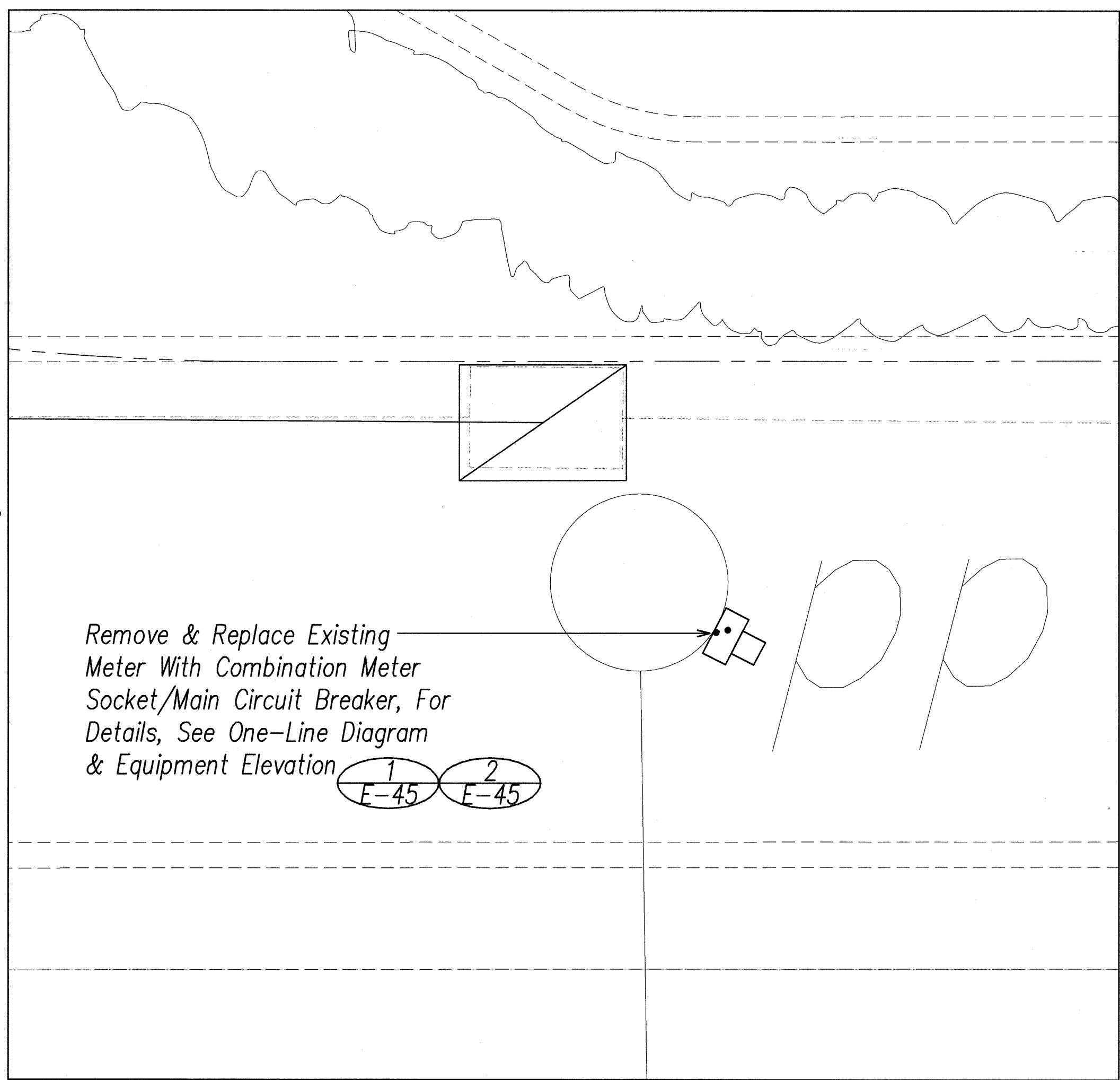
2 E-44 New Electrical Meter Enlarged Plan SCALE: 1"=2'
