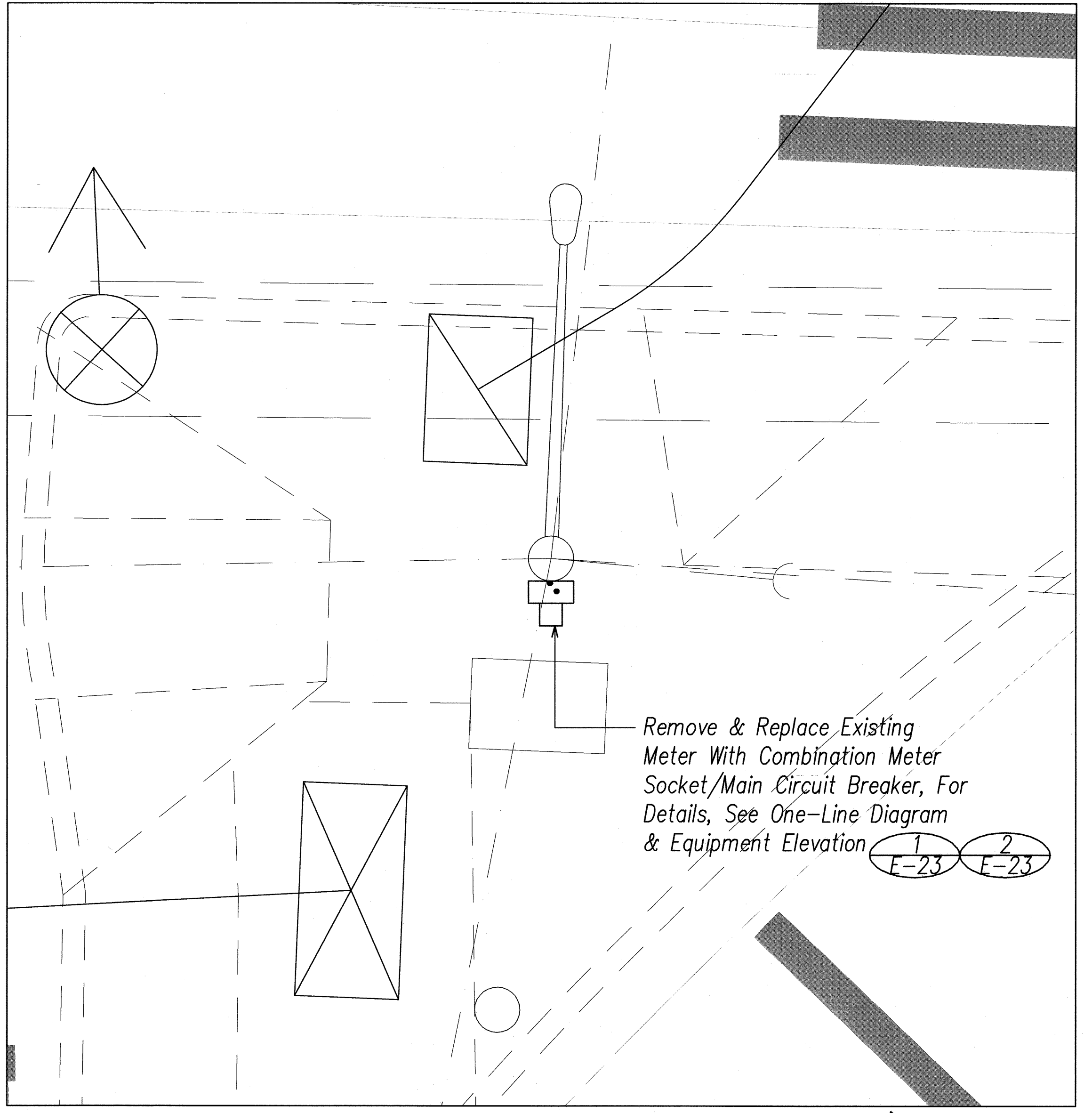
2 E-22 New Electrical Meter Enlarged Plan SCALE: 1"=2'
