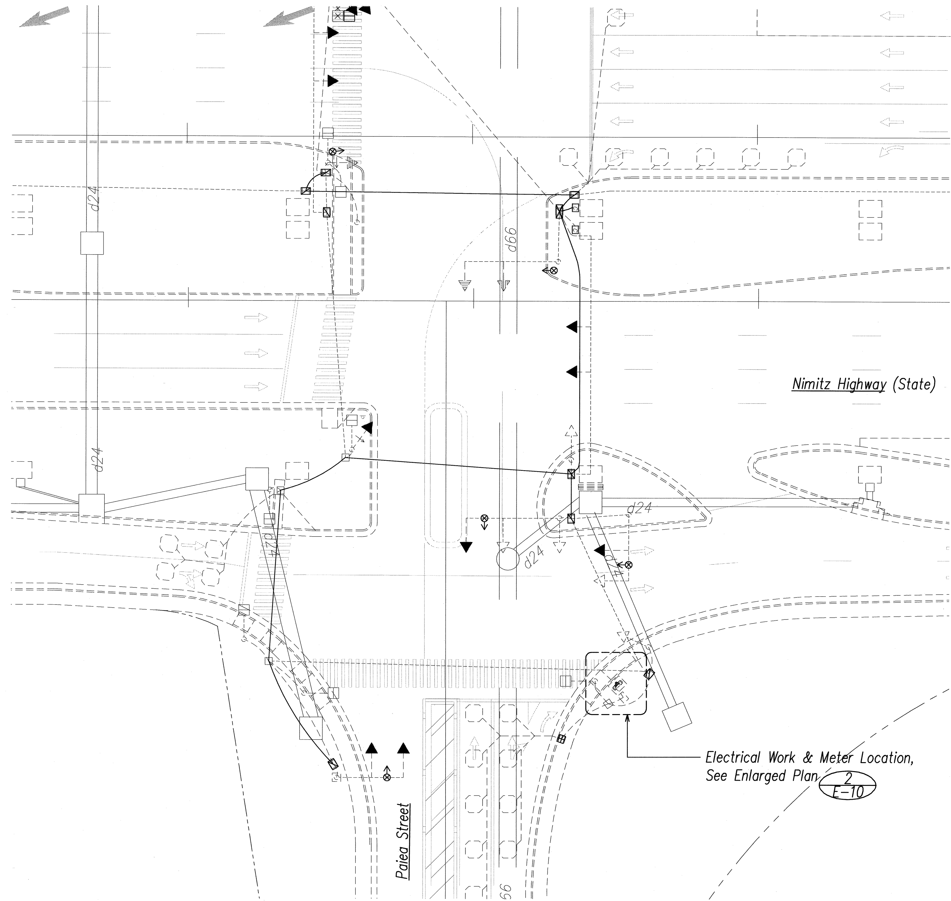
1 Nimitz Hwy. / Paiea Street - Electrical Plan E-10 SCALE: 1"=20'
