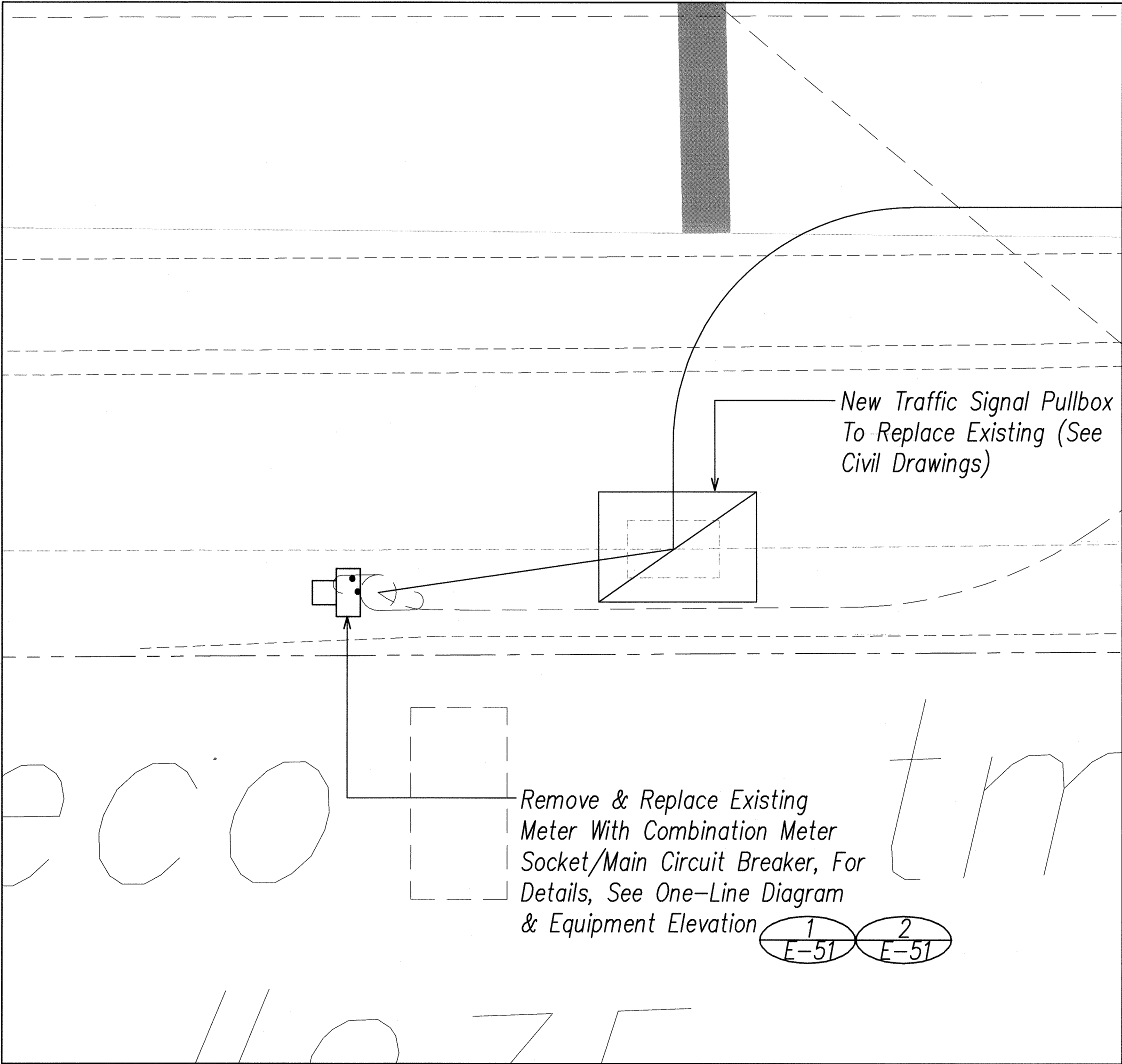
2 New Electrical Meter Enlarged Plan E-50 SCALE: 1"=2' NORTH
