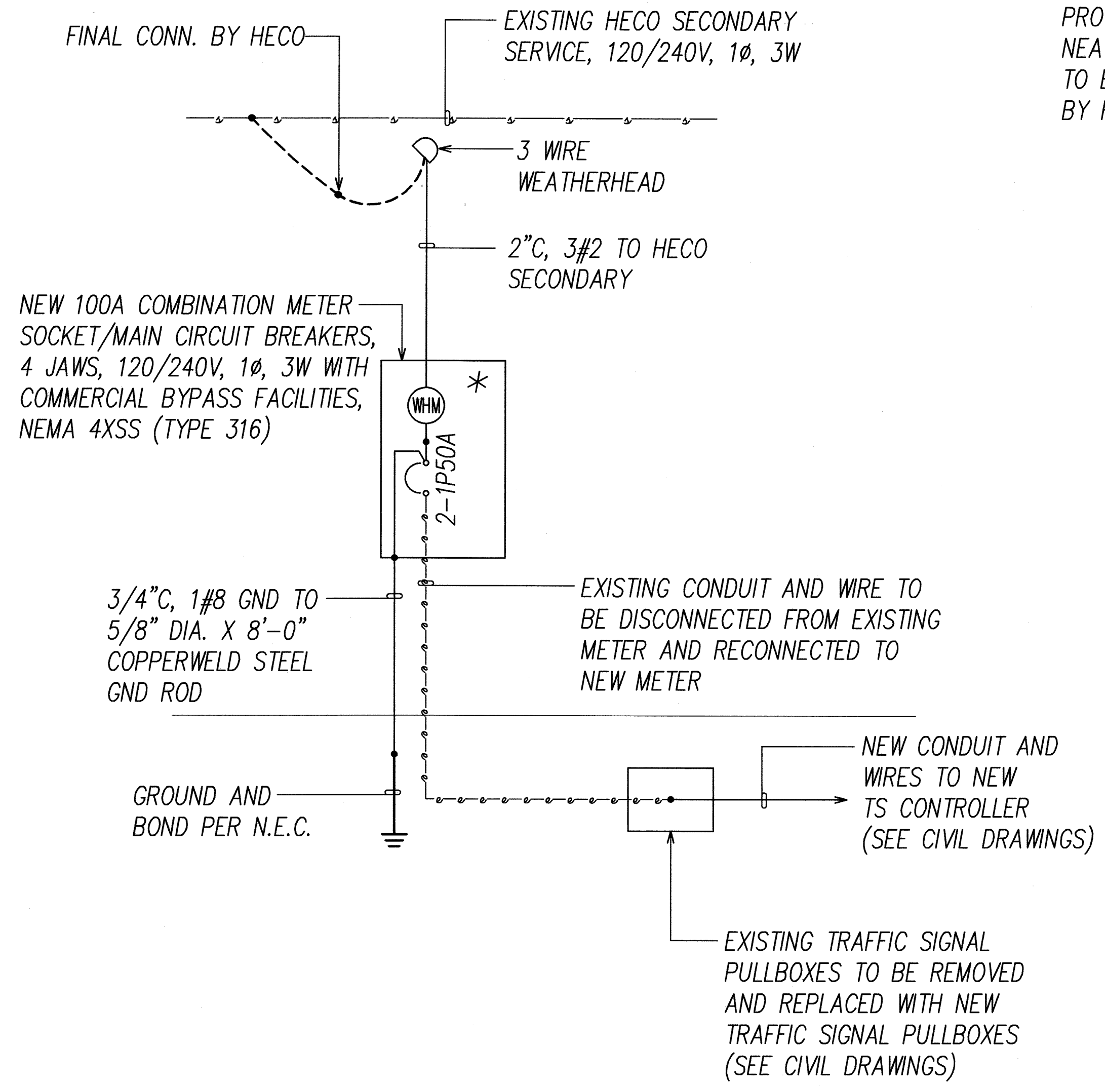
NEW ONE-LINE DIAGRAM
