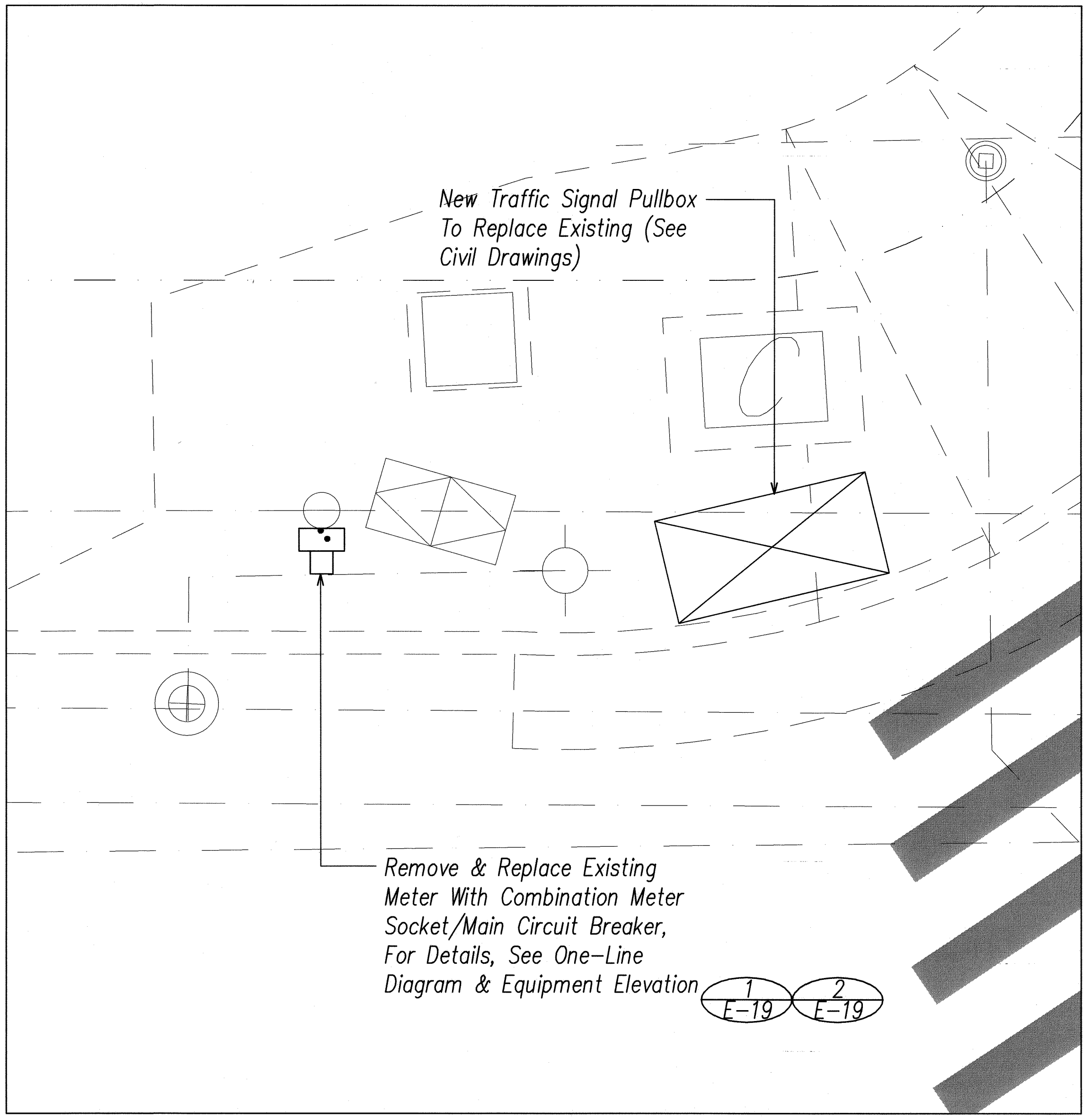
2 New Electrical Meter Enlarged Plan SCALE: 1"=5'
