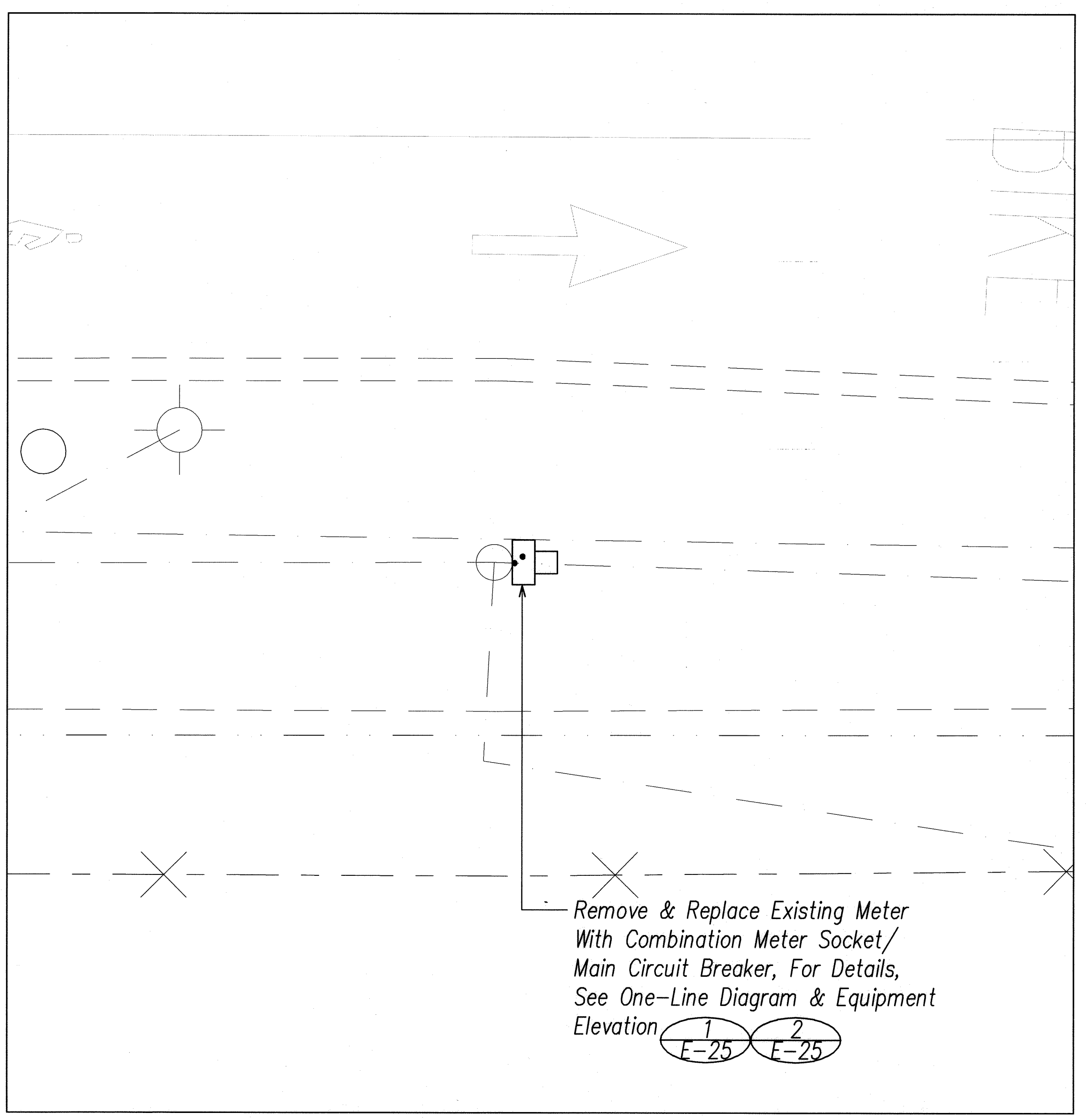
2 E-24 New Electrical Meter Enlarged Plan SCALE: 1"=2'
