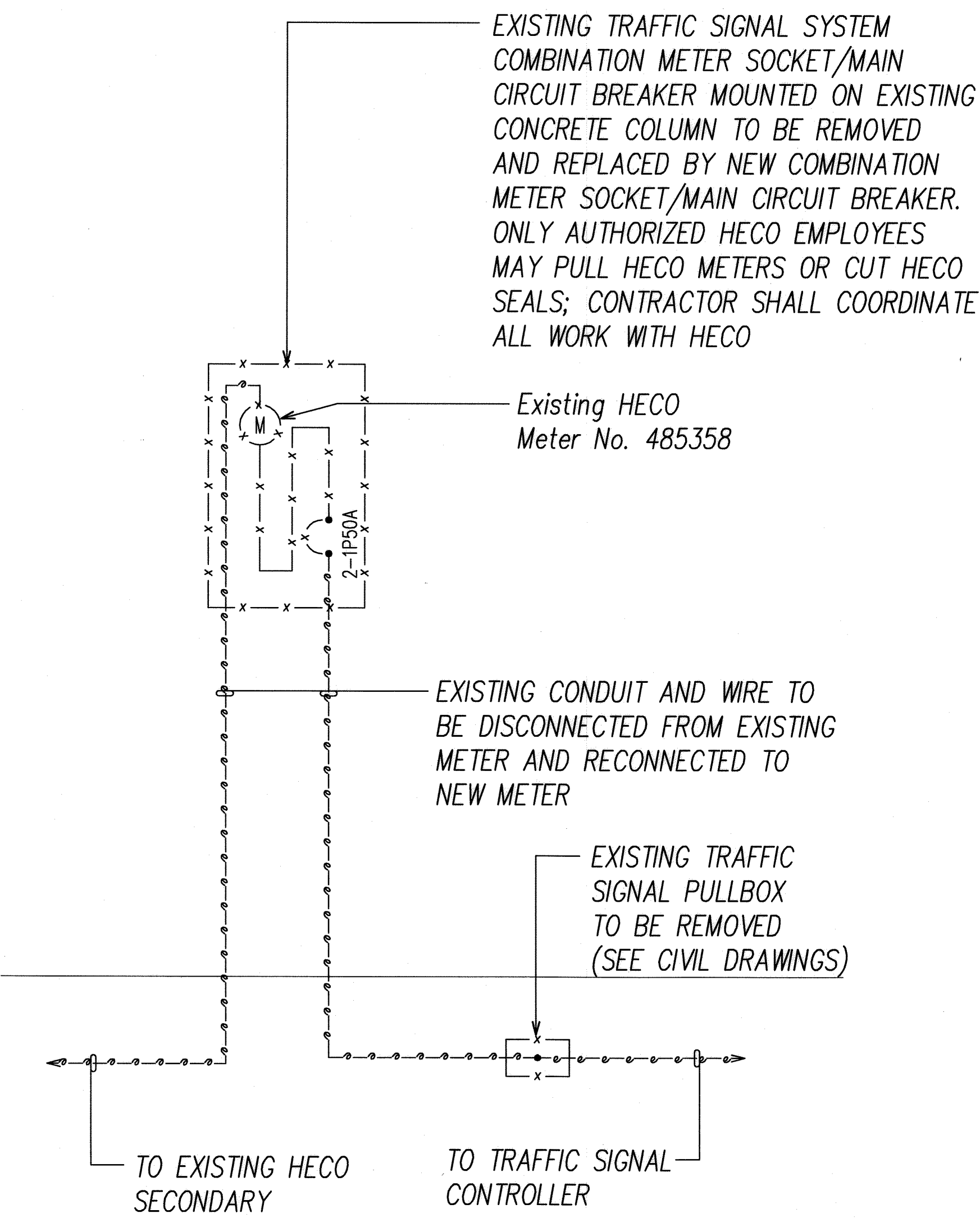
DEMOLITION ONE-LINE DIAGRAM
