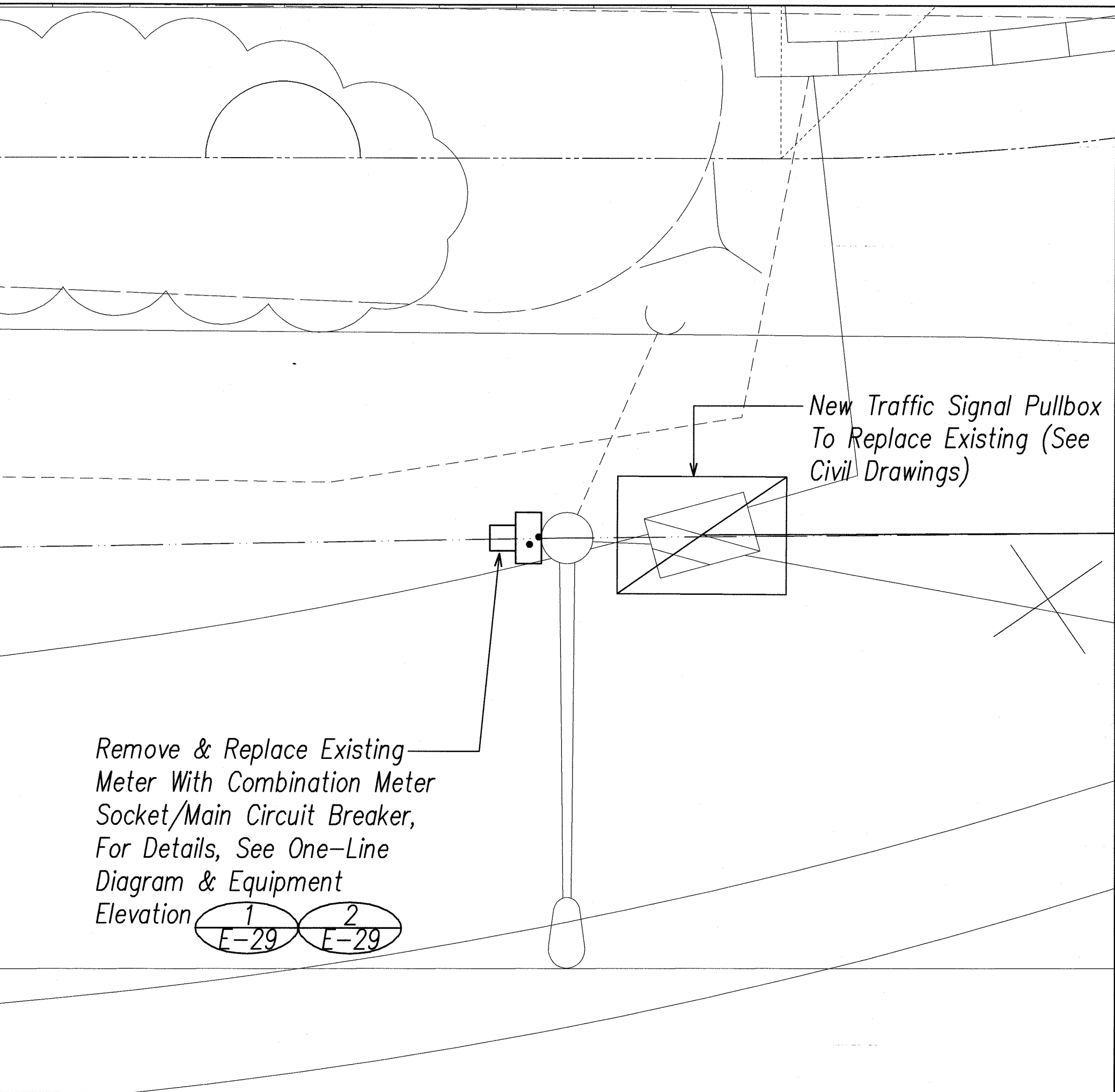
2 New Electrical Meter Enlarged Plan E-28 SCALE: 1"=2'
