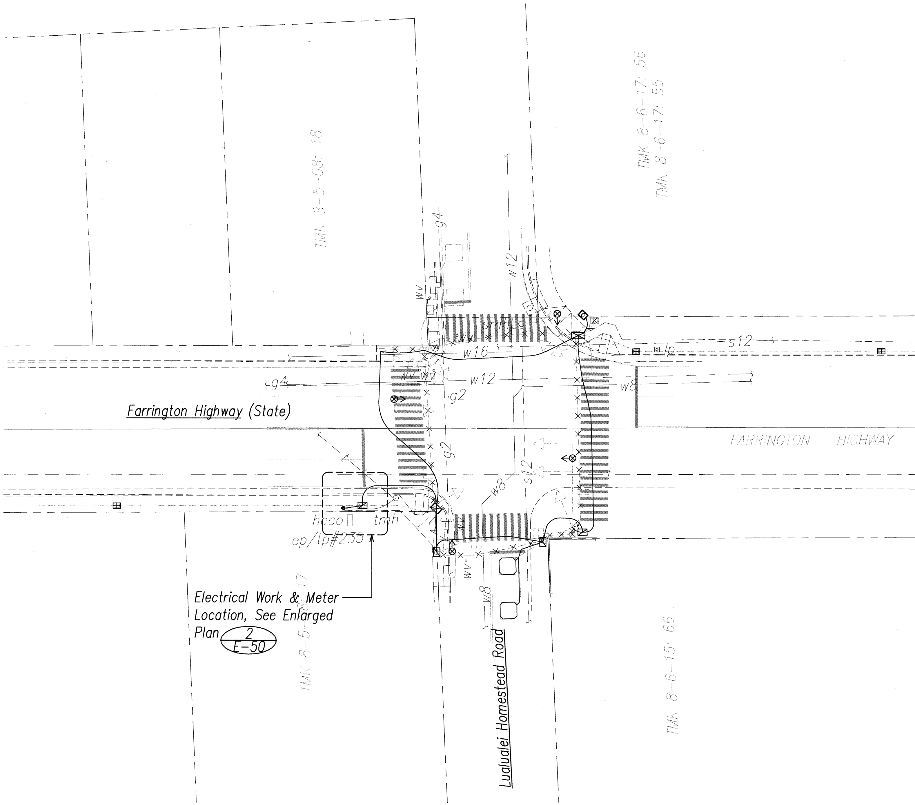
1 Farrington Hwy. / Lualualei Homestead Road - Electrical Plan E-50 SCALE: 1"=20' NORTH
