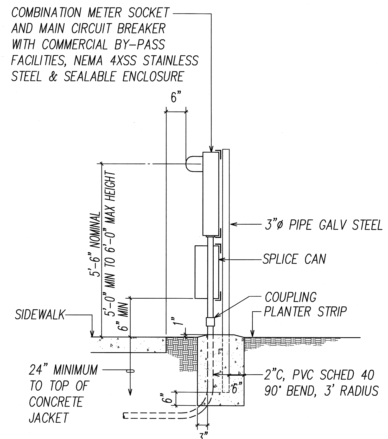
FRONT ELEVATION
