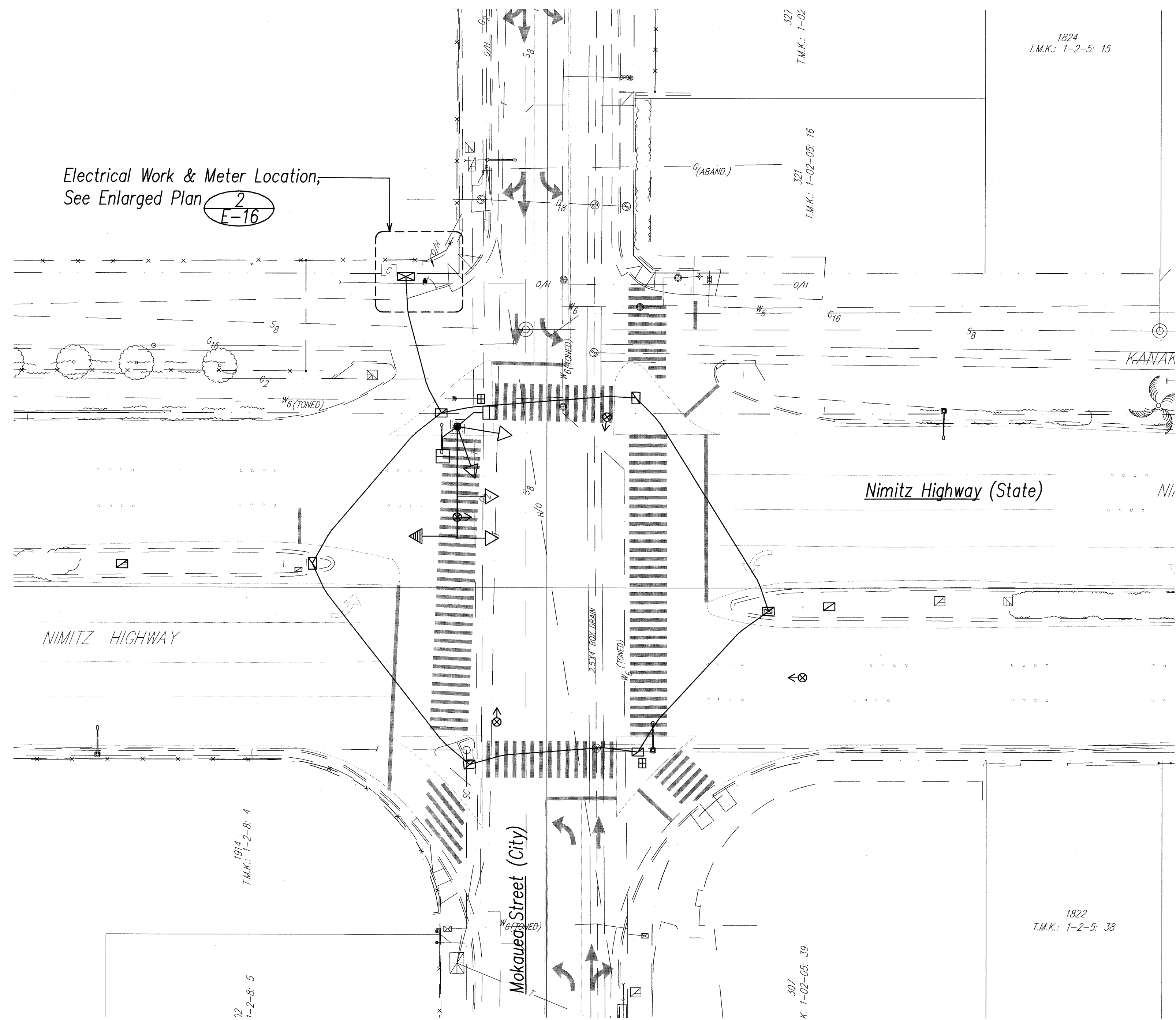
1 Nimitz Hwy. / Mokauea Street - Electrical Plan E-16 SCALE: 1"=20'
