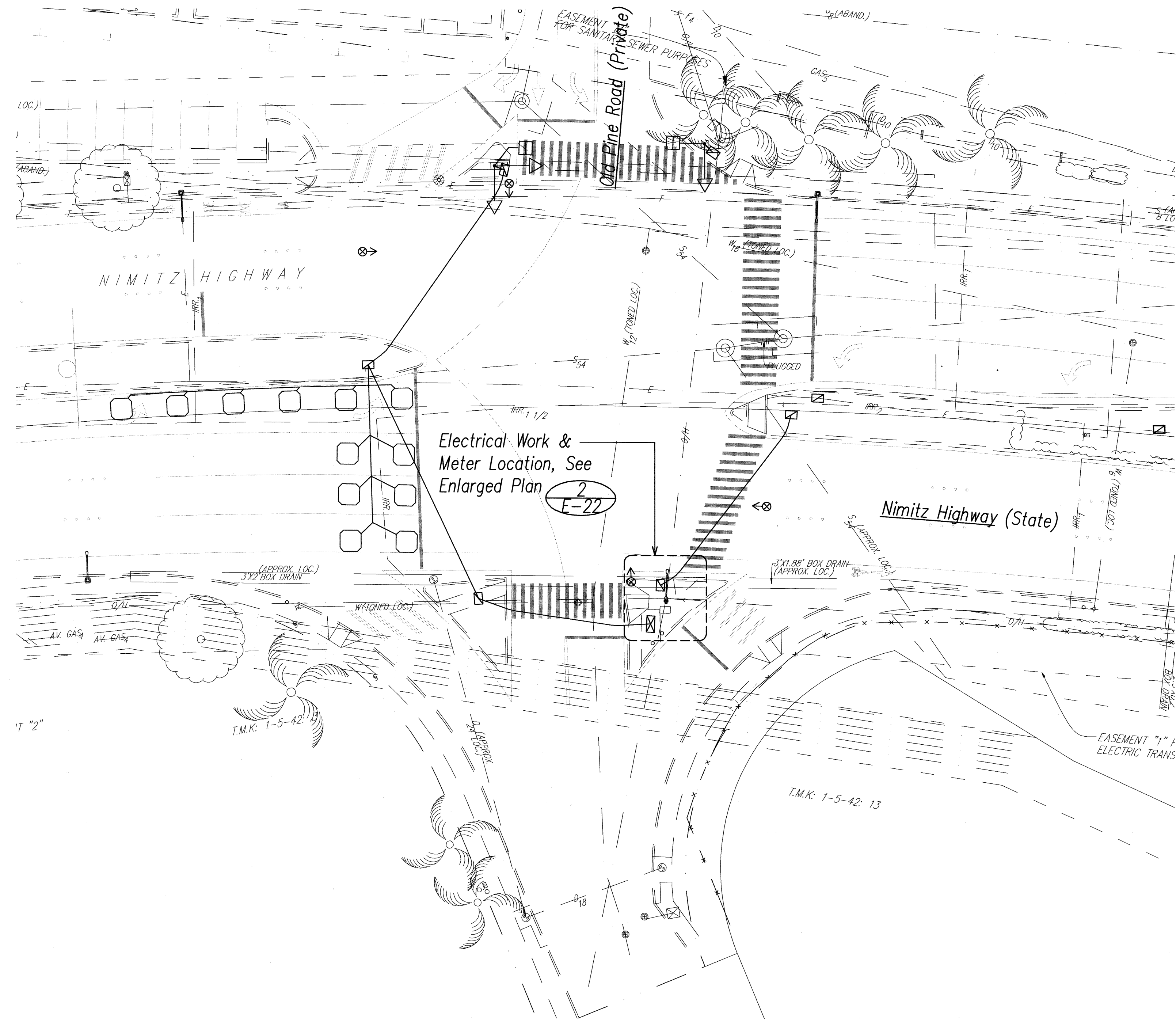
1 E-22 Nimitz Hwy. / Old Pine Road - Electrical Plan SCALE: 1"=20'
