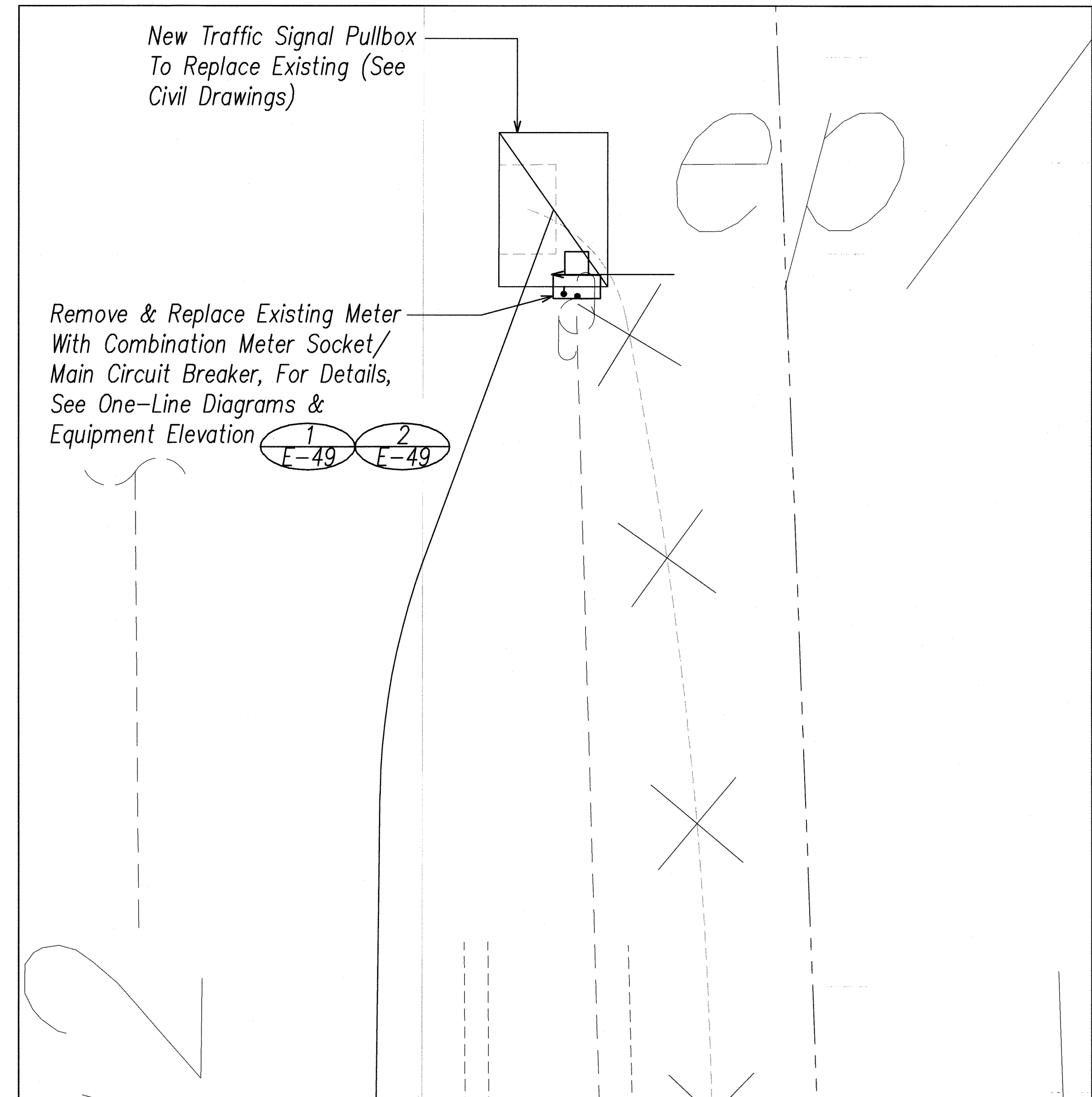
2 New Electrical Meter Enlarged Plan E-48 SCALE: 1"=2'
