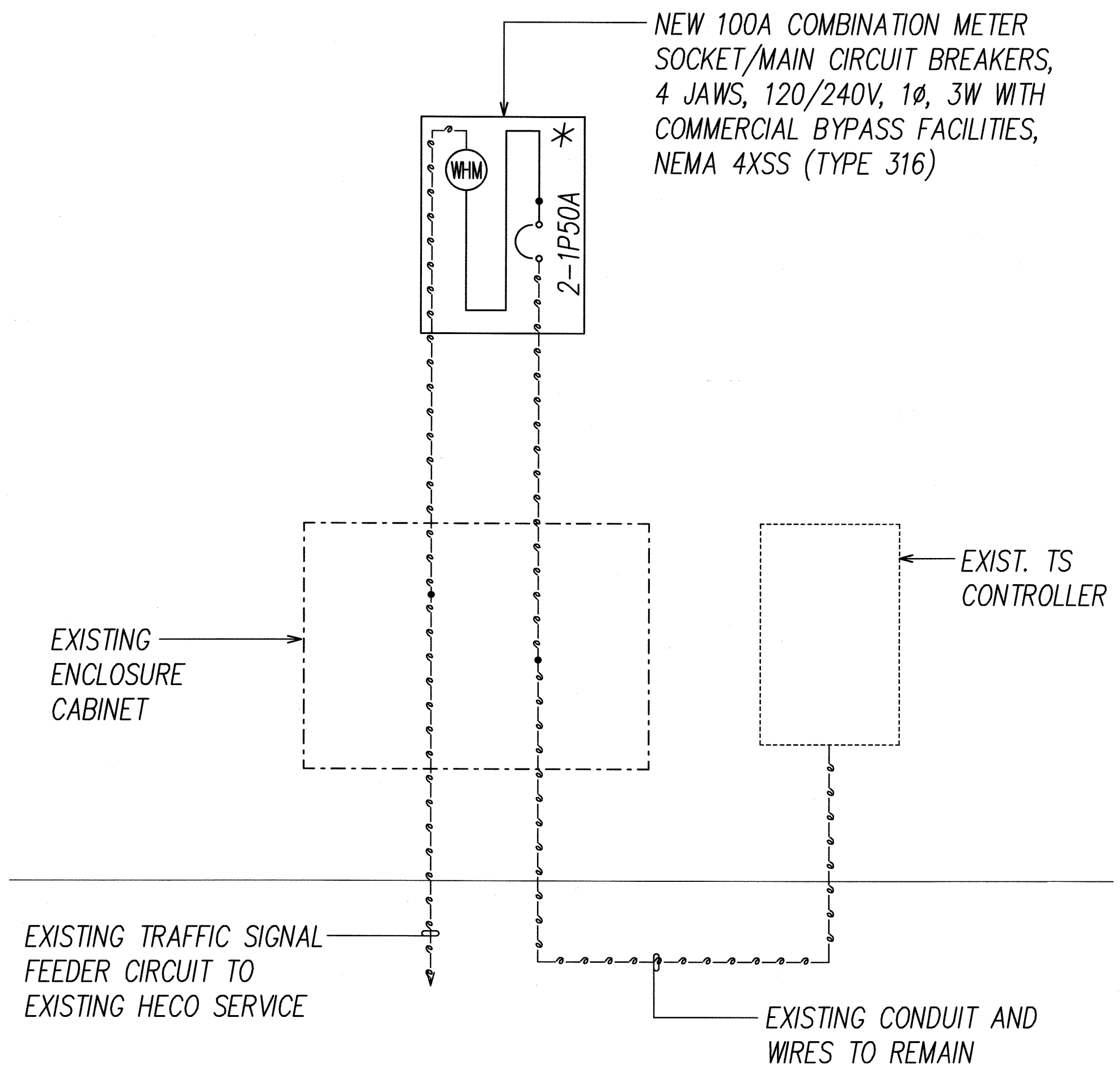
NEW ONE-LINE DIAGRAM
