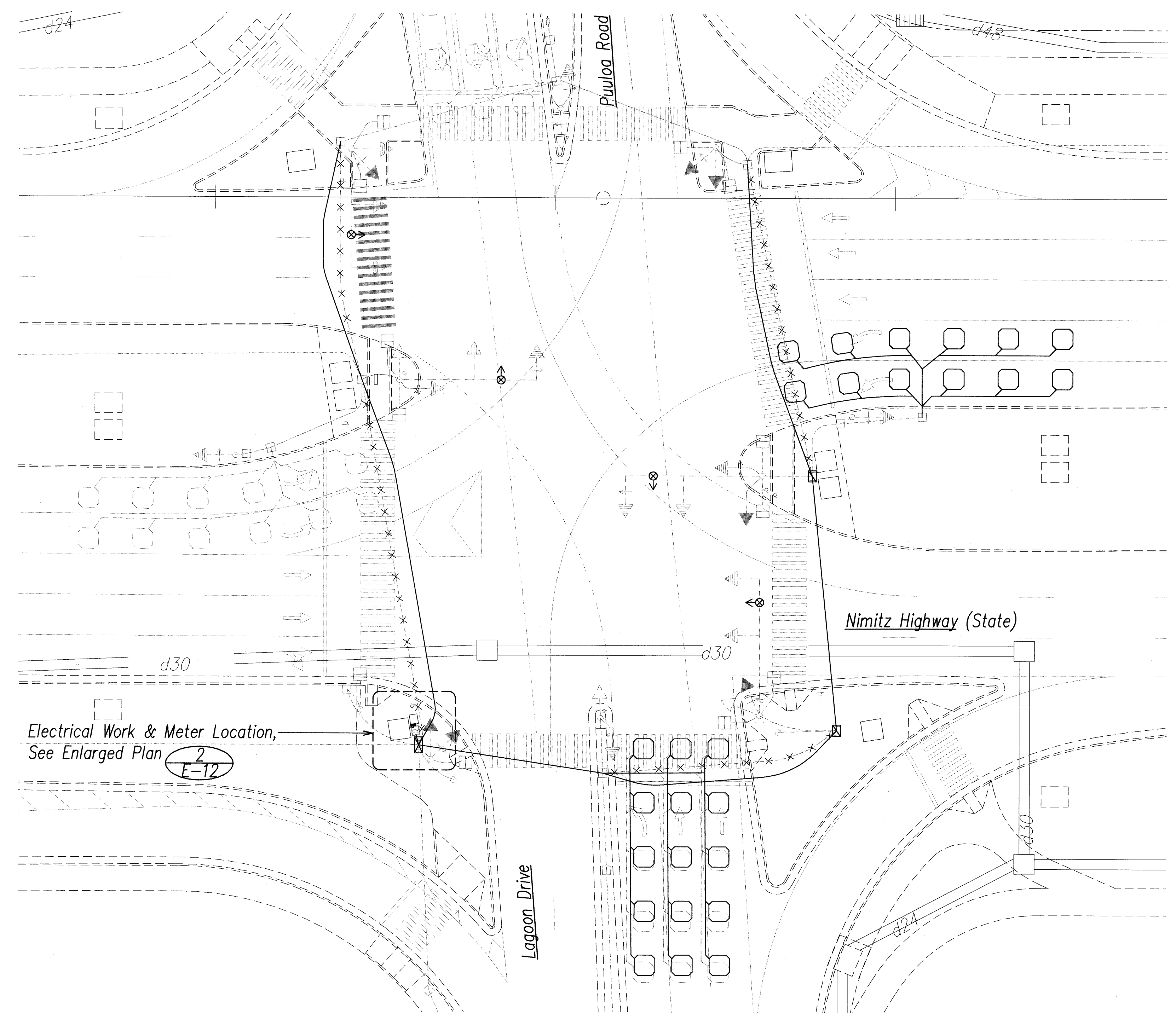
1 E-12 Nimitz Hwy. / Puuloa Road & Lagoon Drive - Electrical Plan SCALE: 1"=20'
