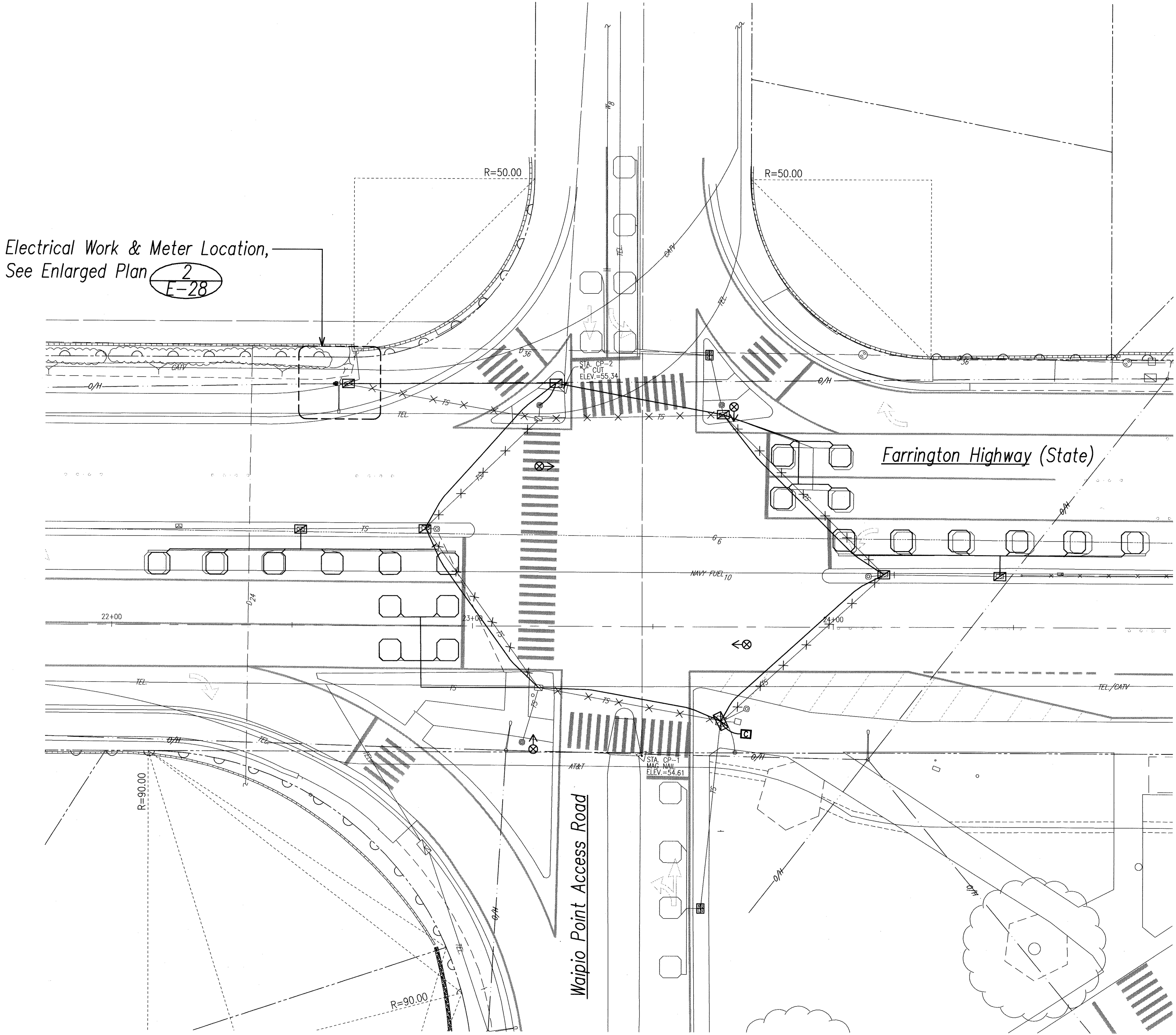
1 Farrington Hwy. / Waipio Point Access Road - Electrical Plan E-28 SCALE: 1"=20'
