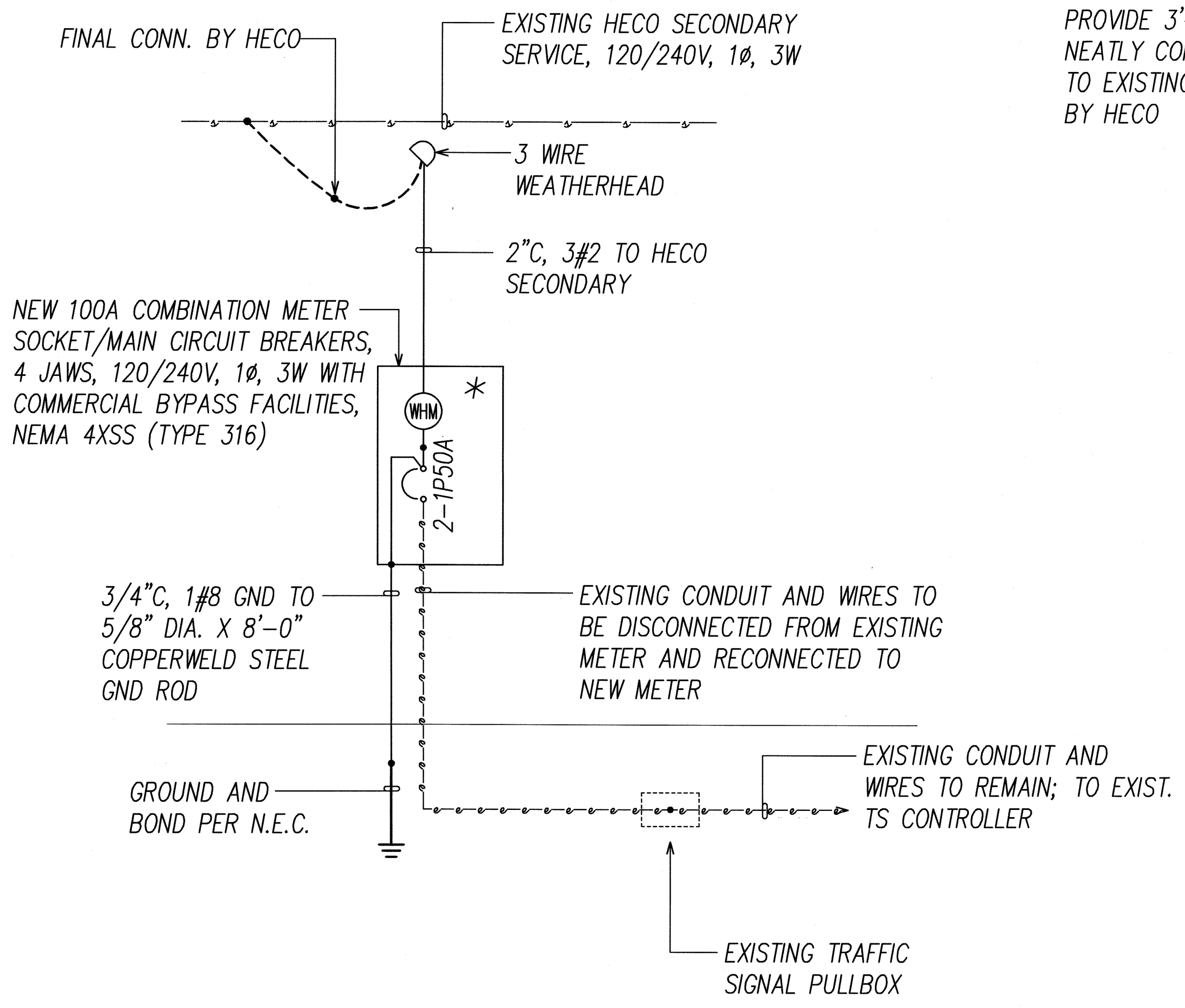
NEW ONE-LINE DIAGRAM
