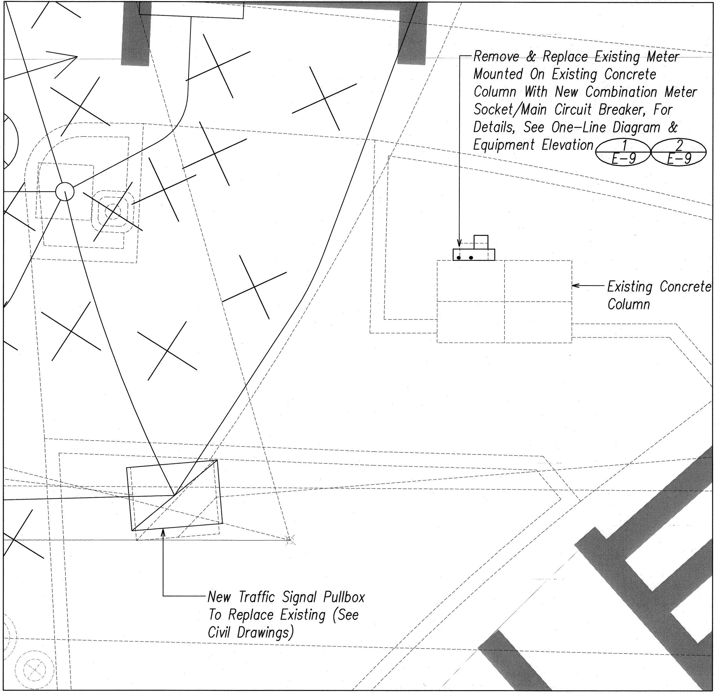
2 E-8 New Electrical Meter Enlarged Plan SCALE: 1"=2'
