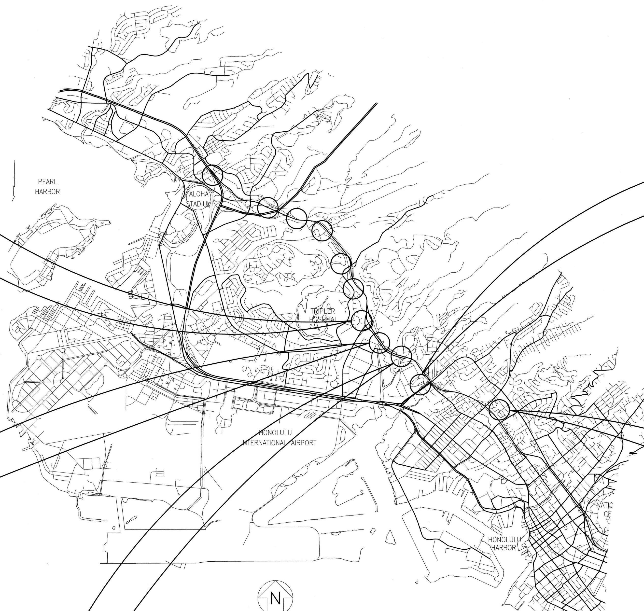
GENERAL PLAN NOT TO SCALE
