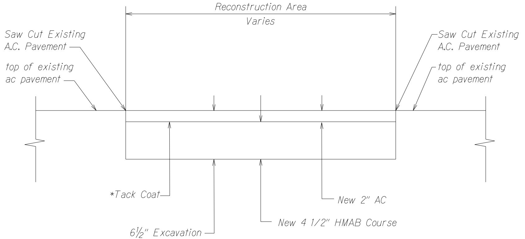
TYPICAL RECONSTRUCTION AREA Not to Scale
