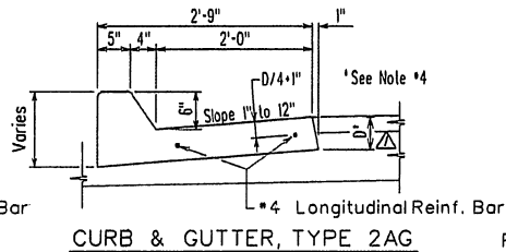
CAST-IN-PLACE CURB & GUTTER CAST-IN-PLACE GUTTER CONSTRUCTION AND CONTRACTION JOINT DETAIL
