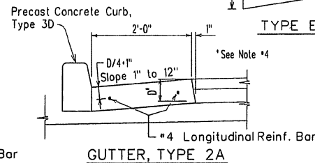
CAST-IN-PLACE CONCRETE CURBS AND/OR GUTTERS
