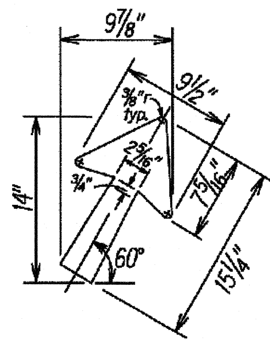
Type "A" Diagonal Arrow Detail
