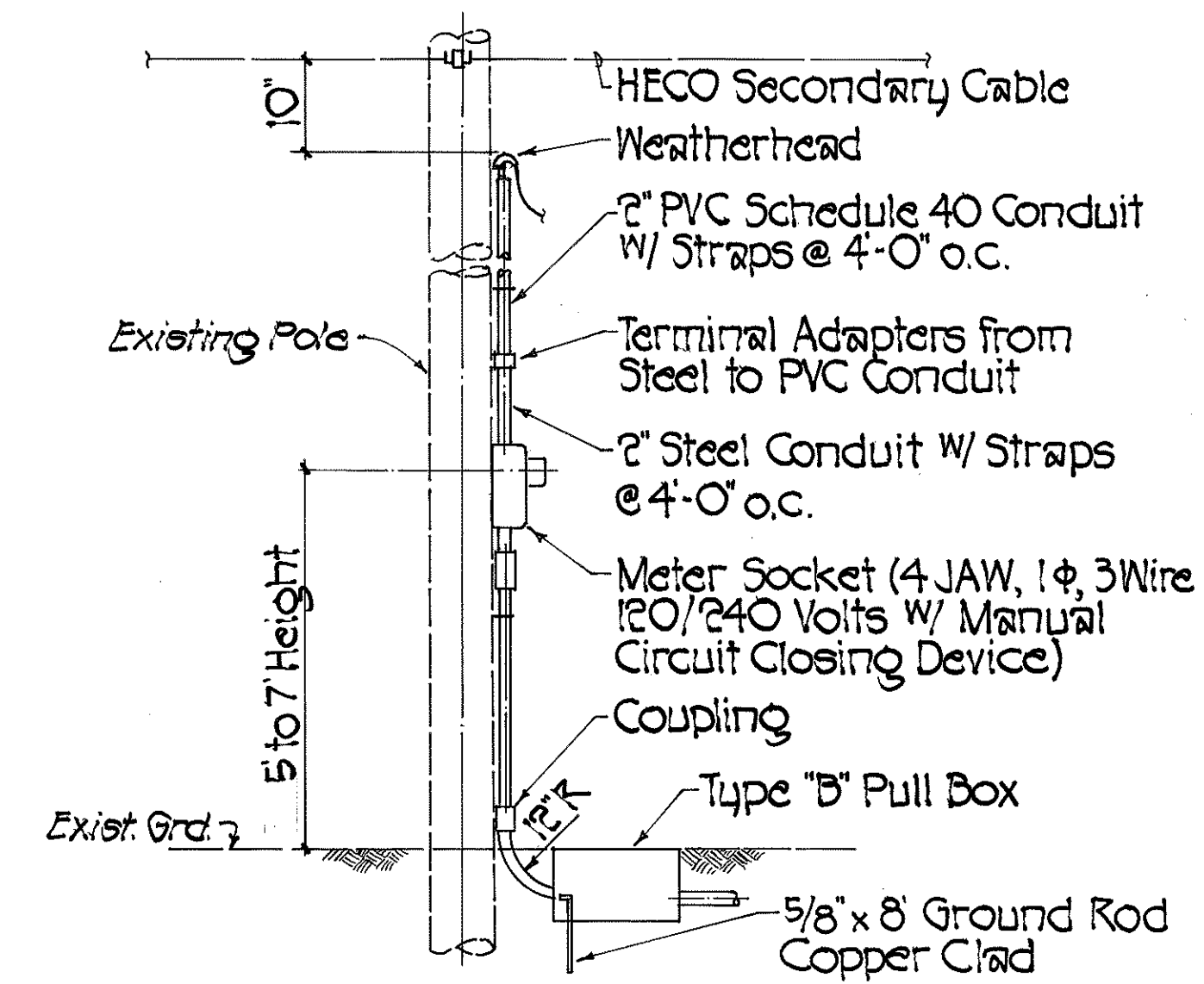
SERVICE POLE DETAIL Not to Scale
