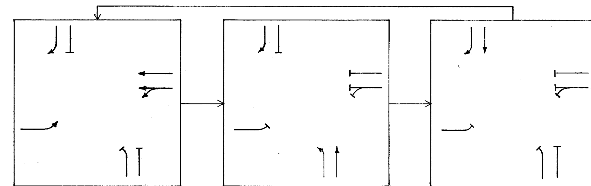
EXISTING CONTROLLER PHASE DIAGRAM EXISTING CONTROLLER: AUTOMATIC SIGNAL 11/4M 3 PHASE
