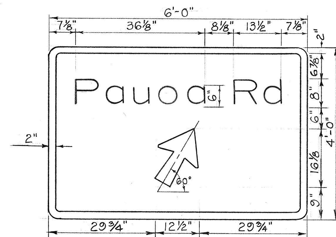
NEW SIGN D-1
