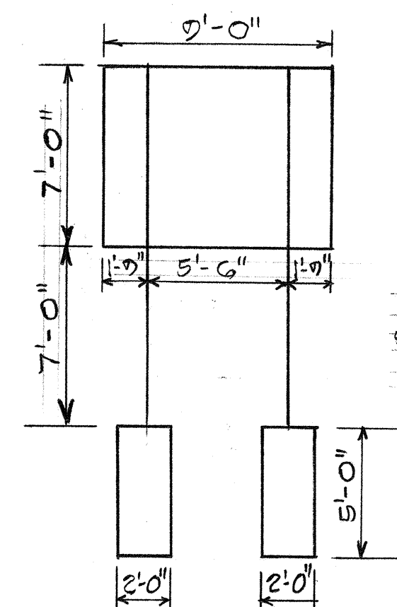
SIGN D-7 SOUTHEAST RAMP - AIEA INTERCHANGE
