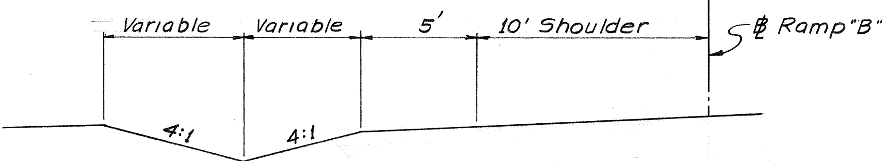
SECTION B-B No Scale
