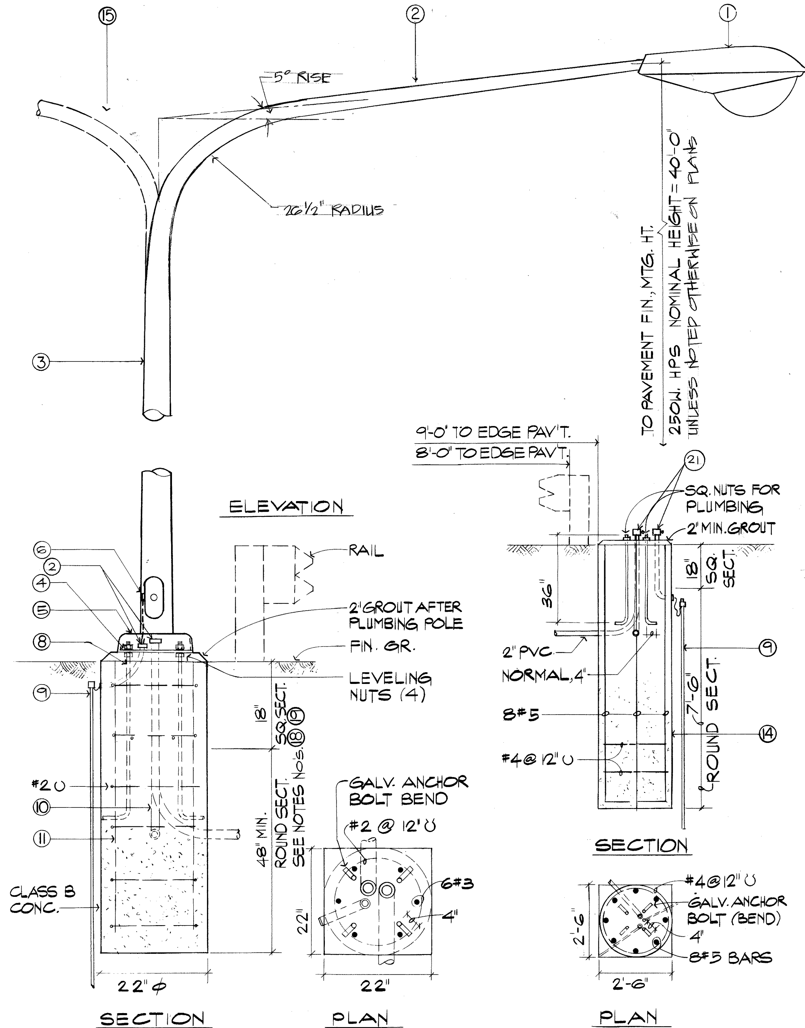
A HIGHWAY LIGHTING STANDARD DETAIL E-22
