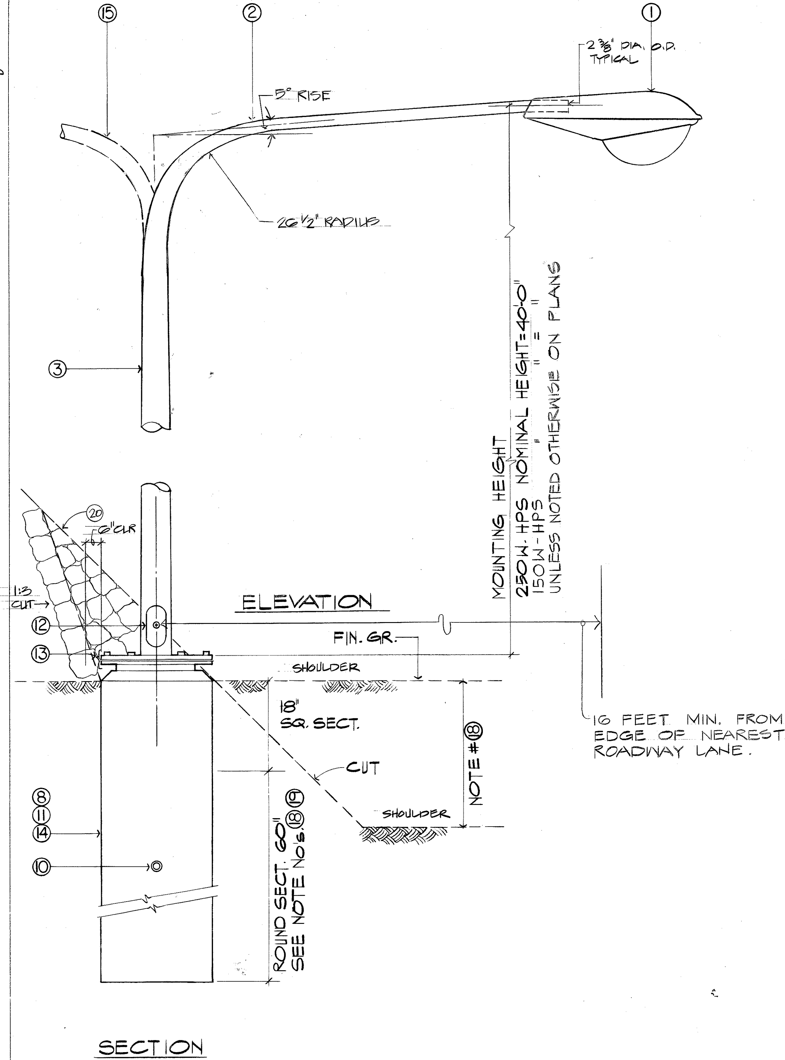
B HIGHWAY LIGHTING STANDARD DETAIL E-22
