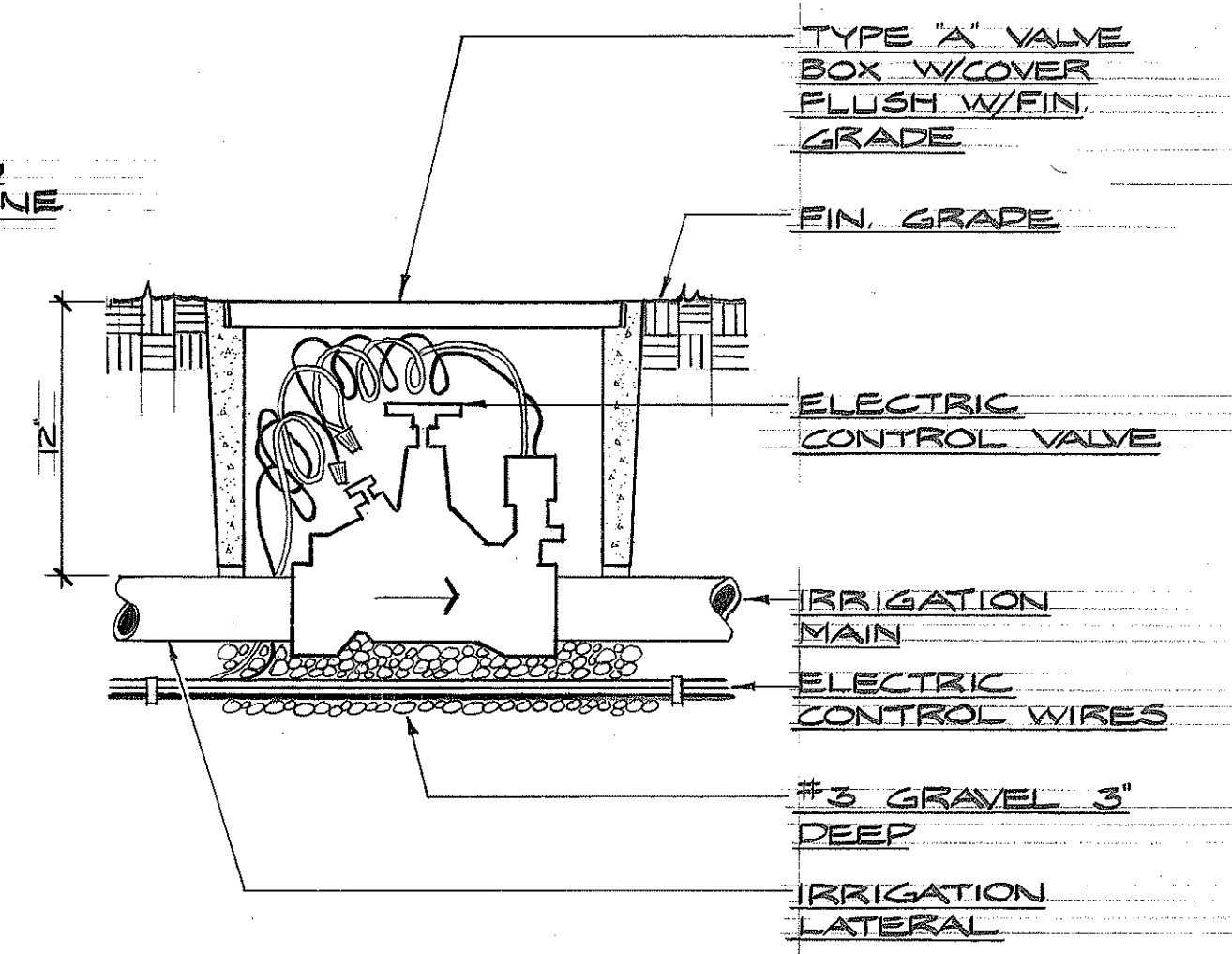
ELECTRIC CONTROL VALVE NO SCALE
