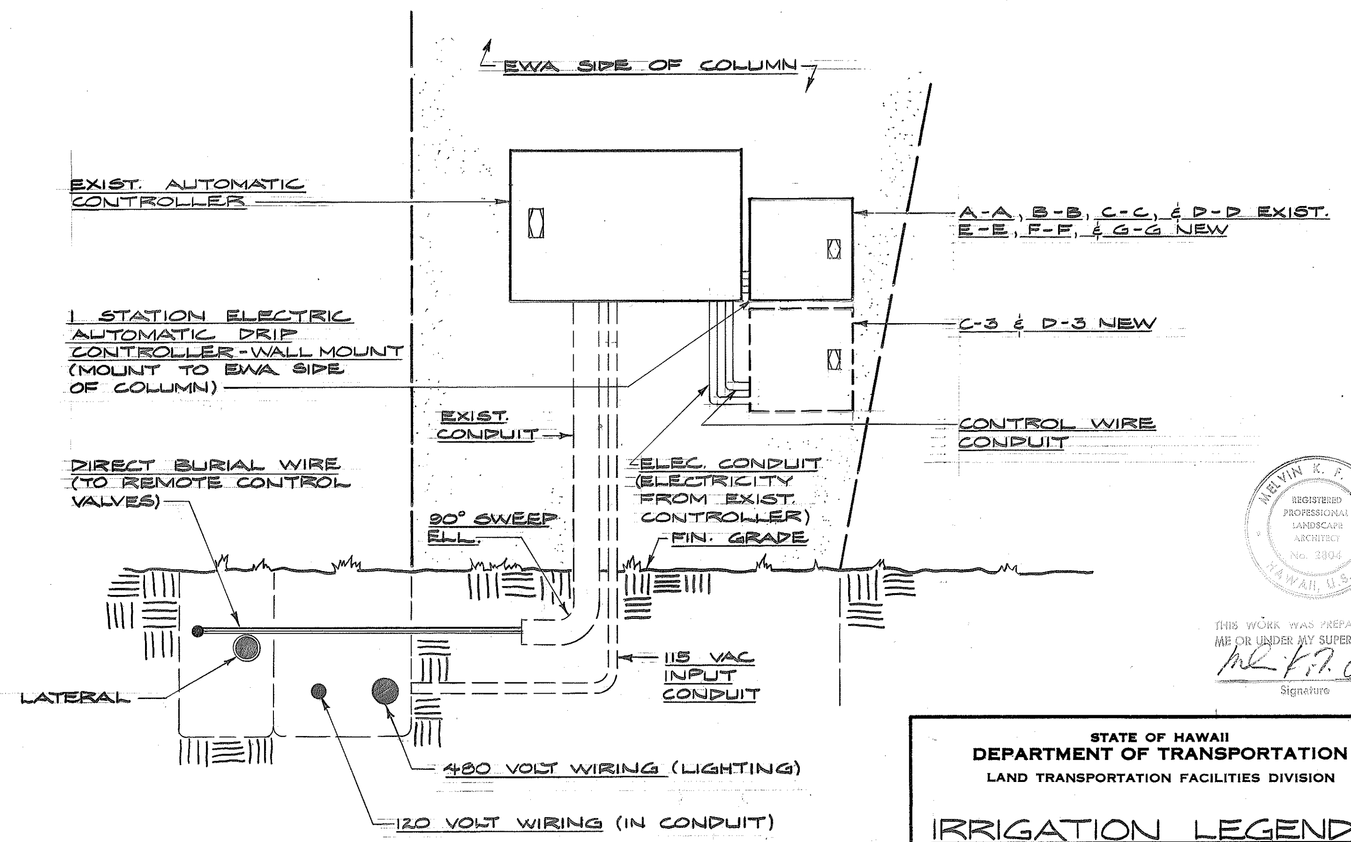
CONTROLLER & TRENCHING DETAIL NO SCALE
