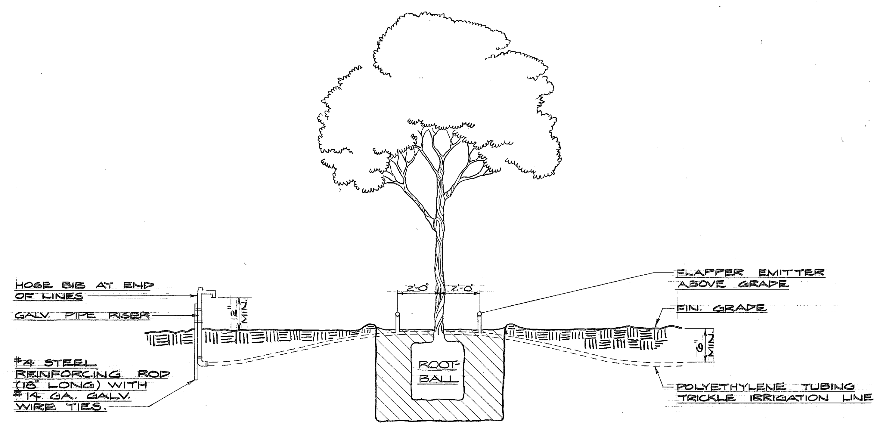
TRICKLE IRRIGATION SYSTEM DETAIL NO SCALE
