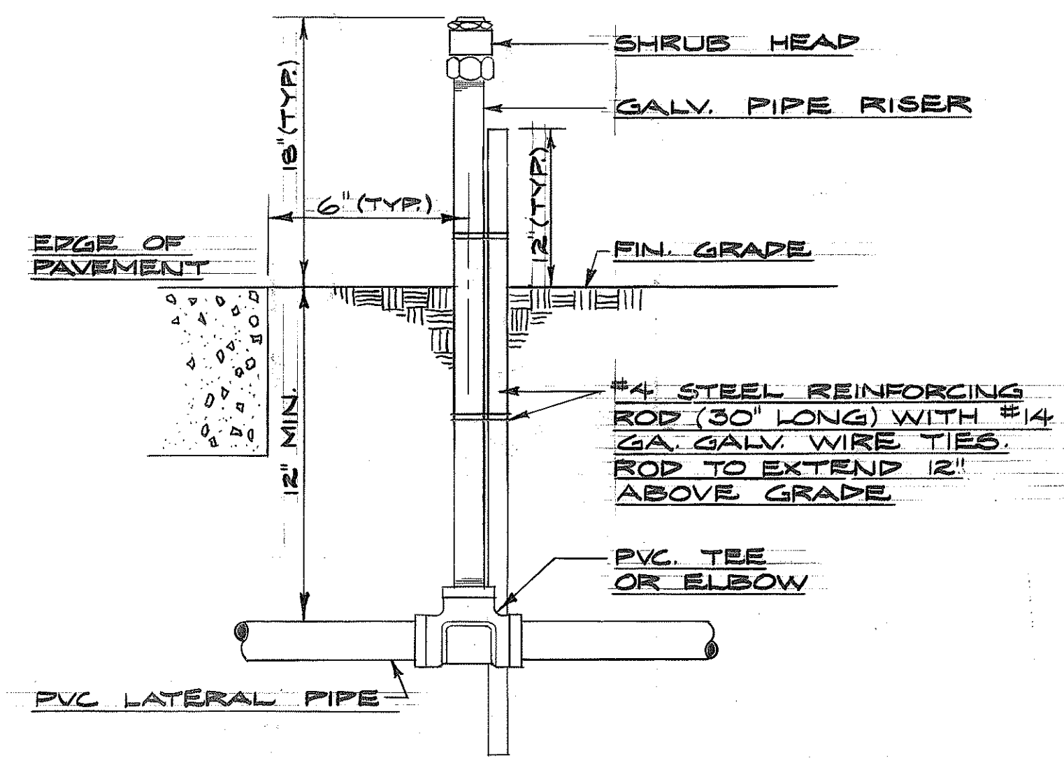
TYPICAL SHRUB HEAD DETAIL NO SCALE
