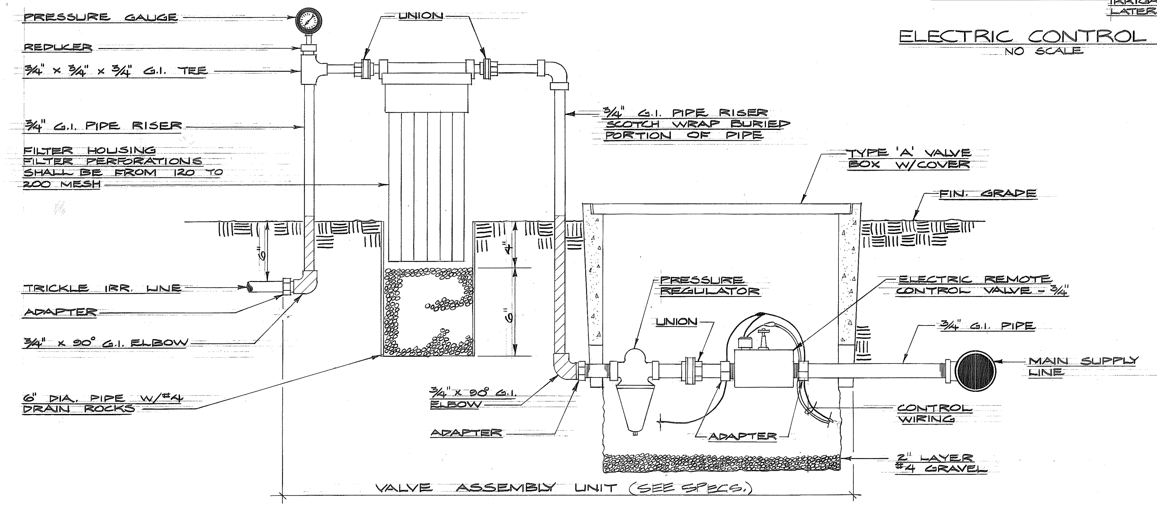
VALVE ASSEMBLY UNIT & ELECTRIC REMOTE CONTROL VALVE (TRICKLE SYSTEMS) NO SCALE
