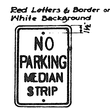
R-42-S 12" x 18"
