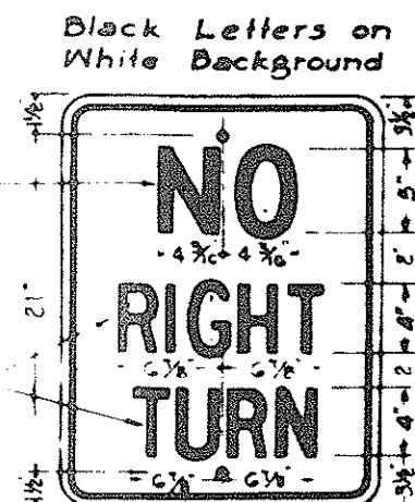
R-6 18" x 24"
