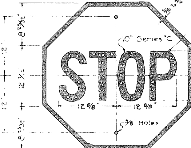
R-1 30" x 30"
