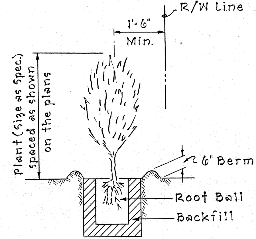
TYPICAL PLANTING DETAIL Not To Scale
