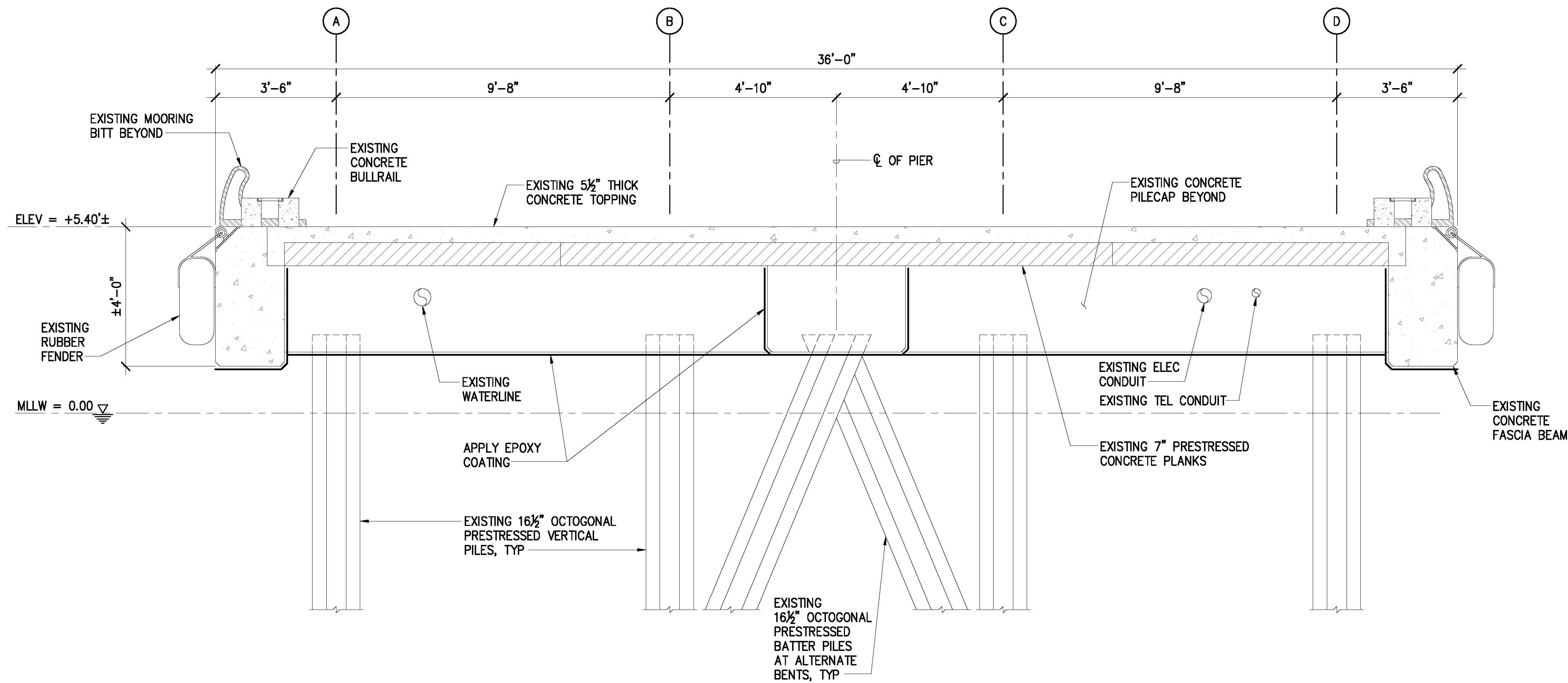
1 S-7 TYPICAL TRANSVERSE SECTION AT PIER 17 SCALE: 1/2" = 1'-0"
