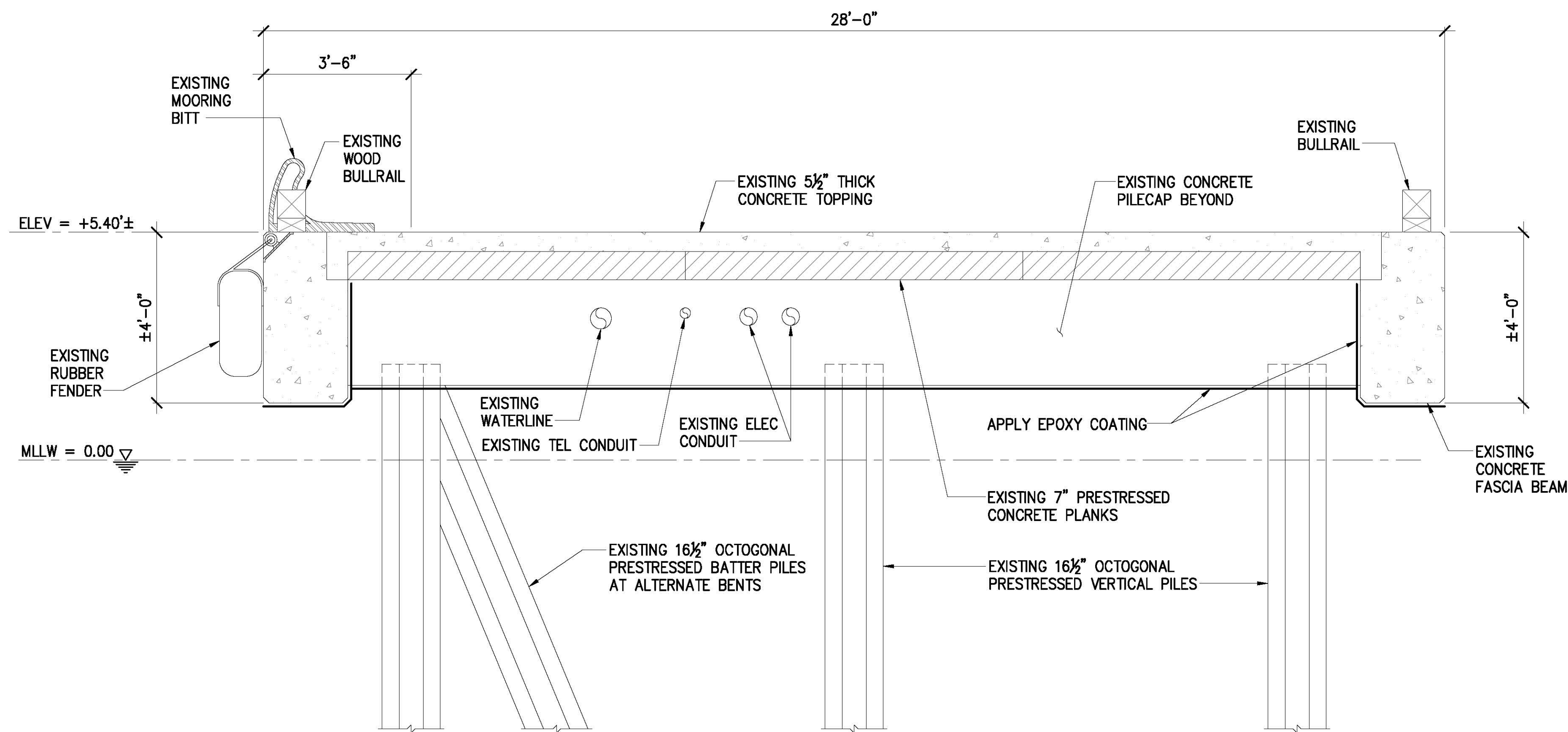
1 S-7 TYPICAL TRANSVERSE SECTION AT PIER 17 SCALE: 1/2" = 1'-0"
