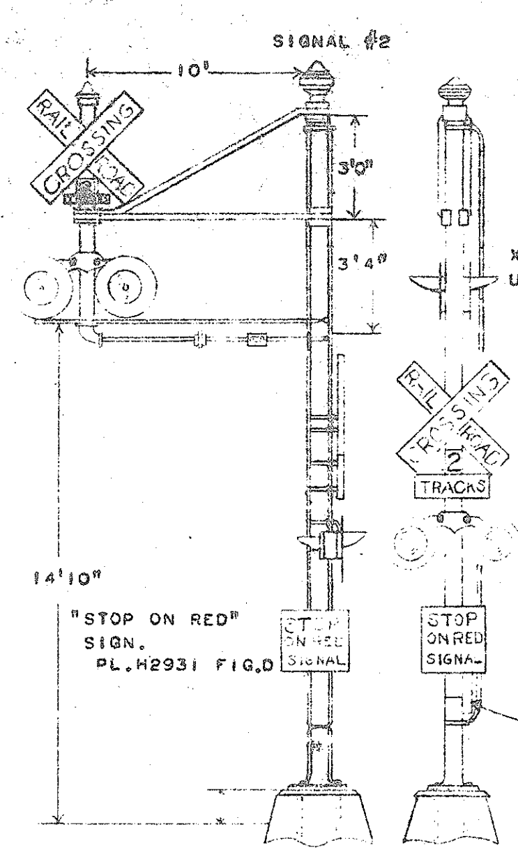
HIGHWAY CROSSING FLASHING LIGHT SIGNAL ASSEMBLY - CANTILEVER TYPE
