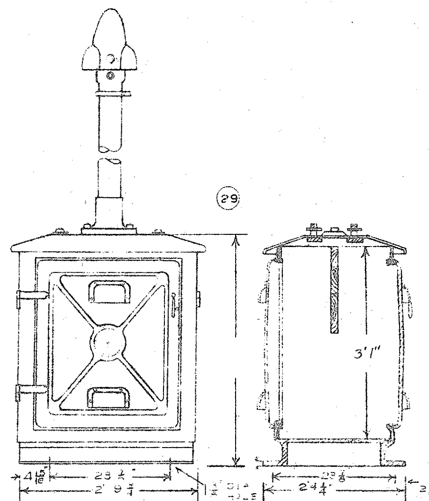
PL.E0935 FIG.A1 DOUBLE DOOR WELDED CASE WITH CABLE POST
