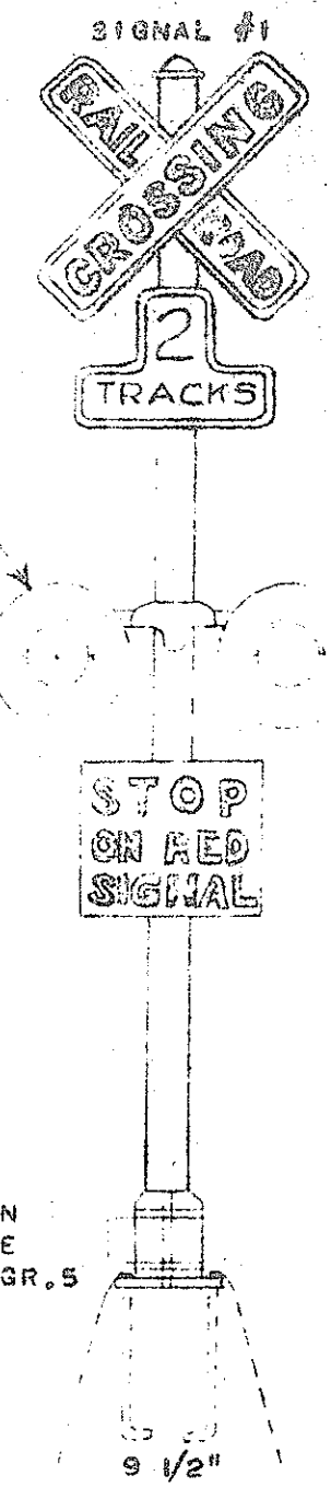
X ARM WITH 2 TYPE XB UNITS PL.H2925 FIG.E
