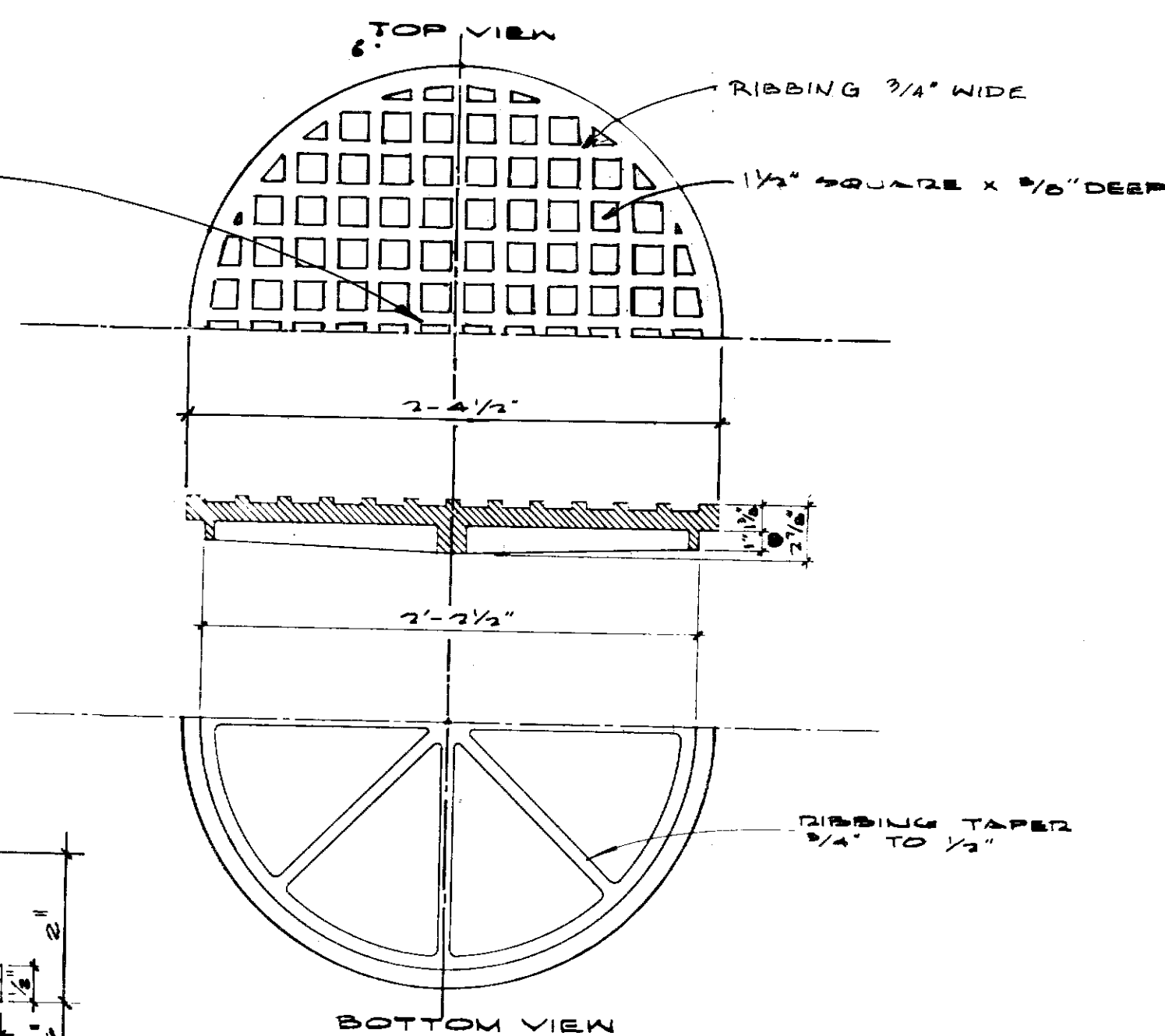
MANHOLE COVER FOR TYPE "B" AND "SB" FRAME
