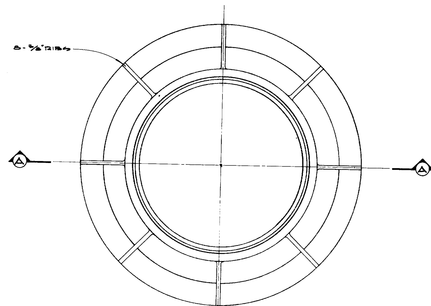
TOP VIEW MANHOLE FRAME TYPE "B" AND "SB"
