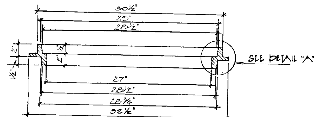
ADAPTOR RING 2" RISER ADAPTOR RING FOR EXISTING 27" DIA. FRAME
