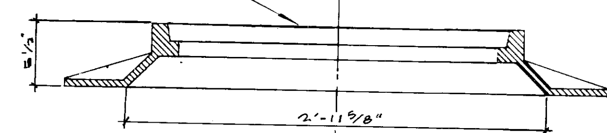
SECTION A-A TYPE "SB" MANHOLE FRAME
