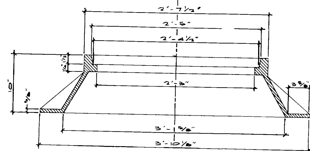
SECTION A-A TYPE "B" MANHOLE FRAME
