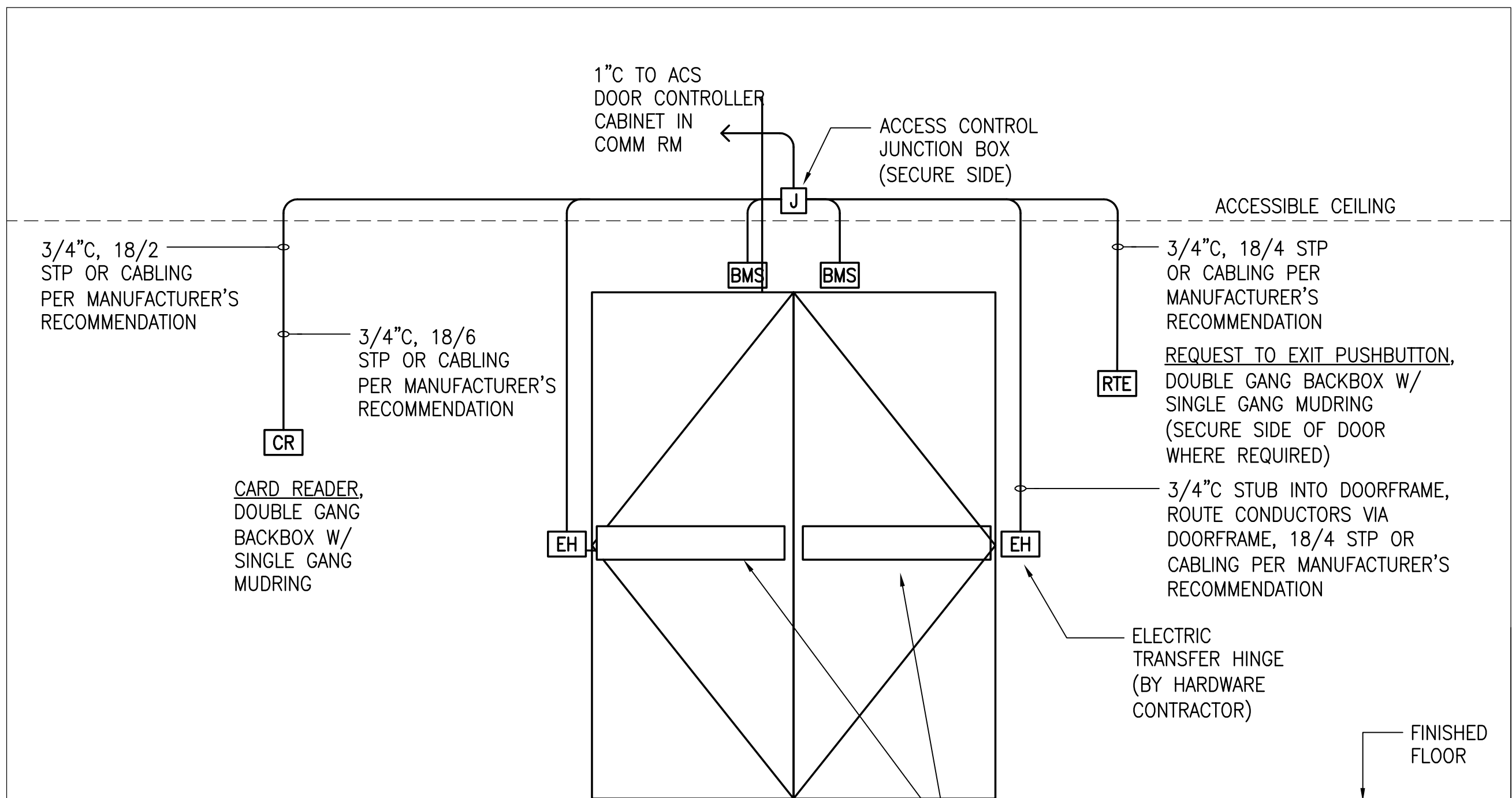
3 ACS DOOR CONNECTION DIAGRAM - DOUBLE DOOR W/ PANIC HARDWARE TC602 NO SCALE
