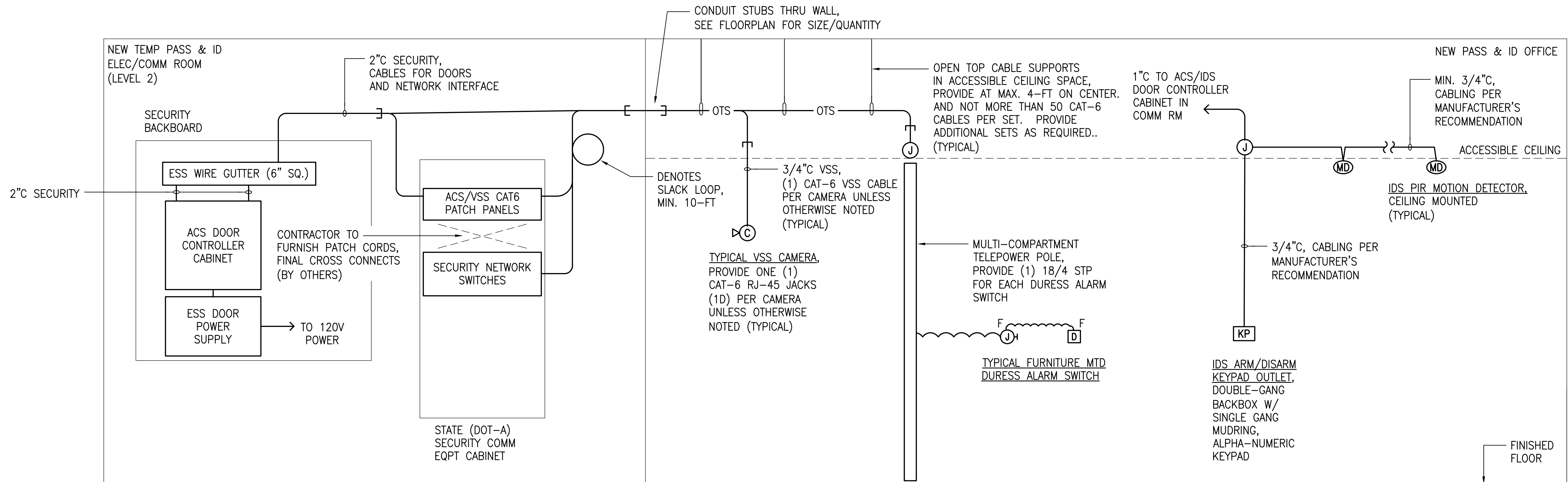
1 TELECOMMUNICATIONS RISER DIAGRAM - STATE (DOT-A) SECURITY ESS DISTRIBUTION TC602 NO SCALE
