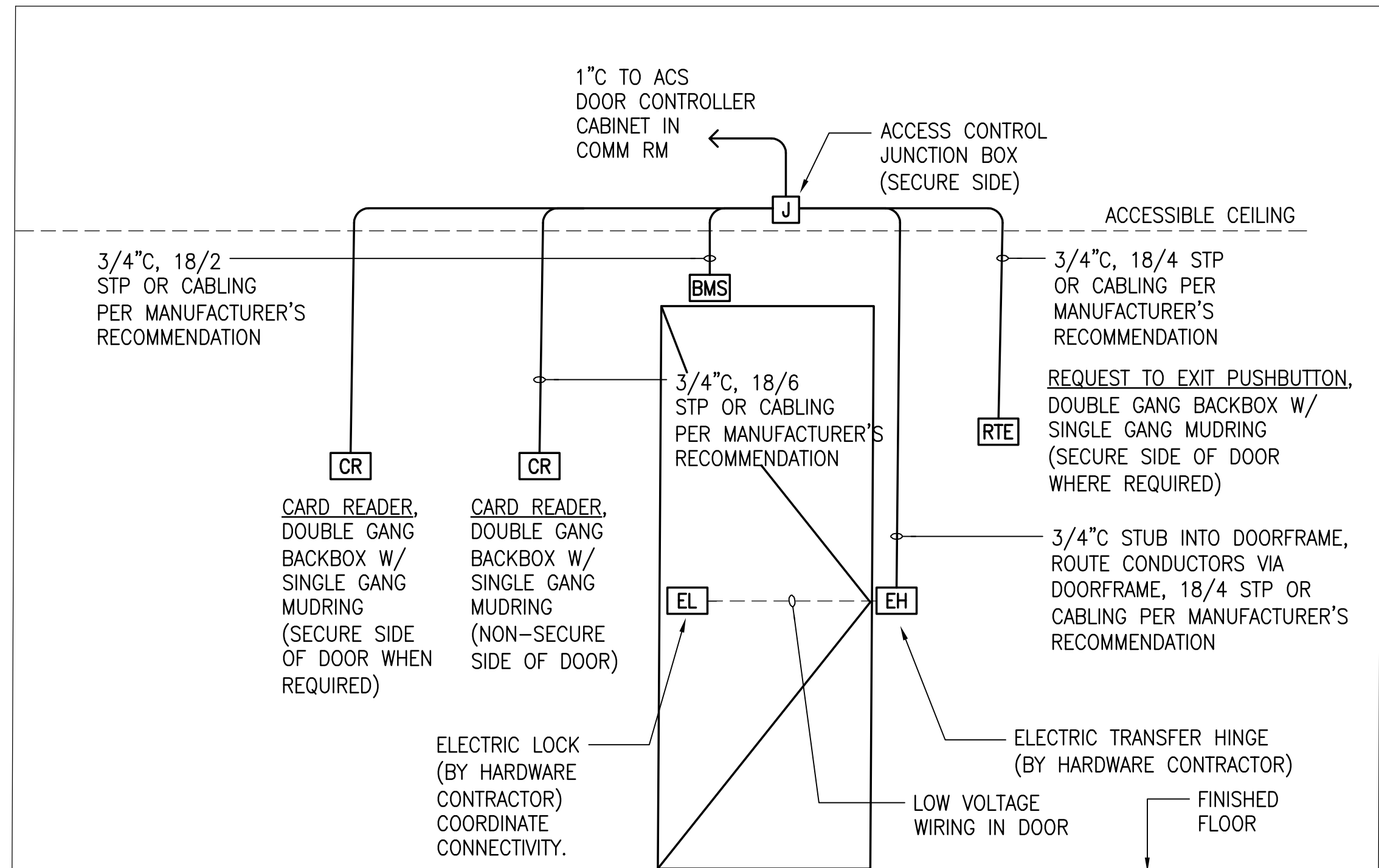
2 ACS DOOR CONNECTION DIAGRAM - SINGLE DOOR W/ ELECTRIC LOCKSET TC602 NO SCALE
