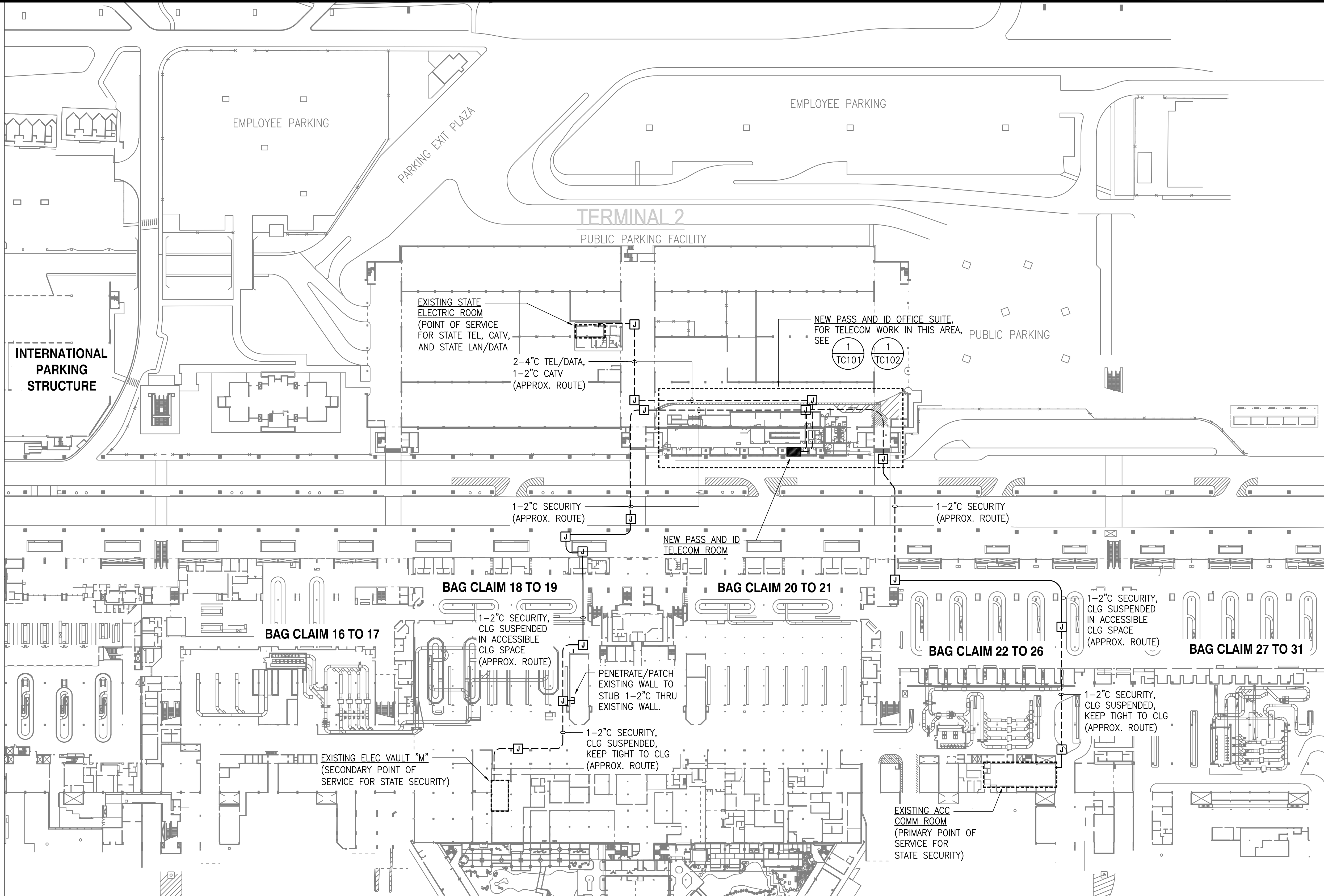
1 OVERALL TELECOM DISTRIBUTION PLAN SCALE: 1/64" = 1'-0"
