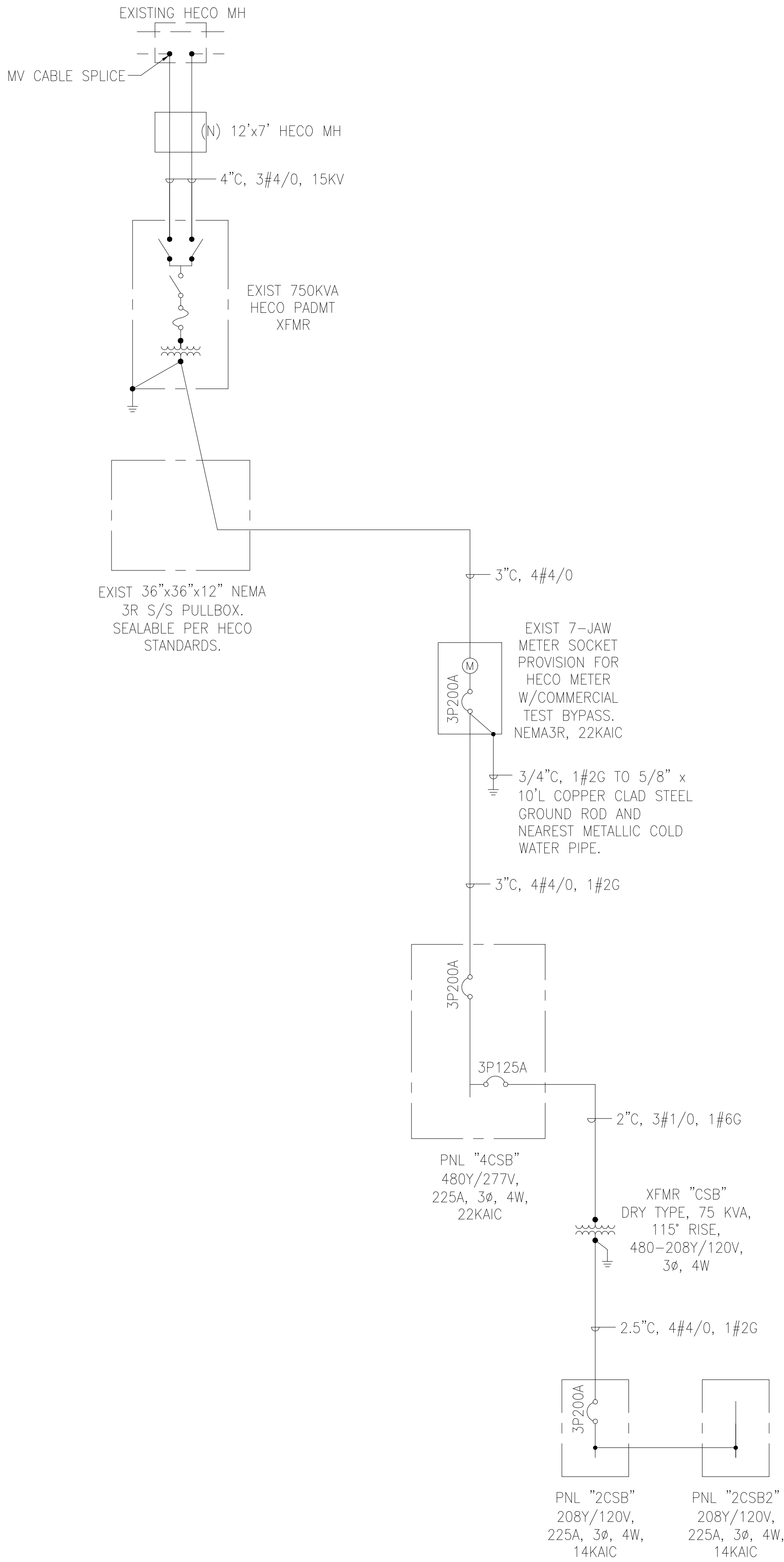
1 E-401 ELECTRICAL ONE-LINE DIAGRAM
