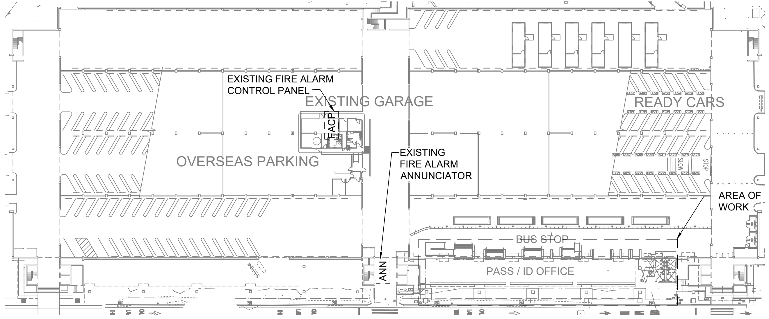
2 FA101 OVERALL GARAGE FIRE ALARM PLAN SCALE: 1" = 50'
