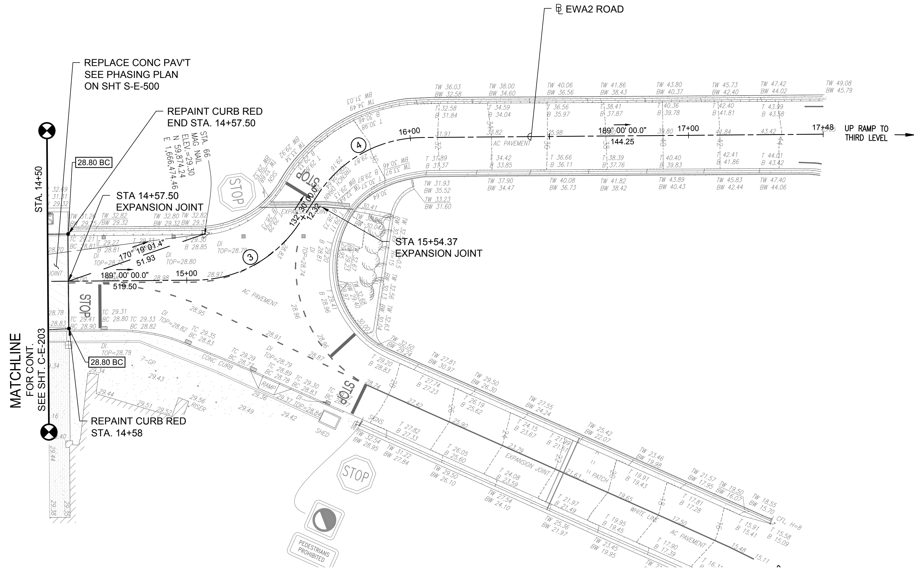
EWA WING LEVEL 2 - PLAN
