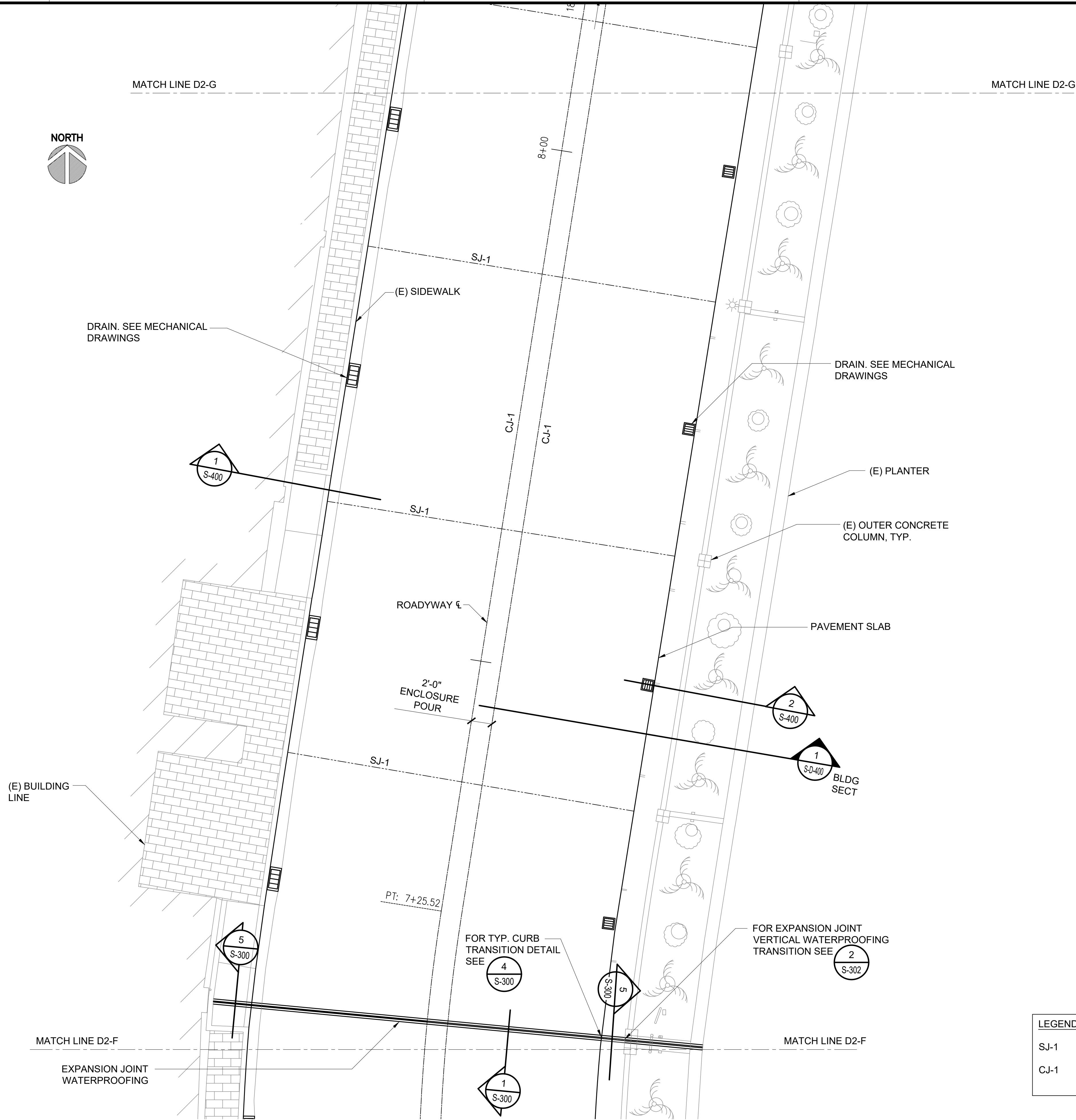
1 S-D-218 ENLARGED DH LEVEL 2 REPAIR PLAN G SCALE: 3/16" = 1'-0"
