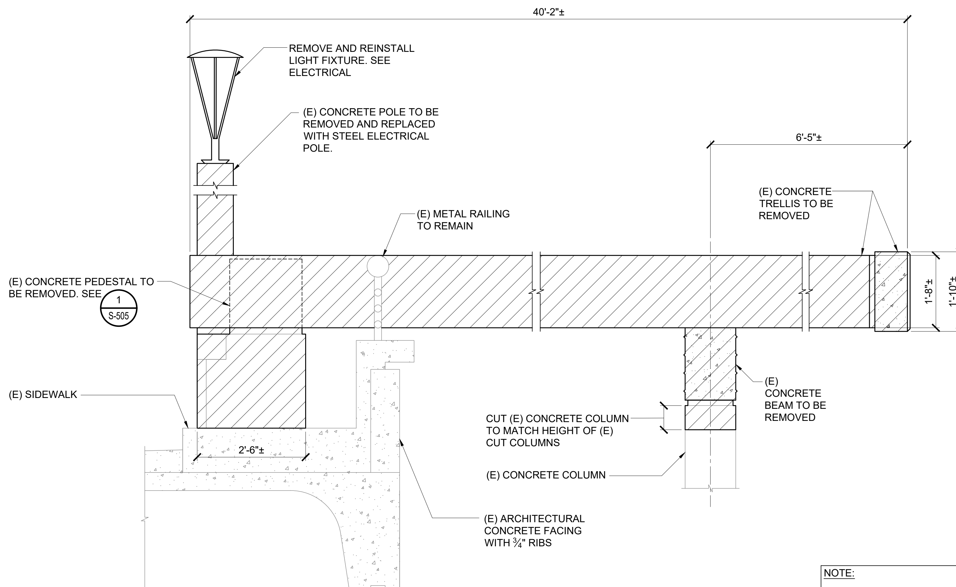
2 S-503 DIAMOND HEAD WING TRELLIS DEMOLITION ELEVATION SCALE: 3/4" = 1'-0"
