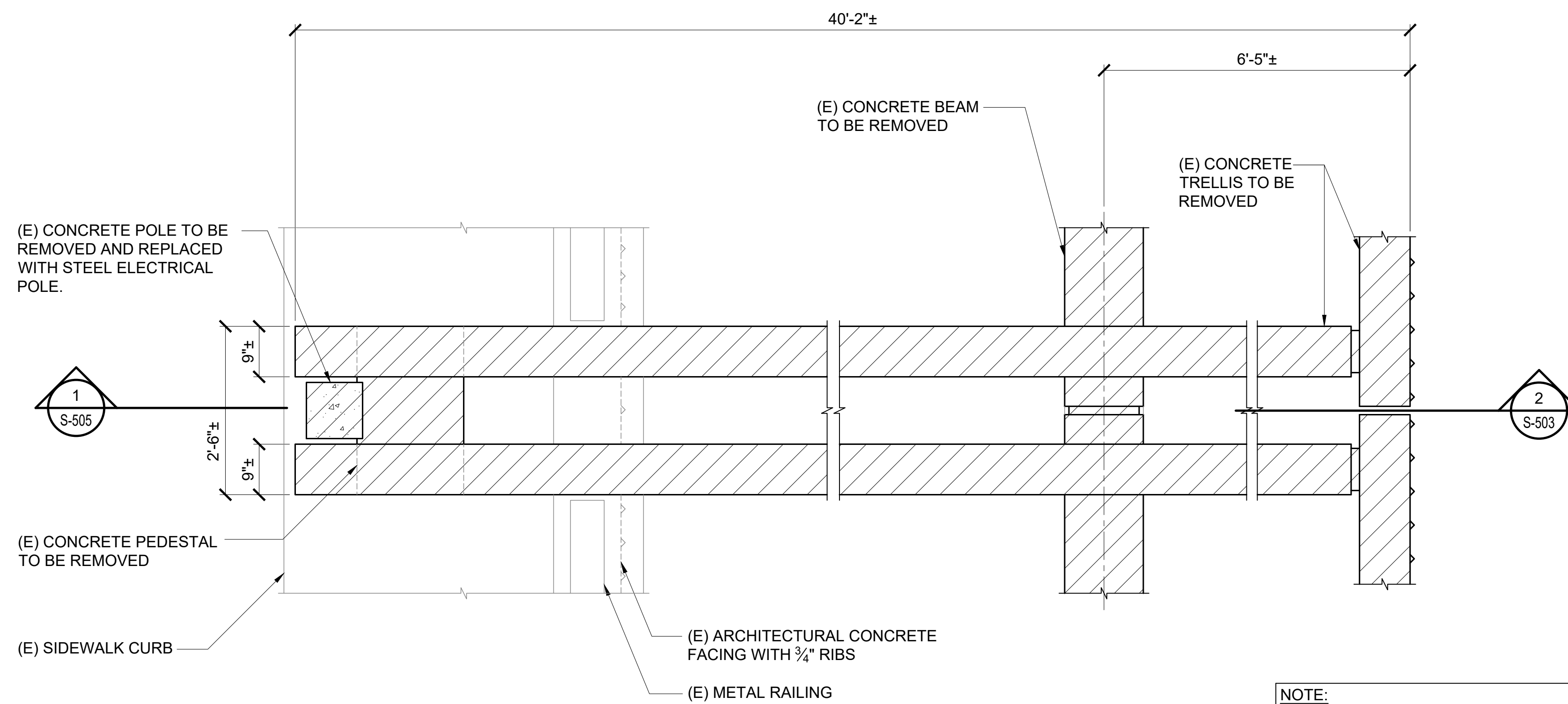
1 S-503 DIAMOND HEAD WING TRELLIS DEMOLITION PLAN SCALE: 3/4" = 1'-0"
