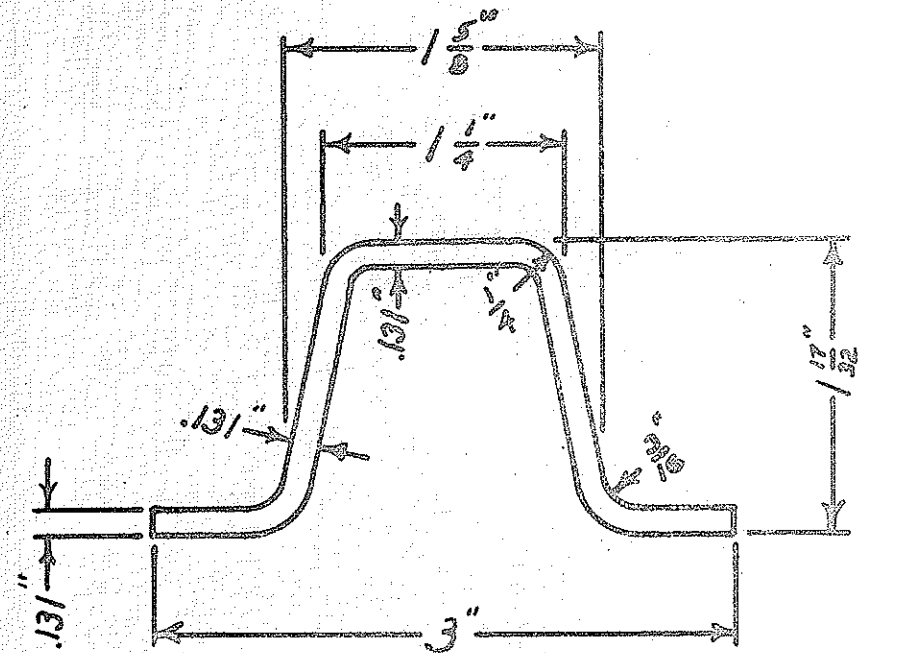
FULL SIZE SECTION OF POST
