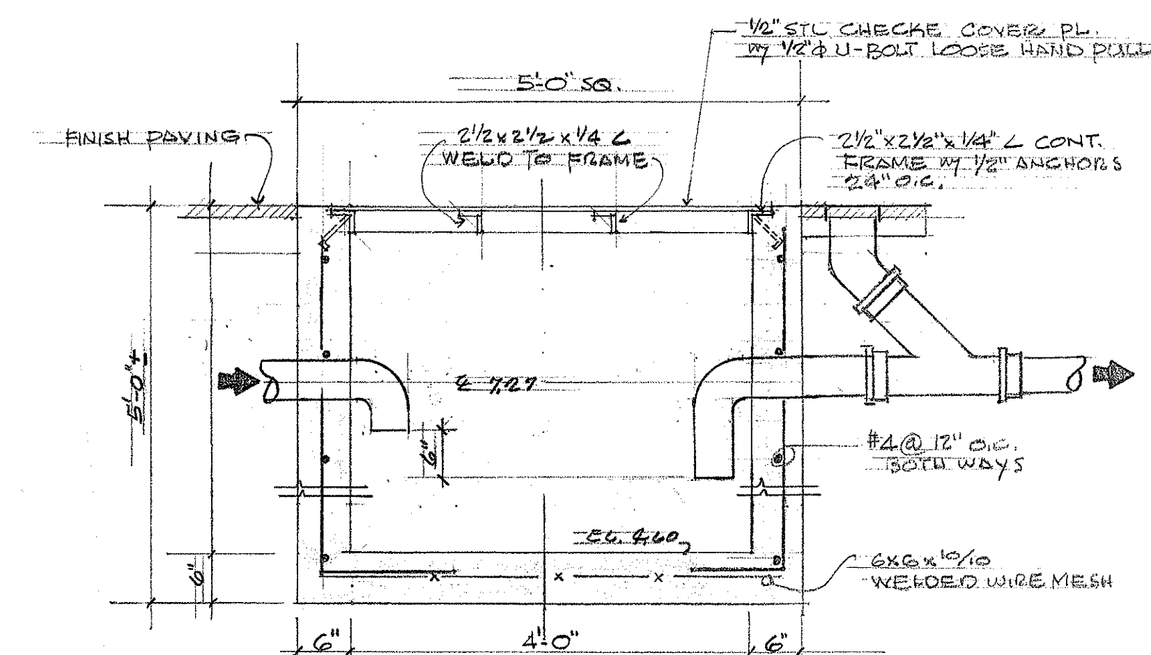
\frac{A}{P.3} SAND & GREASE TRAP DET. SC. 3/4" = 1'-0"
