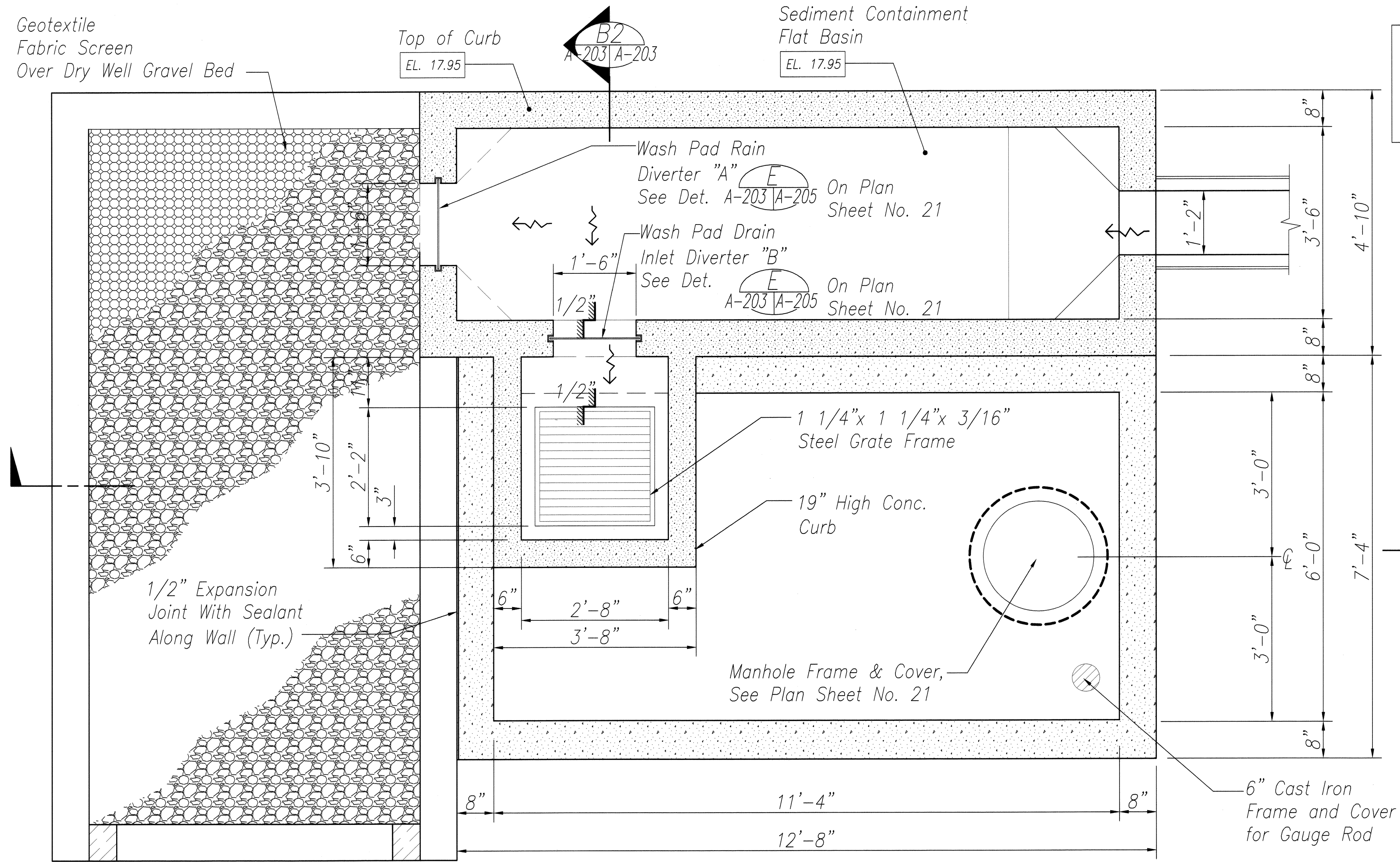
A1 SEDIMENT CONTAINMENT BASIN AND WASH DOWN WATER HOLDING TANK PLAN A-203/A-203 3/4" = 1'-0"
