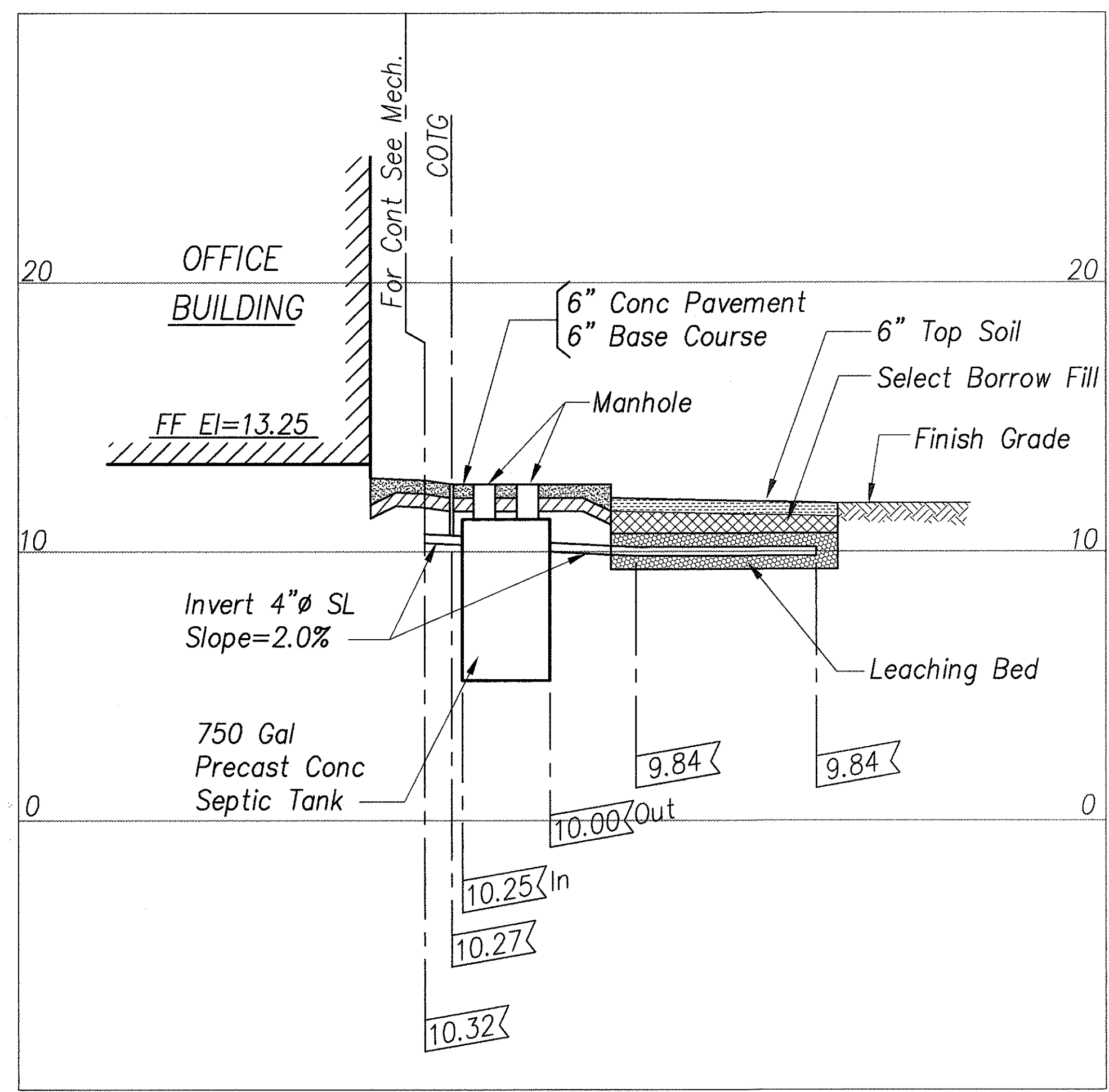
SEWER SYSTEM PROFILE SCALES: HORIZ 1"=10' VERT 1"=4'
