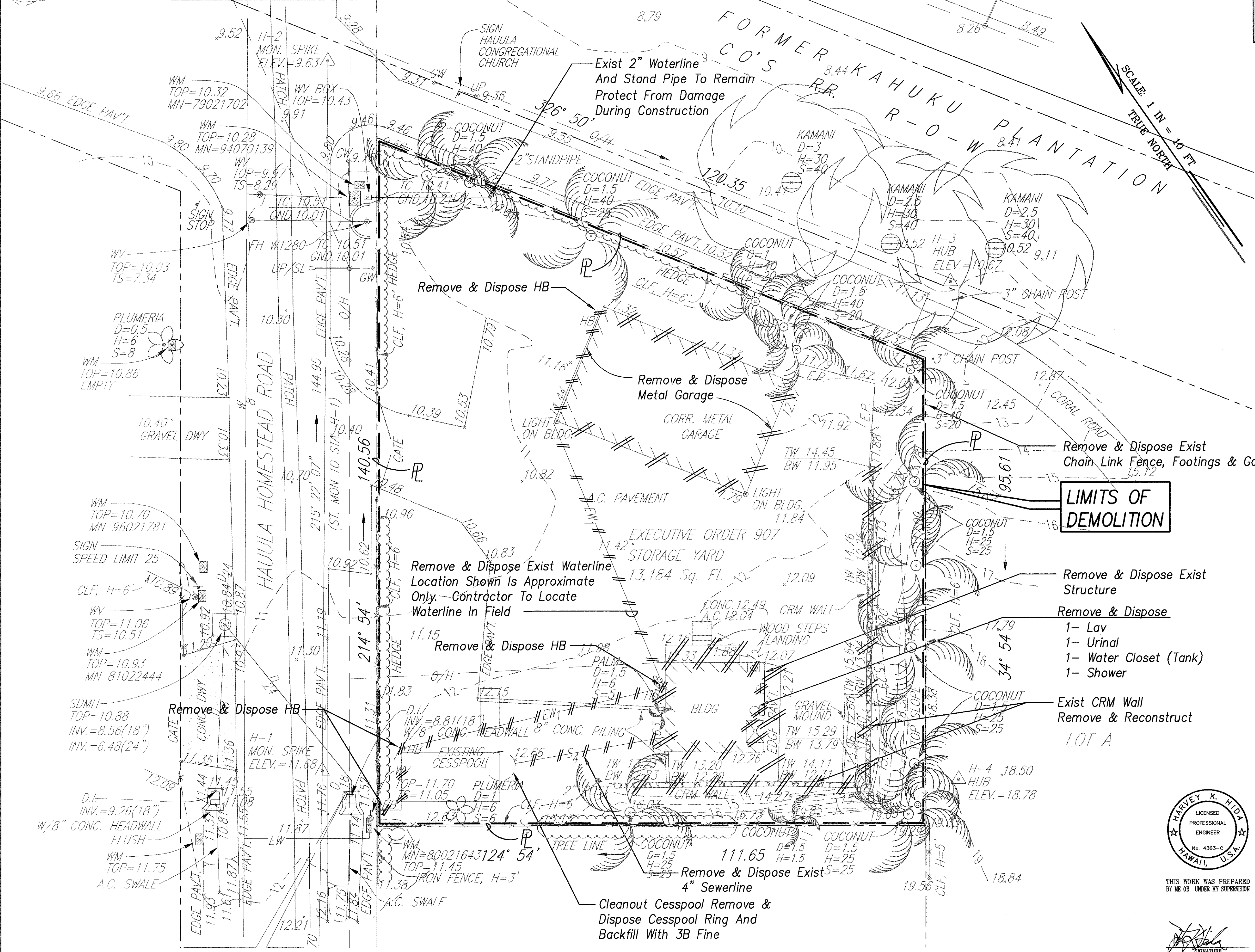
DEMOLITION PLAN SCALE: 1" = 10'
