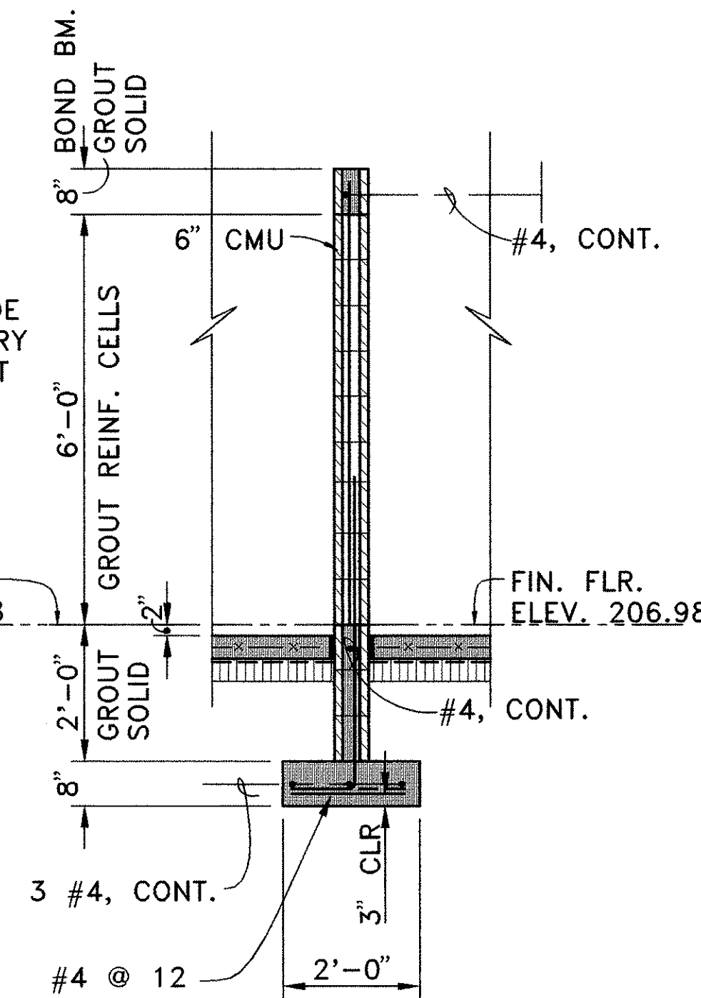
6" CMU WALL AT LOCKERS
