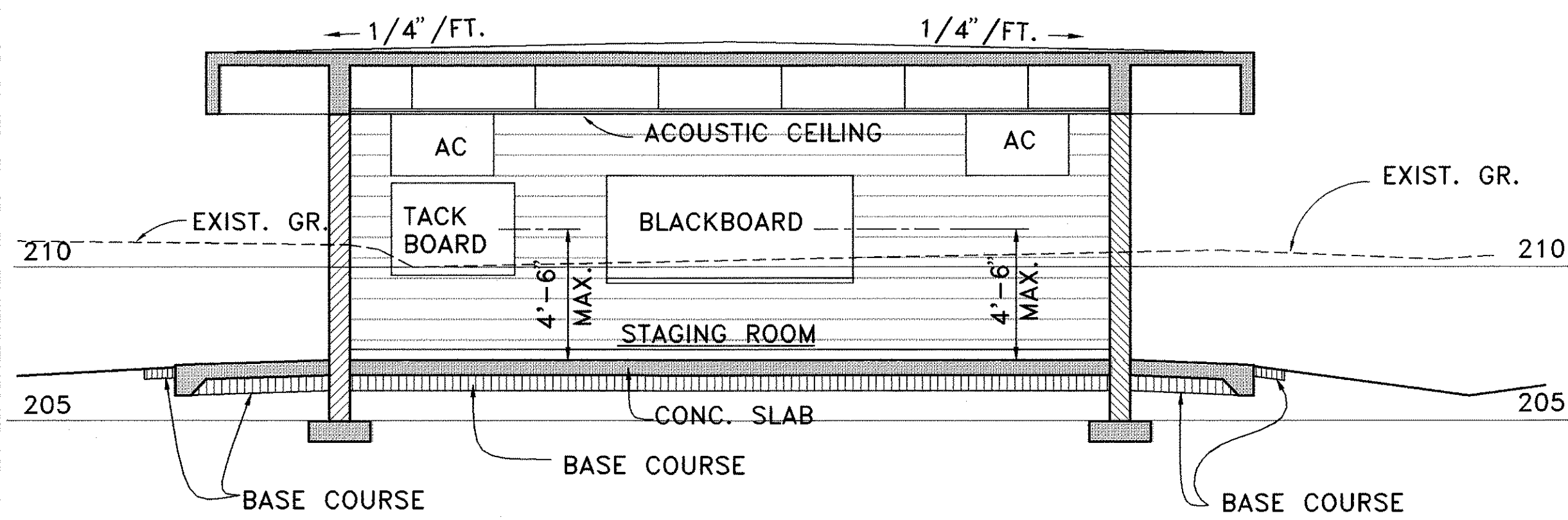
TRANSVERSE SECTION THROUGH ADMINISTRATION BUILDING A SCALE: 1/4" = 1' 0"
