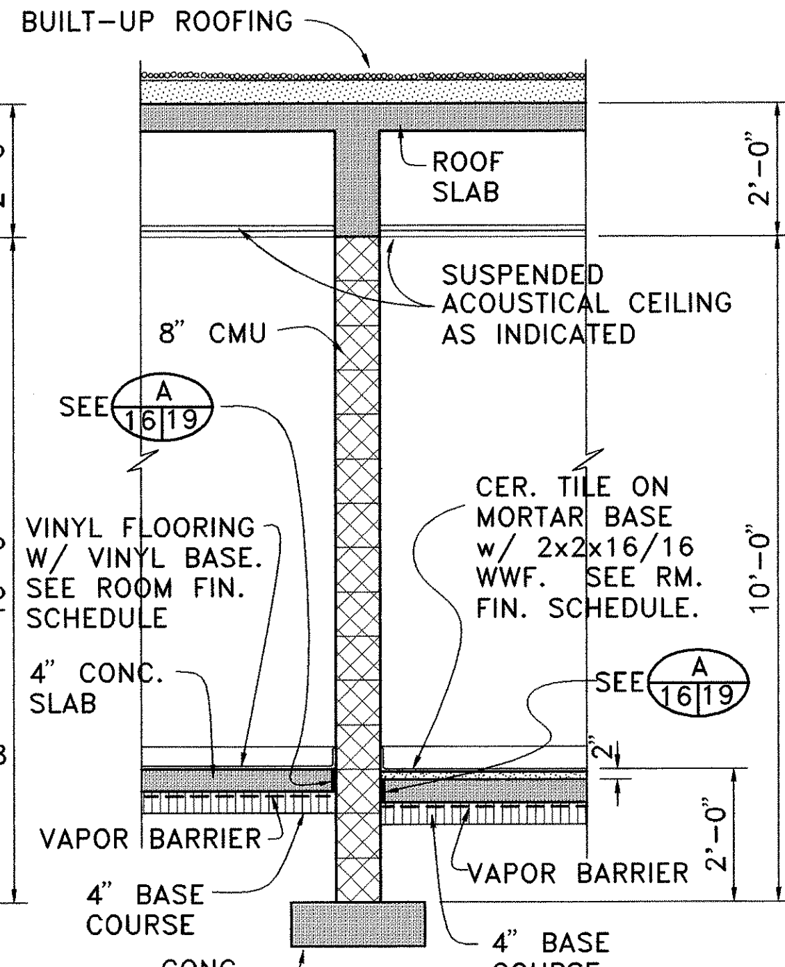
TYPICAL INTERIOR WALL
