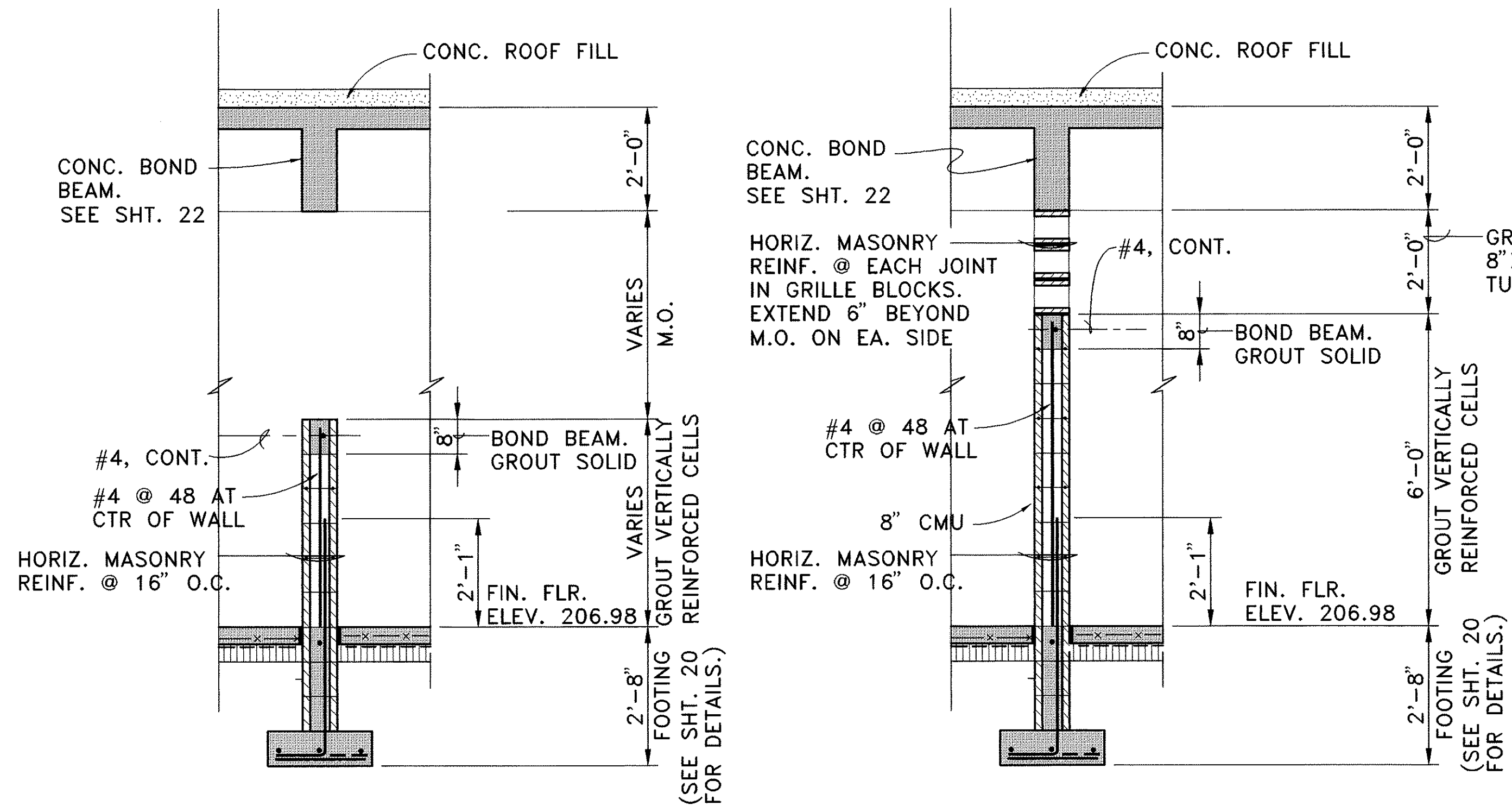
AT WINDOWS & OTHER MASONRY OPENINGS (M.O.)
