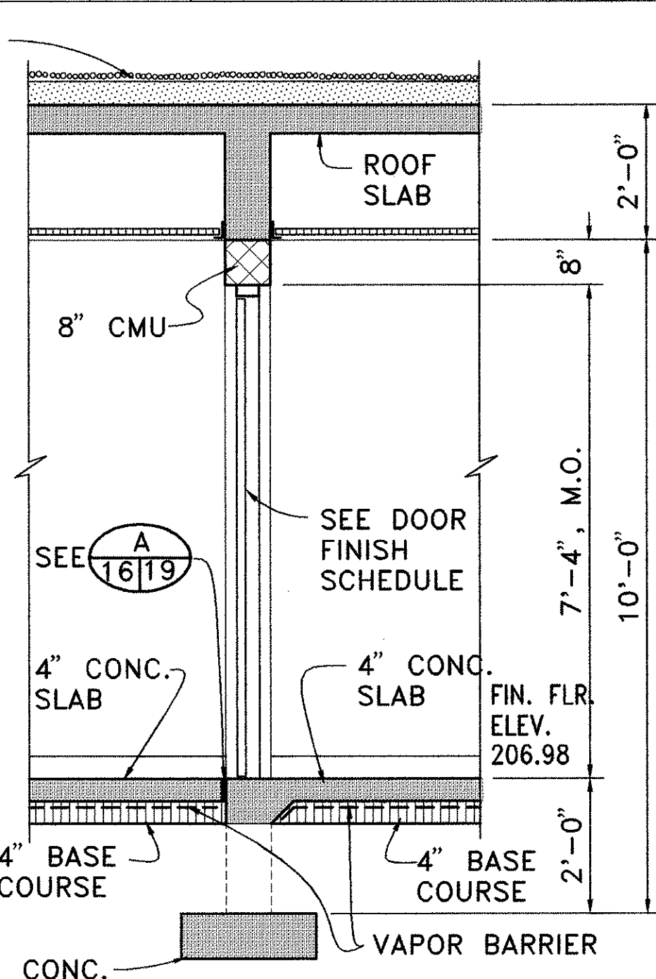
AT INTERIOR DOOR OPENING
