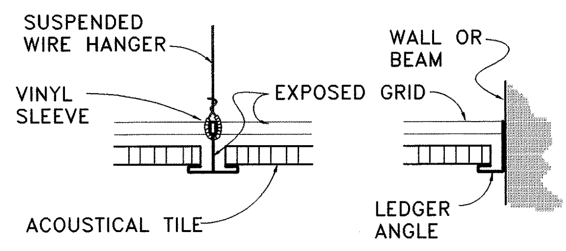
AT HANGERS AT WALLS
