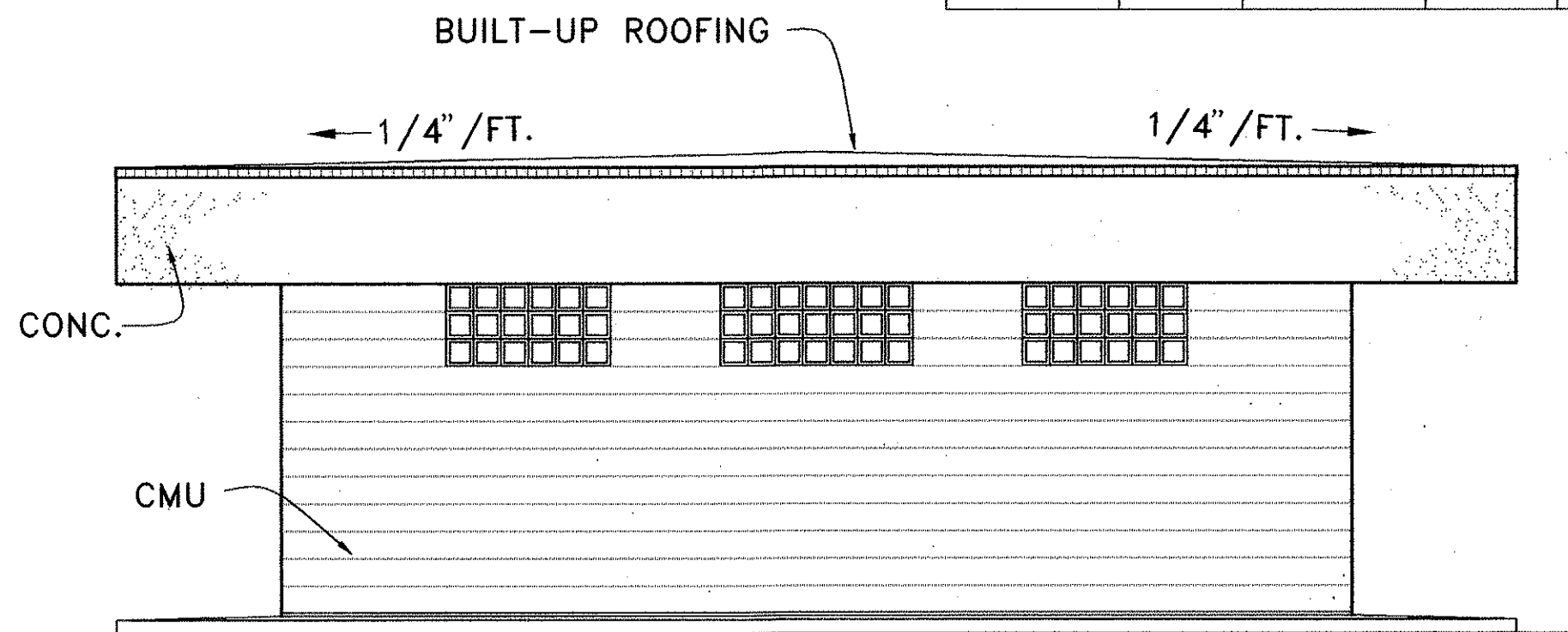
SOUTH ELEVATION
