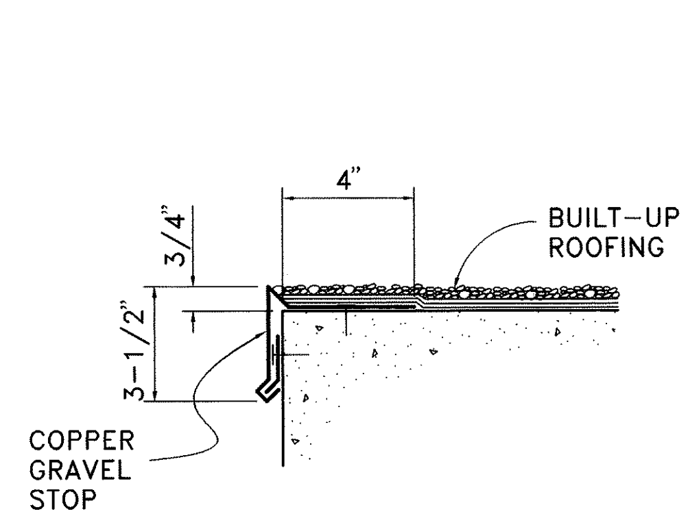
EAVE FLASHING DETAIL A 1818 NOT TO SCALE
