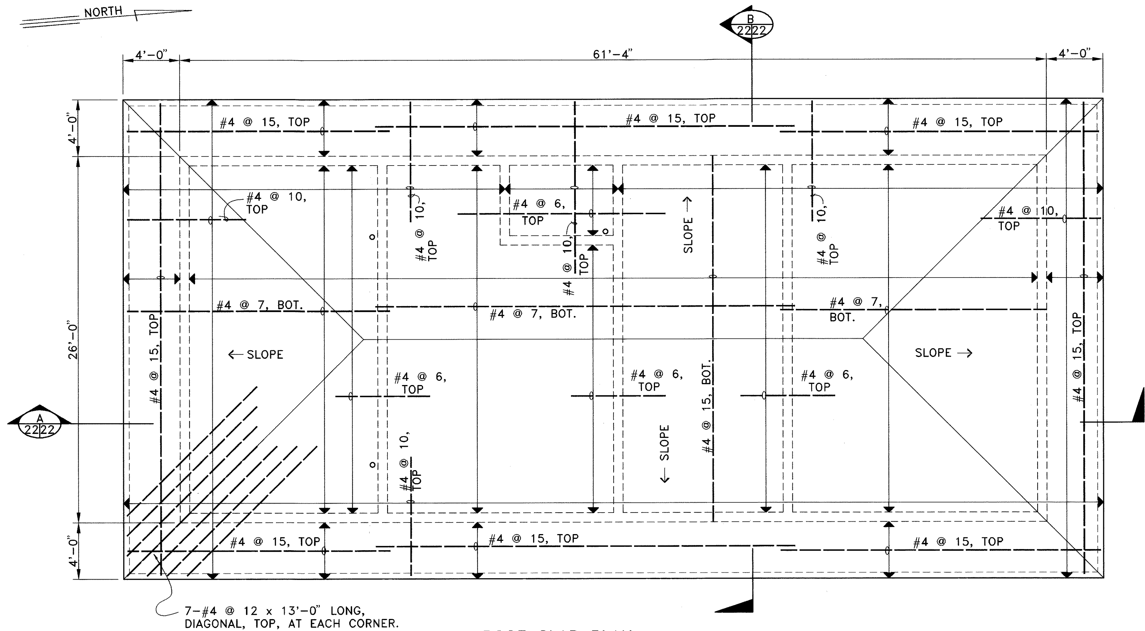
ROOF SLAB PLAN SCALE: 1/4" = 1' 0"
