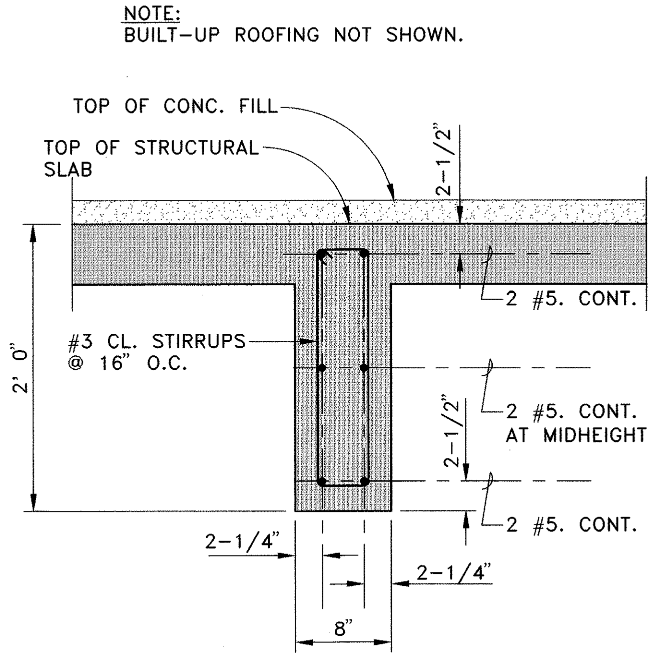
TYPICAL BOND BEAM DETAIL SCALE: 1-1/2" = 1' 0"
