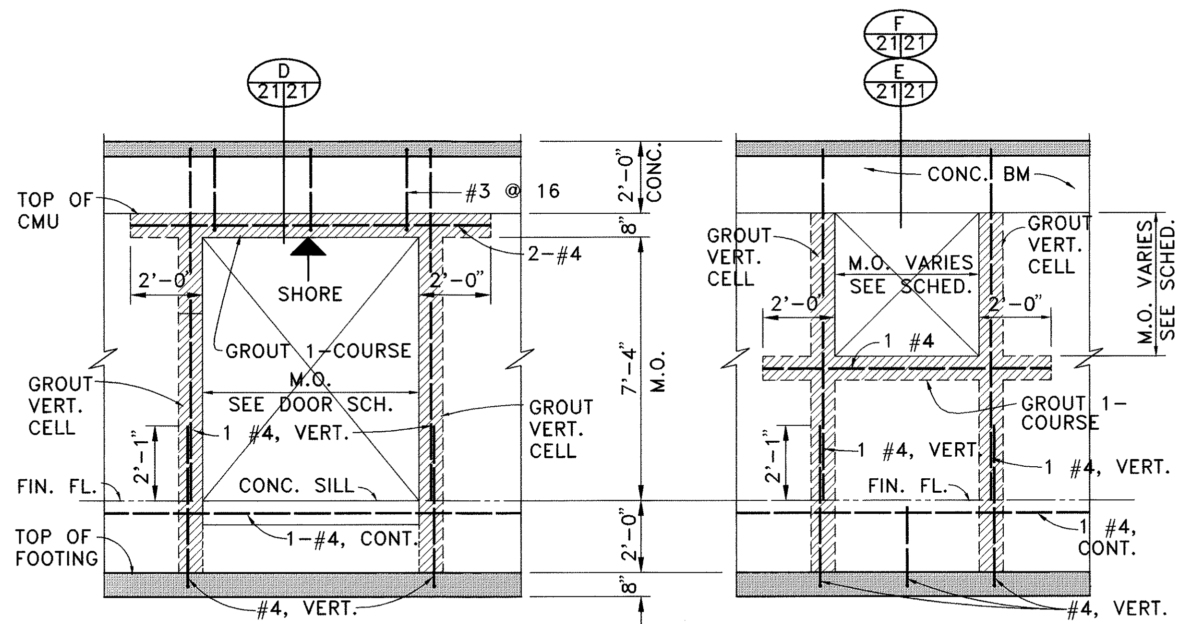
TYPICAL WINDOW OPENING (OPENING FOR A.C. UNIT & GRILL BLOCKS SIMILAR)
