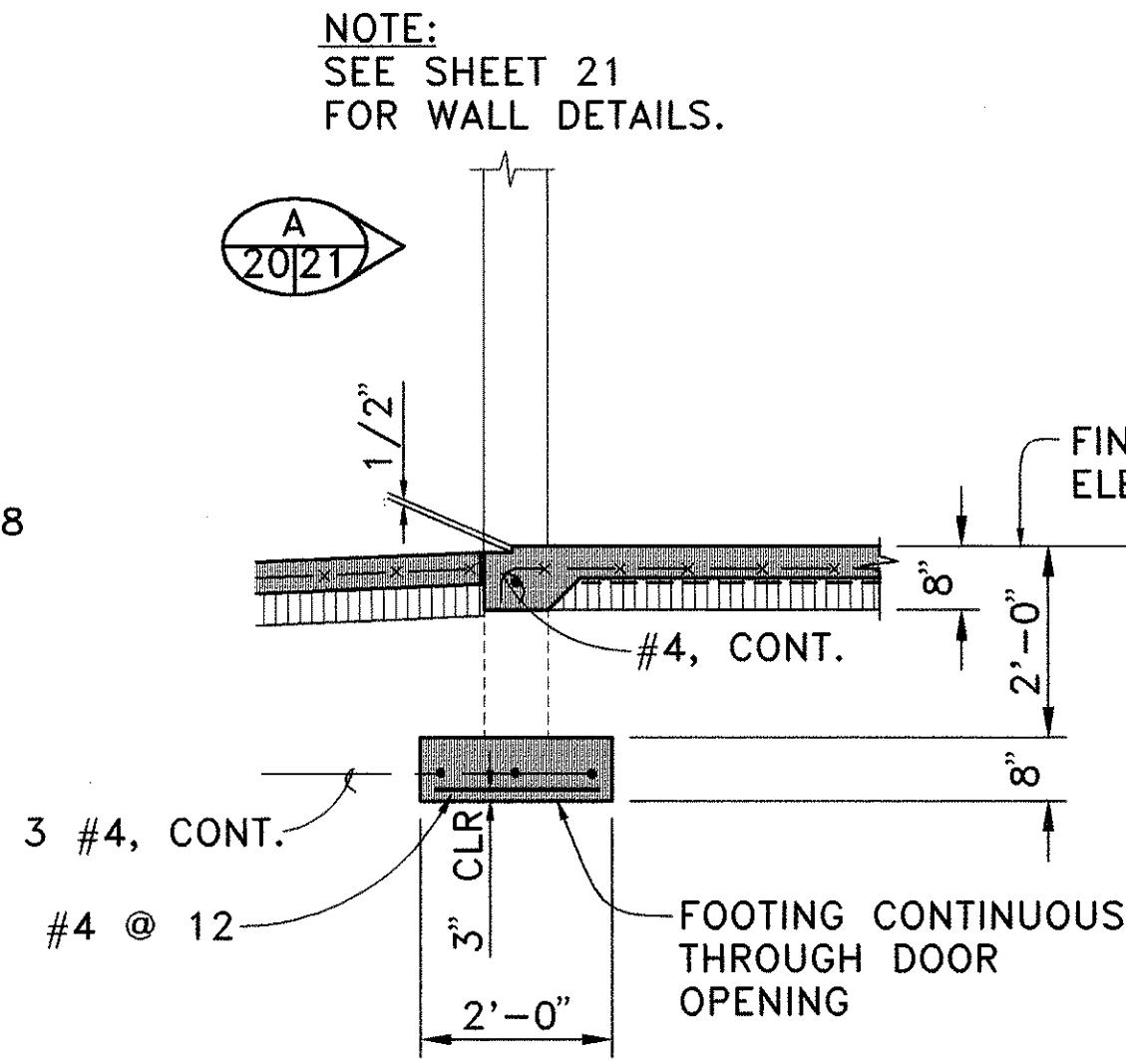
AT EXTERIOR DOOR OPENING
