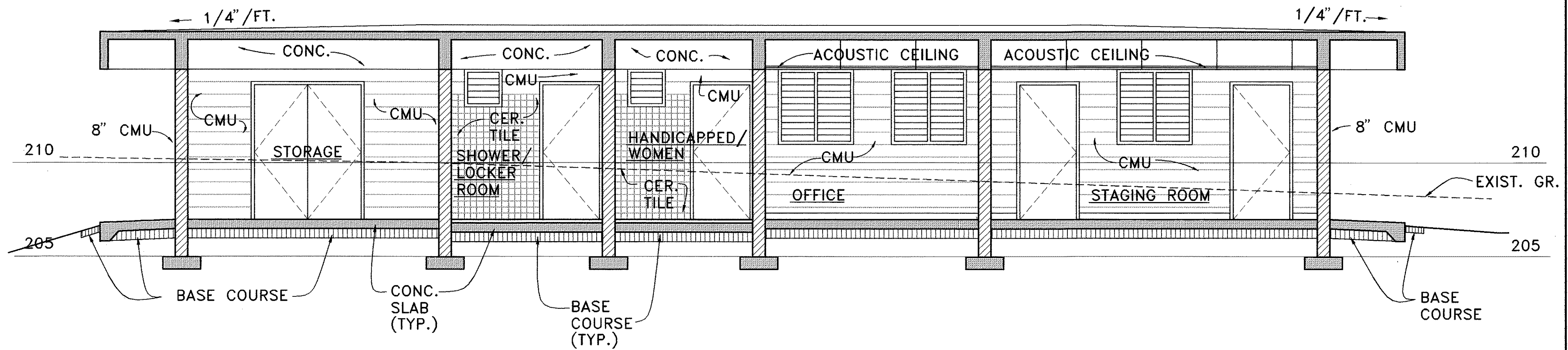
LONGITUDINAL SECTION THROUGH ADMINISTRATION BUILDING B SCALE: 1/4" = 1' 0"
