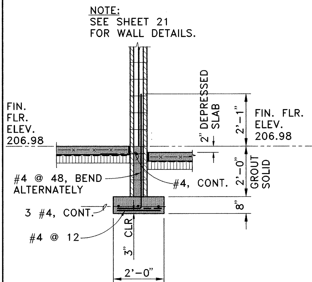
AT DEPRESSED SLAB
