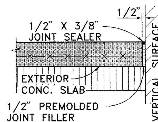
EXTERIOR SLAB EXPANSION JOINT SCALE: 1" = 1' 0"
