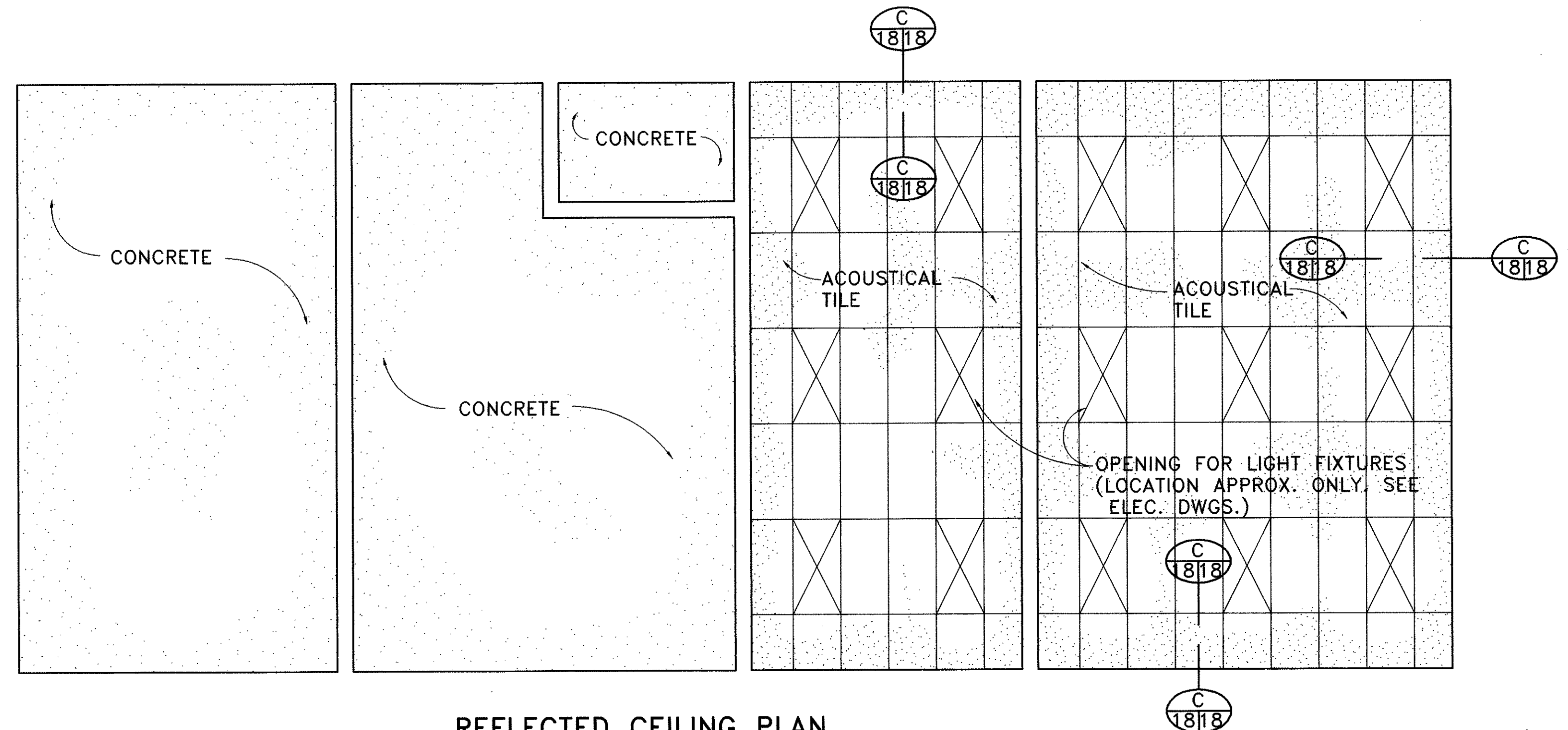
REFLECTED CEILING PLAN SCALE: 1/4" = 1' 0"
