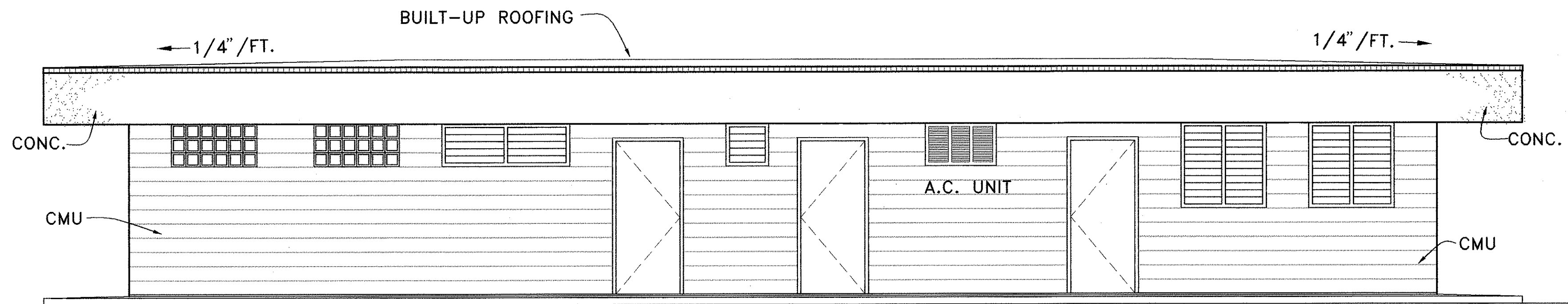
EAST ELEVATION
