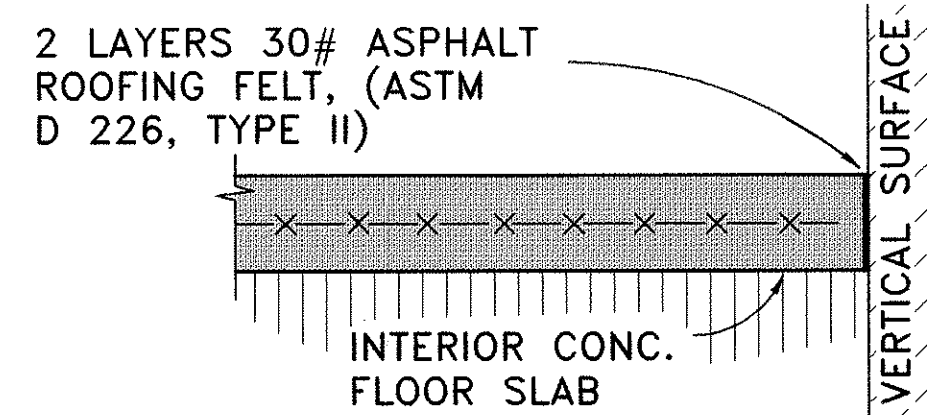
TYPICAL CONCRETE SLAB SCALE: 1" = 1' 0"
