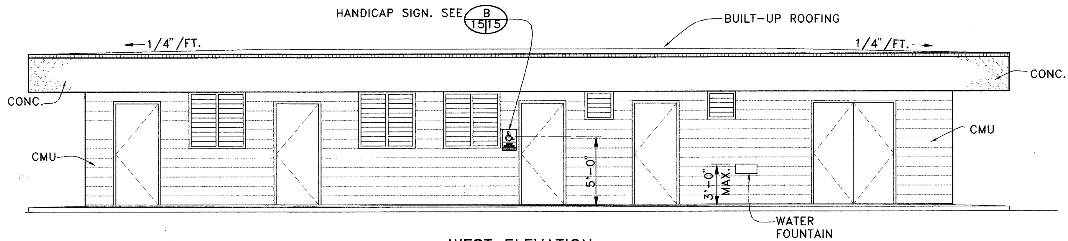
WEST ELEVATION
