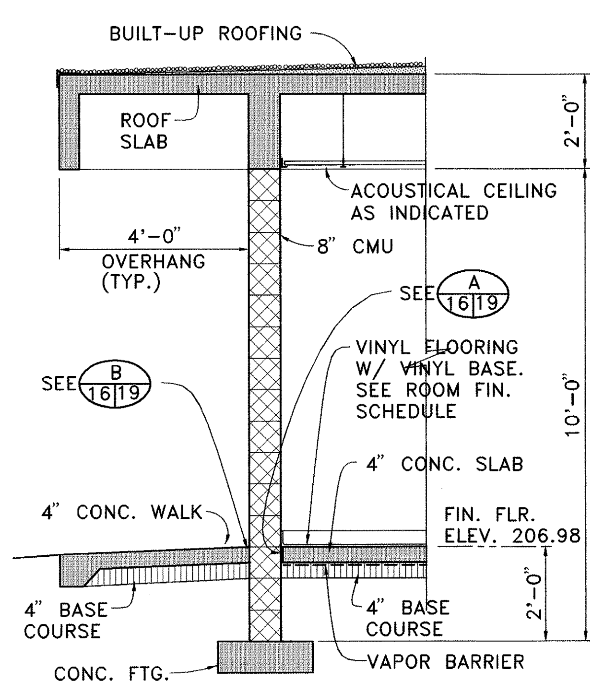
TYPICAL EXTERIOR WALL
