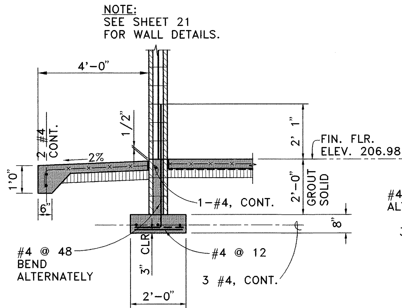
AT EXTERIOR WALL
