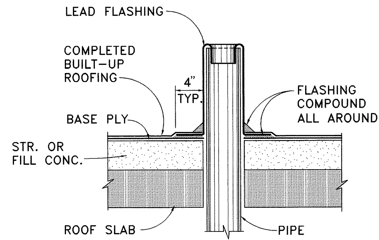
PIPE FLASHING DETAIL B 1818 NOT TO SCALE
