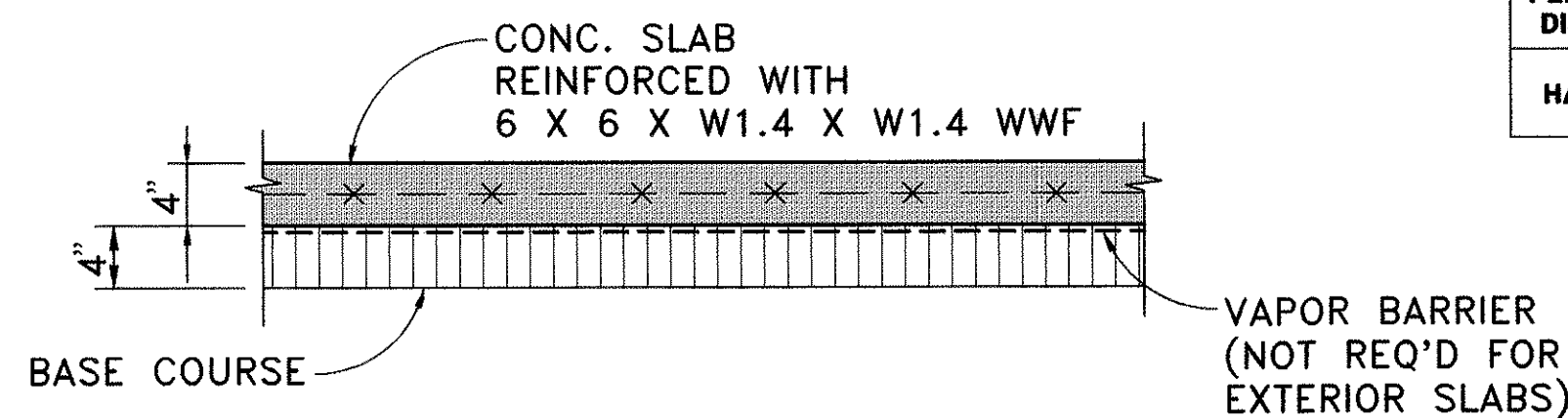
TYPICAL CONCRETE SLAB SCALE: 1" = 1' 0"
