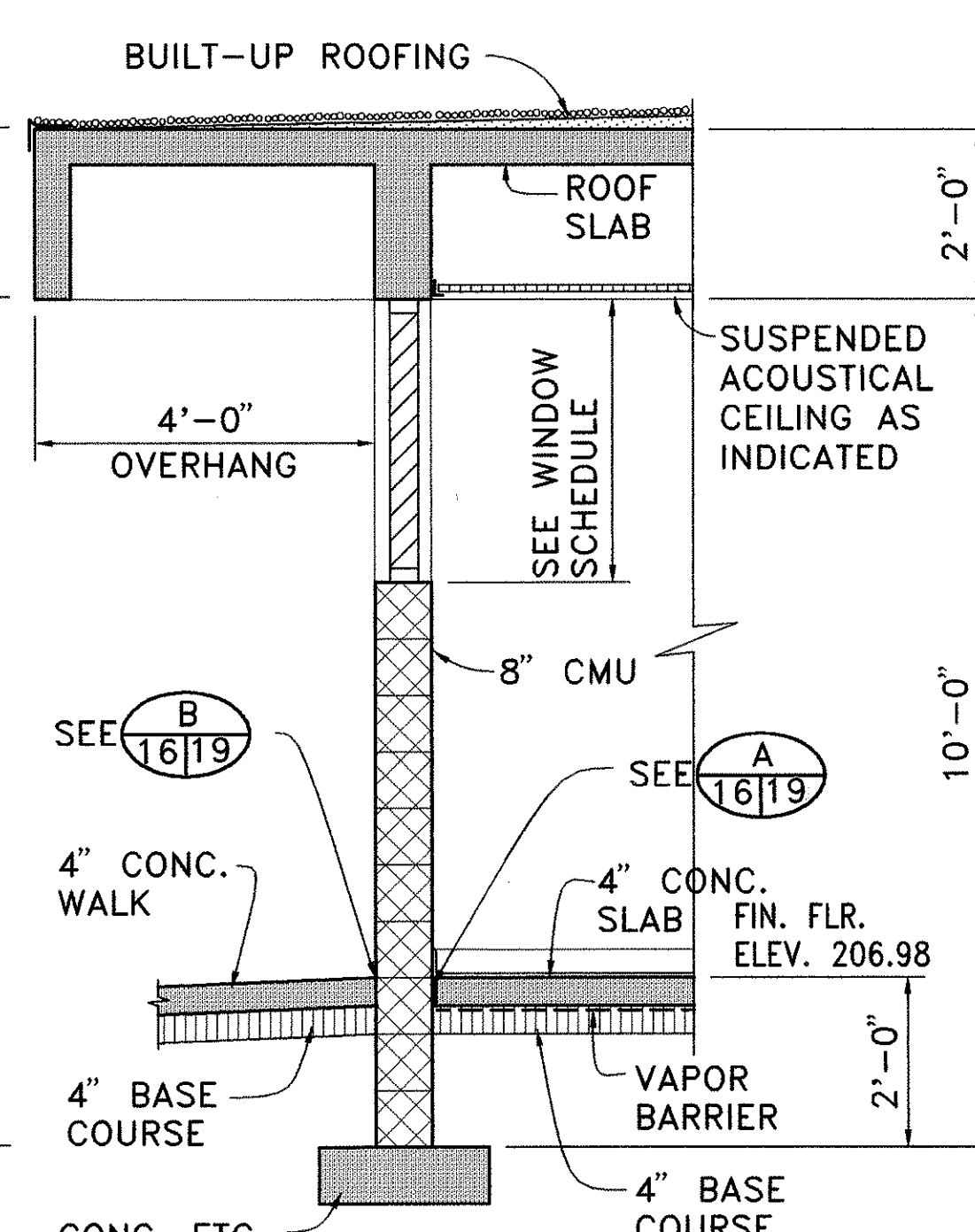
AT EXTERIOR WINDOW OPENING (OPENING FOR A.C. UNIT SIMILAR)
