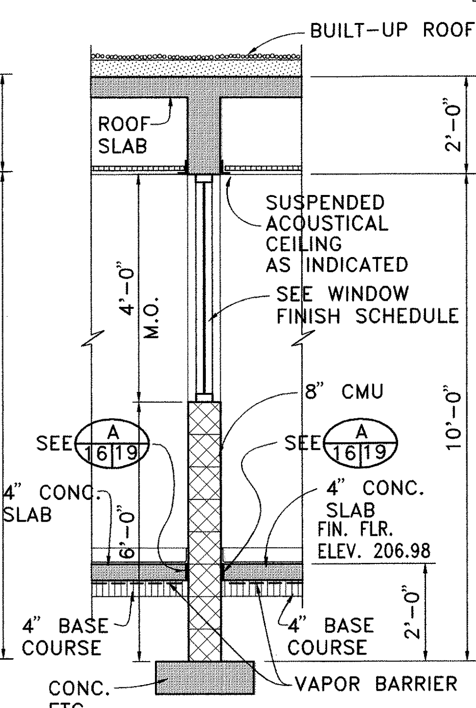
AT INTERIOR WINDOW OPENING
