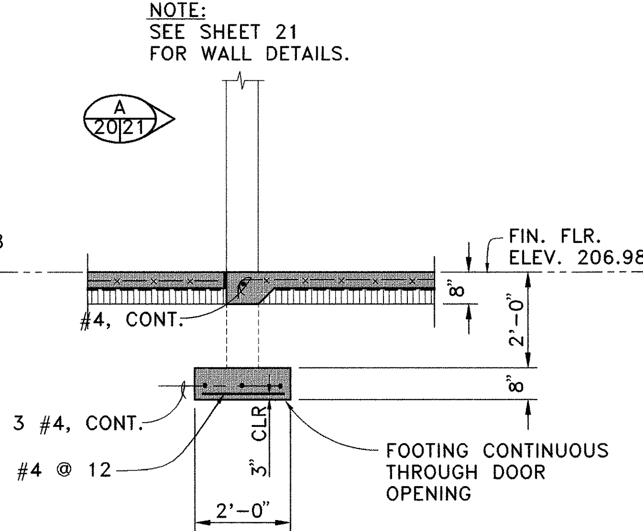
AT INTERIOR DOOR OPENING
