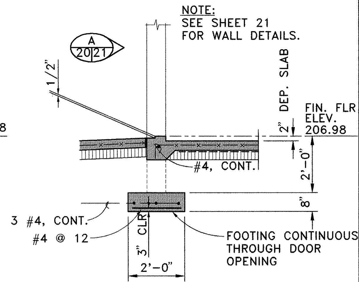
EXTERIOR DOOR OPENING AT DEPRESSED SLAB
