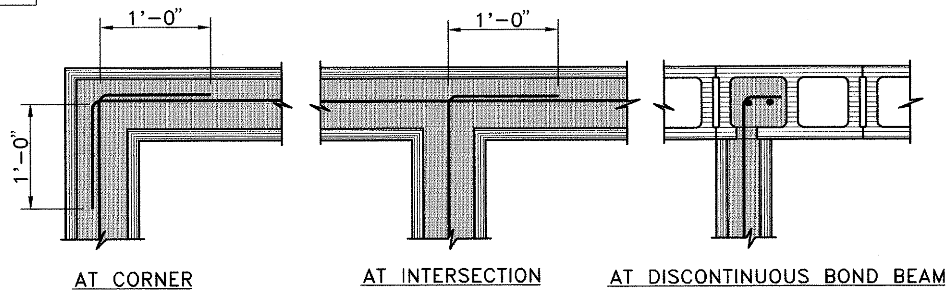
HORIZONTAL REINFORCING STEEL SPLICE NOT TO SCALE
