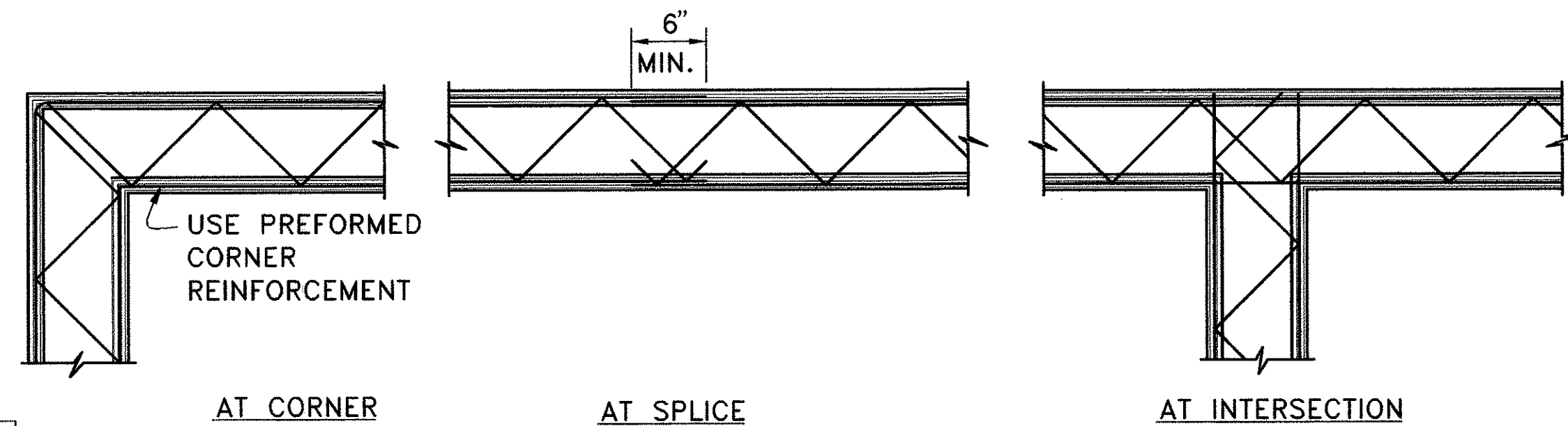
HORIZONTAL MASONRY JOINT REINFORCING DETAILS NOT TO SCALE
