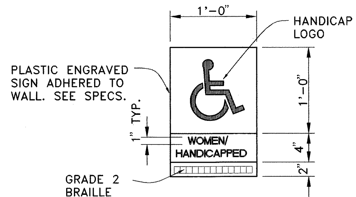
HANDICAP SIGN DETAIL
