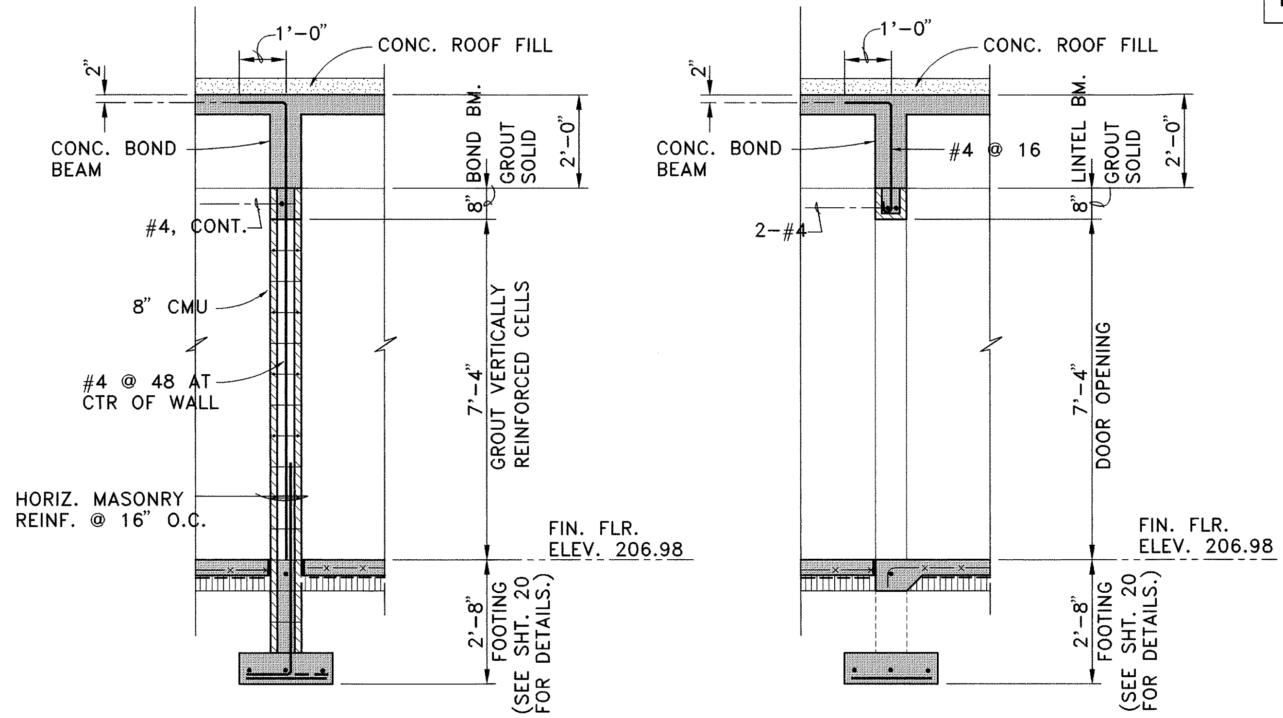
TYPICAL CMU WALL SECTION AT DOOR OPENINGS
