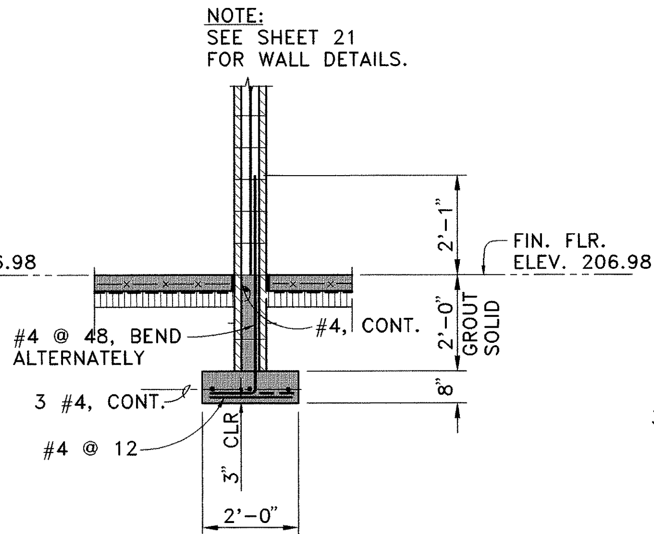
AT INTERIOR WALL
