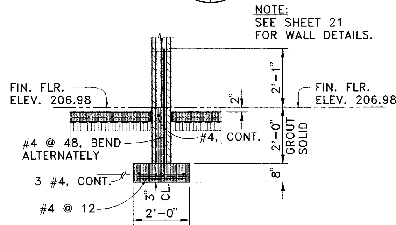
AT INTERIOR WALL
