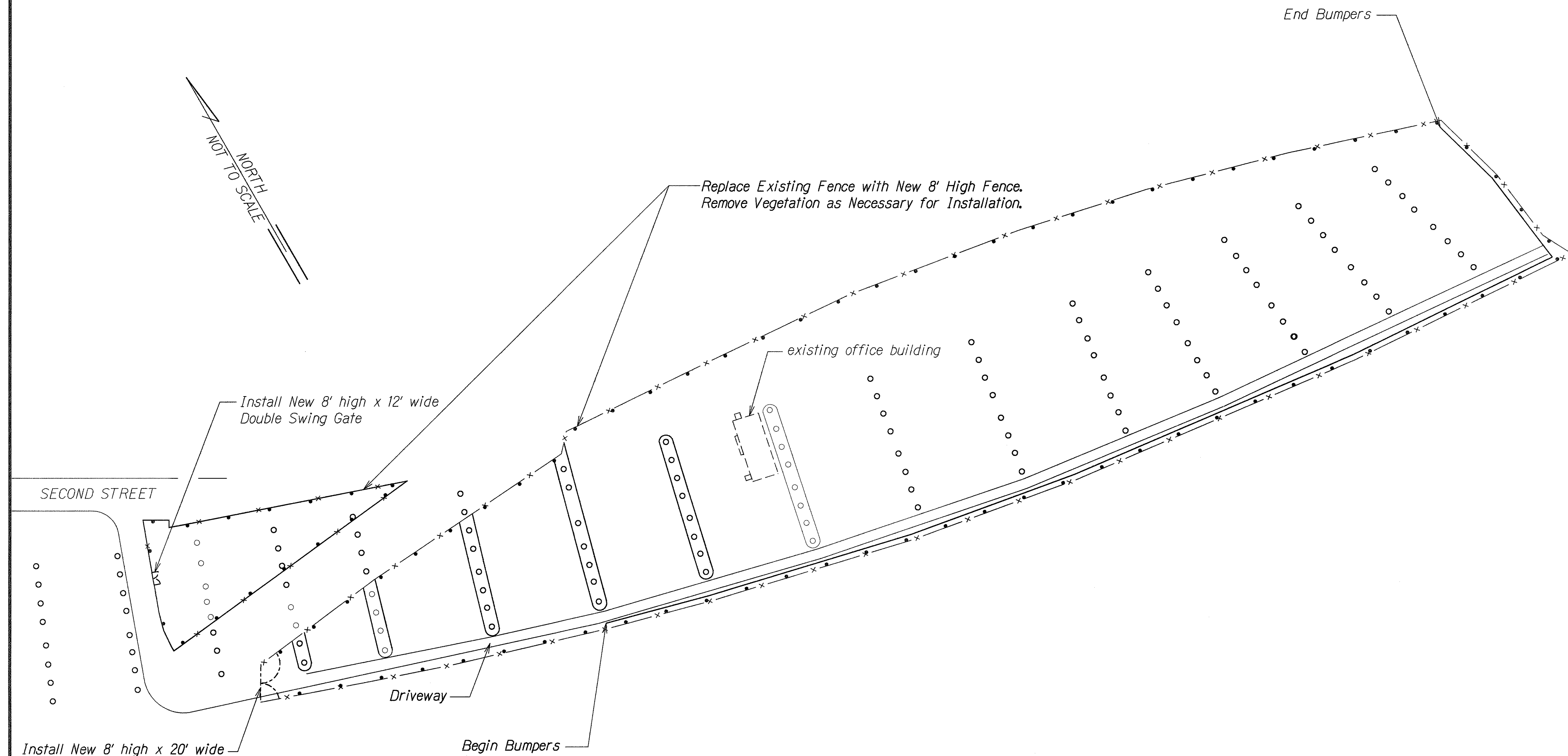
PEARL CITY BASE YARD PLAN Not to Scale
