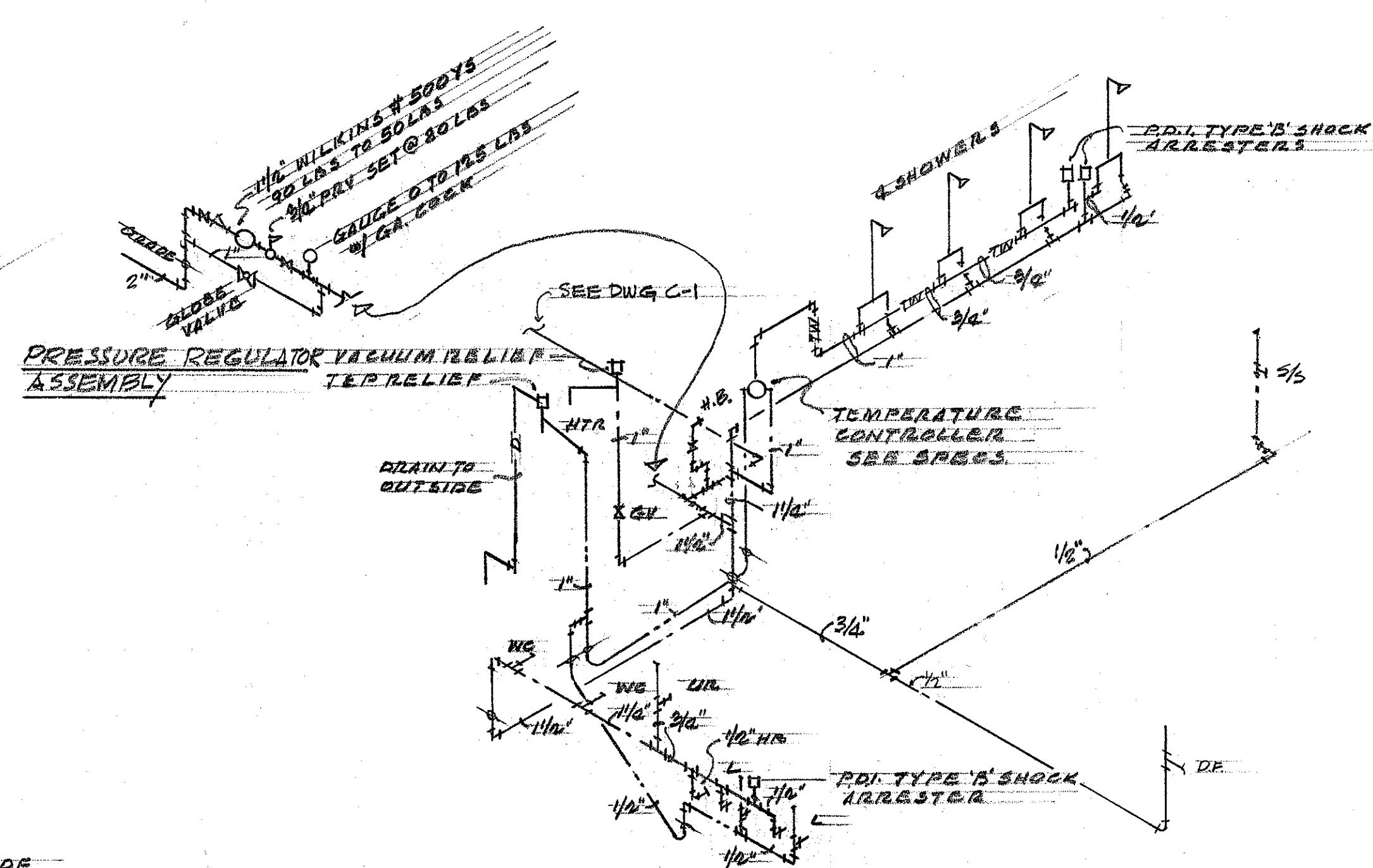
WATER DIAGRAM NO SCALE
