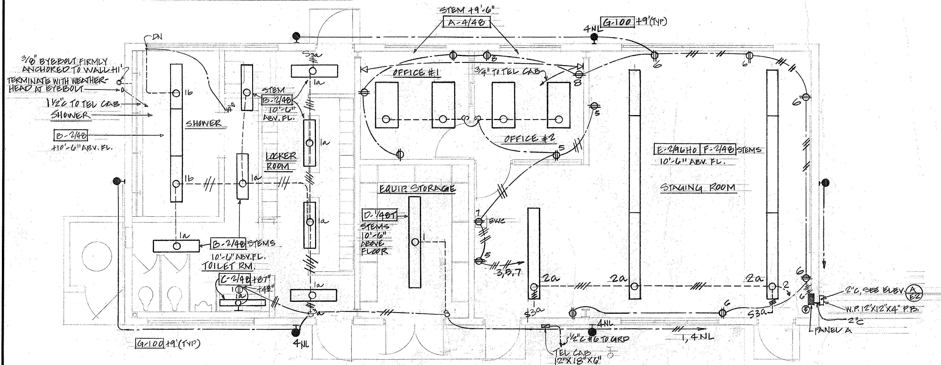
ELECTRICAL FLOOR PLAN
